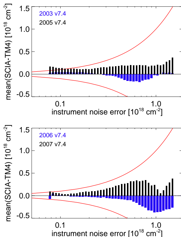
Fig. 4. Average differences between the single SCIAMACHY CO measurements and the spatially and temporally collocated TM4 CO total columns as function of the instrument-noise error for different years using the IMLM retrieval version 7.4. The bars indicate the mean difference for each instrument-noise interval. The red line indicates the 1\text{-}\sigma instrument-noise error levels. Top: 2003 (blue) versus 2005 (black). Bottom: 2006 (blue) versus 2007 (black).
