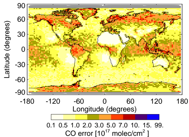
Fig. 7. Global distribution of the average SCIAMACHY CO monthly-mean instrument-noise error on a 3° by 2° grid for the year 2004 for IMLM version 7.4 over land and sea. Blue indicates large instrument-noise errors, white indicates small instrument-noise errors. The data over land are the same as in Fig. 2.
