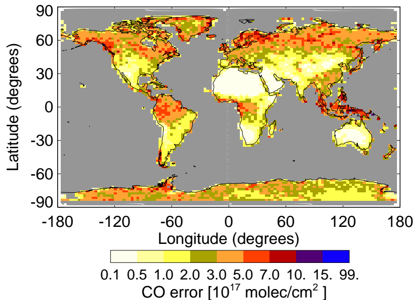
Fig. 2. Global distribution of the SCIAMACHY CO monthly-mean instrument-noise error on a 3^\circ by 2^\circ grid for the year 2004 for IMLM version 7.4. Blue indicates large instrument-noise errors, white indicates small instrument-noise errors.
