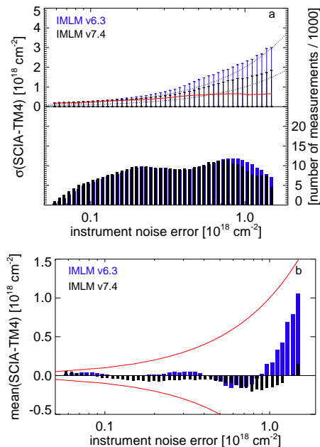
Fig. 3. Comparison of the SCIAMACHY CO total columns from the IMLM retrieval version 6.3 and 7.4 based on single SCIAMACHY measurements for the period January to December 2004. (a) Root mean square (rms) values of the differences between the single SCIAMACHY CO measurements and the spatially and temporally collocated TM4 CO total columns as function of the instrument noise error. The blue bars indicate the distribution based on IMLM v6.3 retrievals, the black bars based on IMLM v7.4 retrievals. The dotted lines indicate the 1- and 2- \sigma instrument-noise error levels. The red line indicates the rms value of the TM4 simulated CO total columns, which is caused by spatio-temporal CO total column variations because observations with similar instrument-noise errors can be scattered around the globe. The blue (IMLMv6.3) and black (IMLMv7.4) bars in the bottom panel denote the number of measurements for each instrument-noise interval. (b) Average differences between the single SCIAMACHY CO measurements and the spatially and temporally collocated TM4 CO total columns as function of the instrument-noise error. The bars indicate the mean difference for each instrument-noise interval. The blue bars indicate data from the IMLM retrieval version 6.3, the black bars version 7.4. The red line indicates the 1- \sigma instrument-noise error levels.
