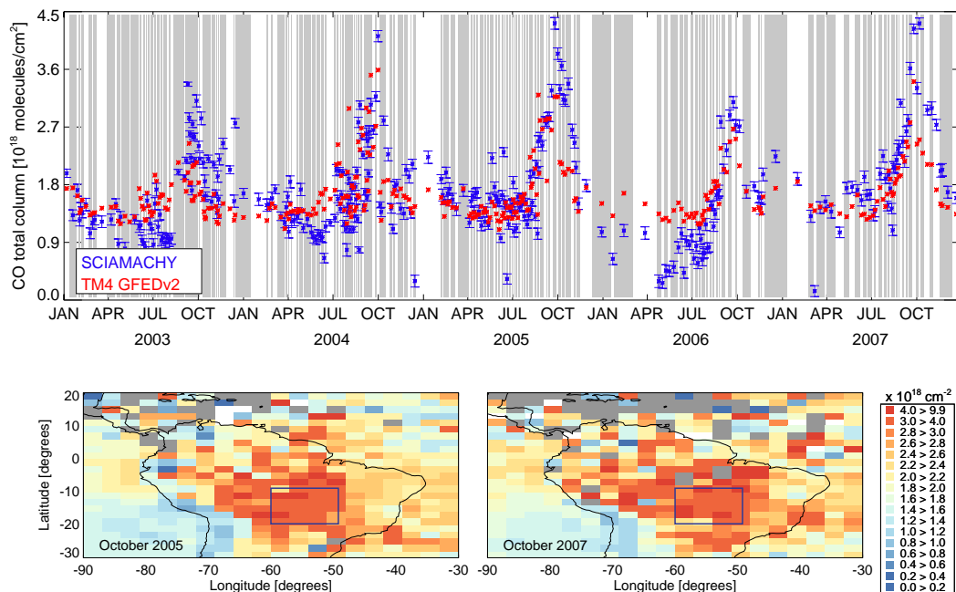
Fig. 14. Top panel: Timeseries for the period January 2003–December 2007 over Brazil using SCIAMACHY CO measurements averaged over the area indicated by the blue boxes in the bottom panels. The SCIAMACHY CO measurements are averaged over a varying time period indicated by the grey vertical bars in order to obtain an instrument-noise error of 1 \times 10^{17} \text{ cm}^{-2} for each SCIAMACHY data point (blue). The red stars indicate the spatially and temporally collocated TM4 CO total columns. Note that in October 2004, 2005, and 2007 the CO total columns are significantly higher than in October 2003 and 2006. Bottom left panel: Brazil in October 2005. Monthly mean 3^\circ \times 2^\circ SCIAMACHY CO total columns. Over sea the columns below the clouds are filled with TM4 values. Over land SCIAMACHY CO total columns are shown (cf. Sect. 3). Blue indicates low CO columns and red high CO columns. Bottom right panel: as bottom left panel, but for October 2007.
