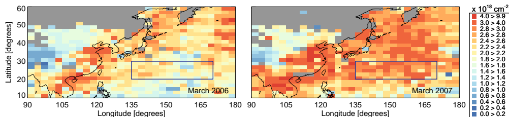
Fig. 12. Top panel: Timeseries for the period January 2003–December 2007 using SCIAMACHY CO measurements averaged over the area East of China as indicated by the blue boxes in the bottom panels. The SCIAMACHY CO measurements are averaged over a varying time period indicated by the grey vertical bars in order to obtain an instrument-noise error of 1 \times 10^{17} \text{ cm}^{-2} for each SCIAMACHY data point (blue). The red stars indicate the spatially and temporally collocated TM4 CO total columns. The SCIAMACHY CO columns above the clouded ocean scenes are filled with the TM4 CO column below clouds to obtain a total column. Year-to-year variations are clearly seen. Bottom left panel: Asian outflow in March 2006. Monthly mean 3^\circ \times 2^\circ SCIAMACHY CO total columns. Over sea the columns below the clouds are filled with TM4 values. Blue indicates low CO columns and red high CO columns. Bottom right panel: as bottom left panel, but for March 2007.
