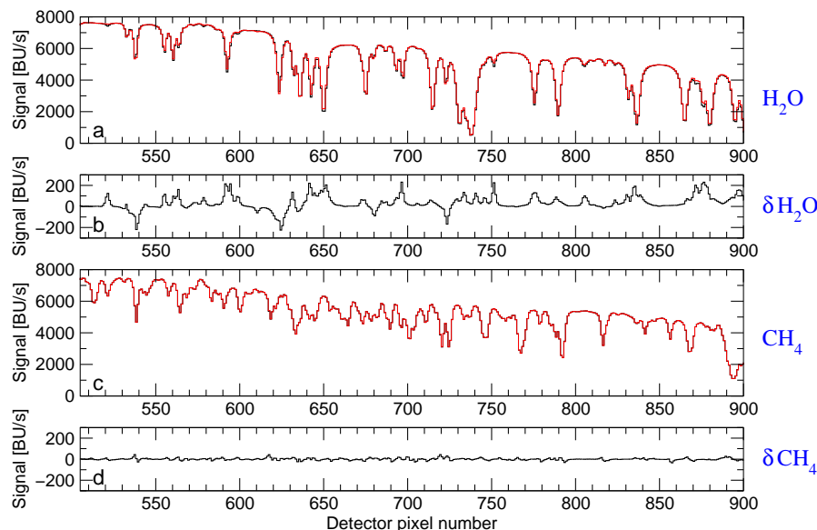
Fig. 1. Differences between HITRAN 2004 and the new spectroscopy used in this paper (see text). The simulated atmospheric spectra shown are at SCIAMACHY spectral resolution. The retrieval window used for CO retrievals lies between detector pixel 505 and 615 corresponding to the wavelength range 2324.5–2337.9 nm. (a) Simulated atmospheric reflectance spectra of the H 2 O lines using the HITRAN 2004 database (black) and the new database from Jenouvrier et al. (2007) (red). (b) Difference between the red and black curves from panel a. (c) Simulated atmospheric reflectance spectra of the CH 4 lines using the HITRAN 2004 database (black) and the new database from Predoi-Cross et al. (2006) (red). (d) Difference between the red and black curves from panel c.
