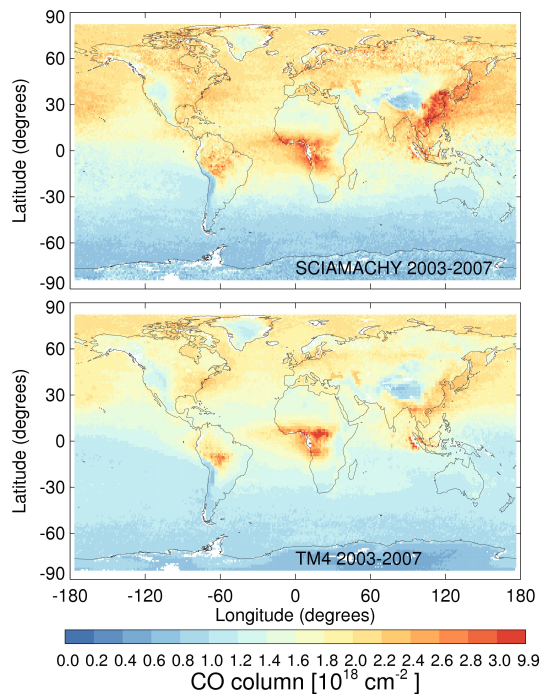
Fig. 11. Five year average CO total columns on a 1° by 1° grid. Top: SCIAMACHY CO. Bottom: TM4. Blue indicates low CO columns and red high CO columns. Note that the SCIAMACHY CO columns above low clouds over sea are filled up with TM4 CO below the cloud to obtain total columns.
