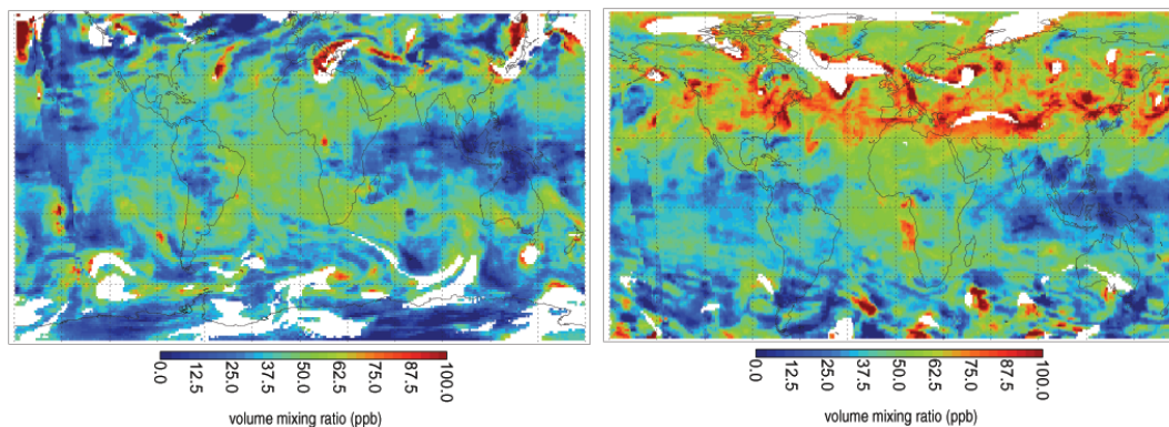
Fig. 1. Column-mean O 3 tropospheric mixing ratio derived from OMI/MLS for 1 January (left) and 1 July 2005 (right). Missing values (white areas) occur where either no data are available or where quality control checks flag the data as suspect (see text).
