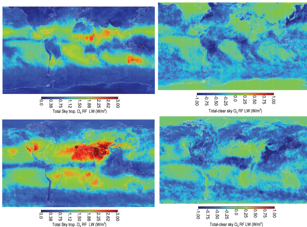
Fig. 5. Total-sky long-wave (LW) tropospheric O 3 RE in 2005: January (top left) and July (bottom left); Total minus clear-sky LW RE: January (top right) and July (bottom right).
