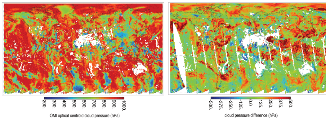
Fig. 3. Gridbox mean optical centroid cloud pressure (OCCP) from OMI (left) and OCCP minus MODIS cloud-top pressure (right) for 1 July 2005.
