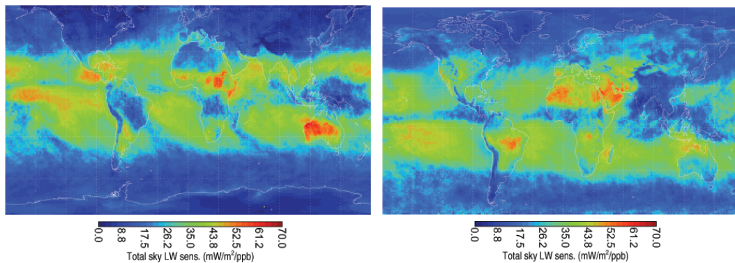
Fig. 6. Sensitivity of the LW RE to ozone mixing ratio for January (left) and July (right) 2005.
