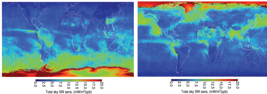
Fig. 8. Sensitivity of the SW RE to ozone mixing ratio for January (left) and July (right) 2005.
