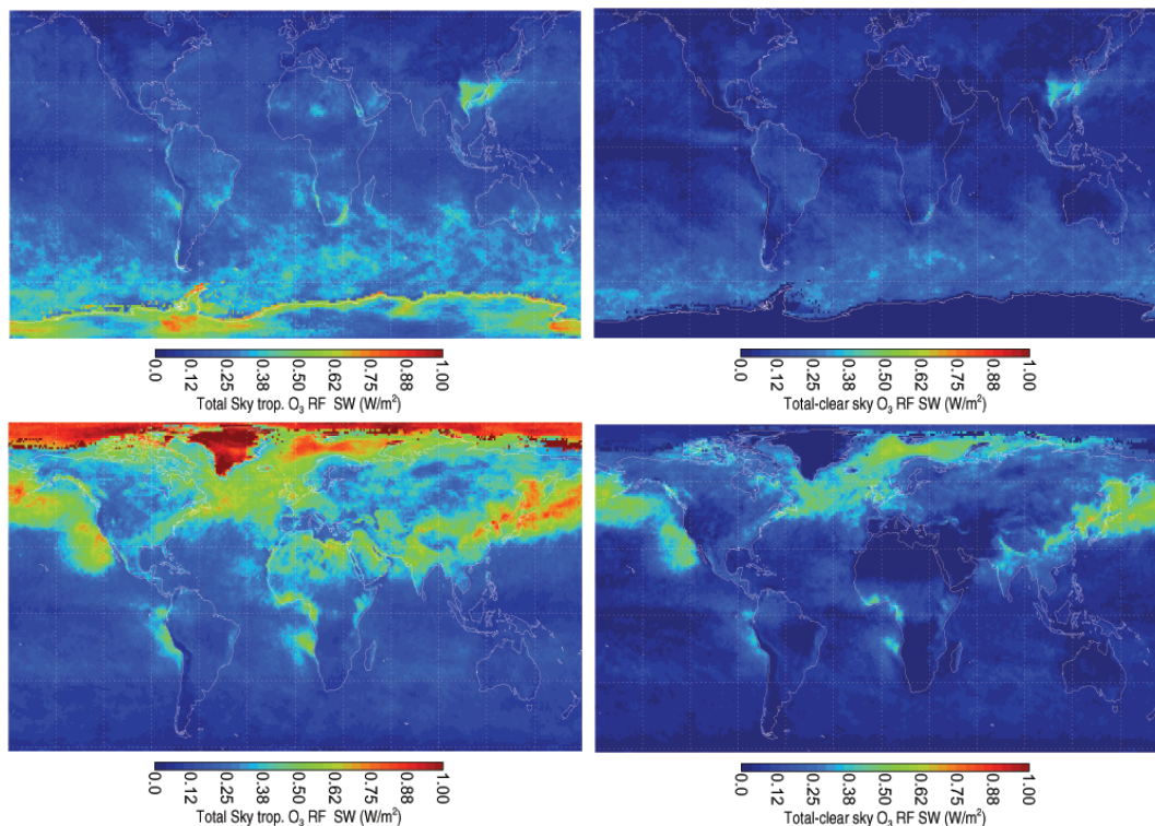
Fig. 7. Total-sky short-wave (SW) tropospheric O 3 RE in 2005: January (top left) and July (bottom left); Total minus clear-sky SW RE: January (top right) and July (bottom right).
