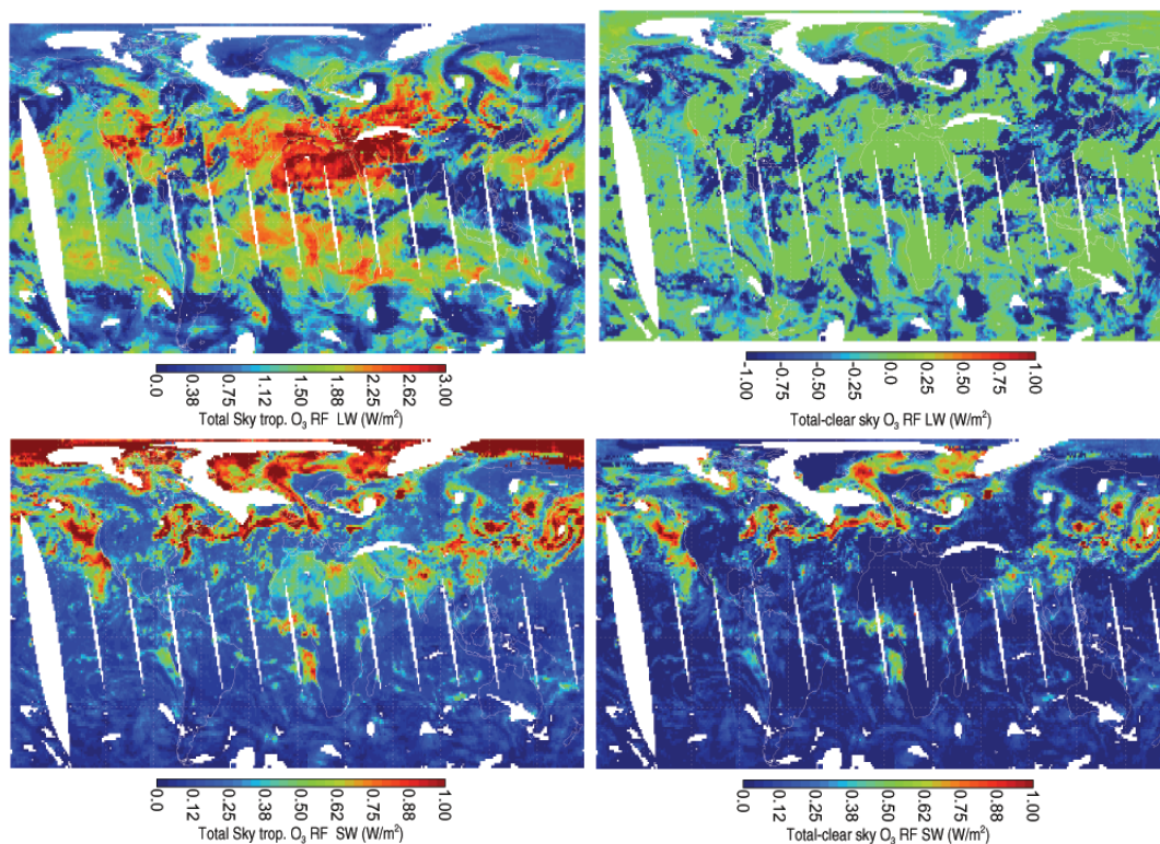
Fig. 4. Instantaneous (unadjusted) daily-averaged total-sky tropospheric O 3 radiative effect (RE): Long-wave (top left) and short-wave (bottom left); Total minus clear-sky RE: Long-wave (top right) and short-wave (bottom right) on 1 July 2005.
