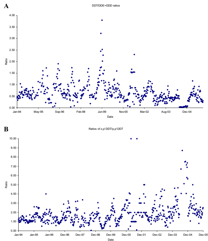
Fig. 4. Ratios of DDT/DDE+DDD ( A ) to show the age of the DDT signal, and o,p' -DDT/ p,p' -DDT ( B ) to determine whether sources are from Dicofol or Technical DDT.
