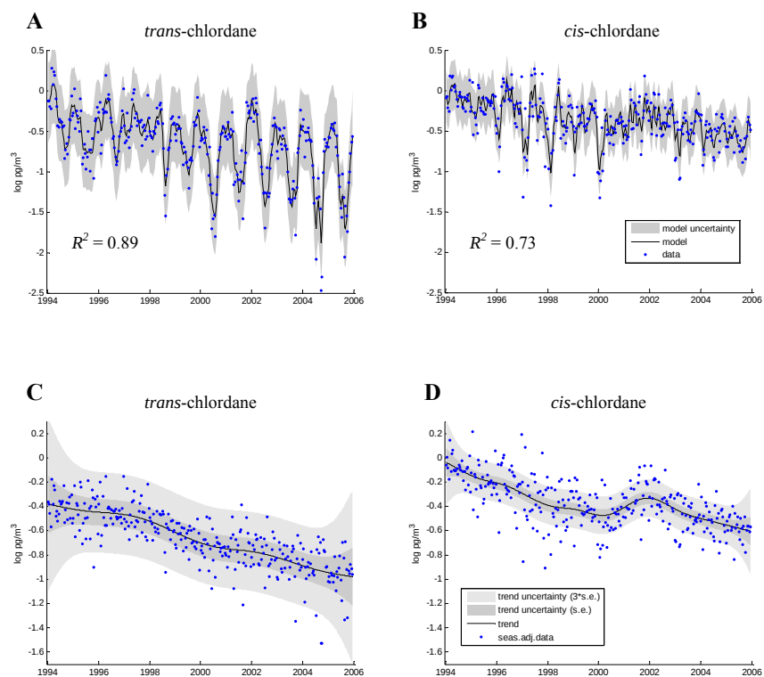
Fig. 1. Measured data and model fit for trans -chlordane ( A ) and cis -chlordane ( B ) with goodness of fit ( R^2 ). Seasonally adjusted data and underlying trend are provided in plots ( C ) ( trans -chlordane) and ( D ) ( cis -chlordane).
