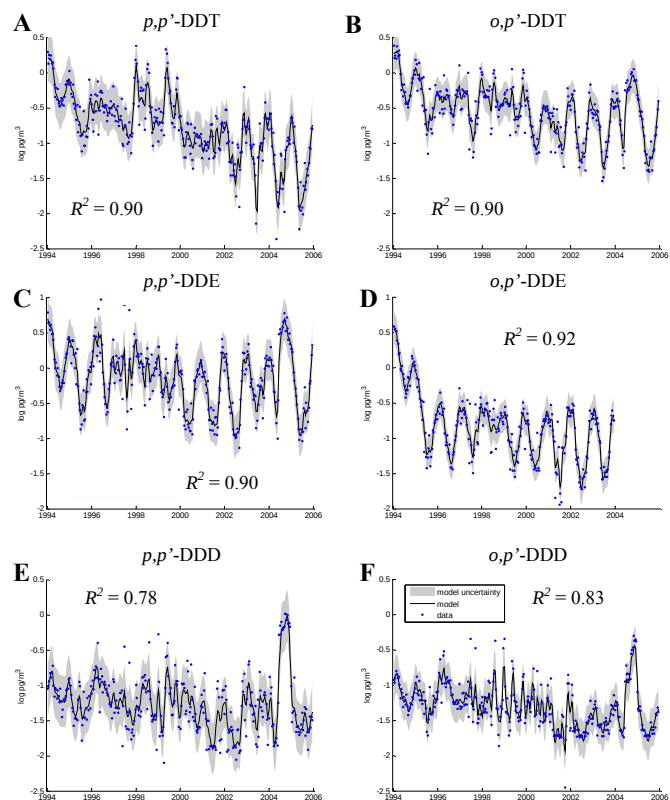
Fig. 3. Measured data and model fit for p,p' -DDT ( A ); o,p' -DDT ( B ); p,p' -DDE ( C ); o,p' -DDE ( D ); p,p' -DDD ( E ) and o,p' -DDD ( F ). Goodness of fit is provided in each case ( R^2 ).
