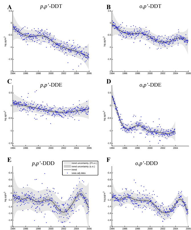
Fig. 5. Seasonally adjusted data and underlying trend for p,p' -DDT (A); o,p' -DDT (B); p,p' -DDE (C); o,p' -DDE (D); p,p' -DDD (E) and o,p' -DDD (F). ( o,p' -DDE excludes 2004–2005).
