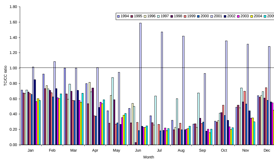
Fig. 2. Average monthly TC/CC ratios at Zeppelin 1994–2005.
