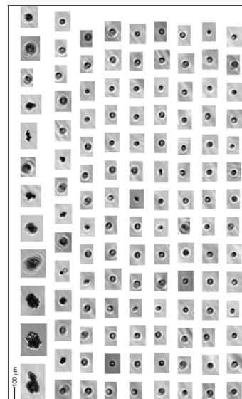
Fig. 10. Experiment IN04_31 showing ice nucleation on SD2 at -25^{\circ}\text{C} . Plot captions are as for Fig. 6.
