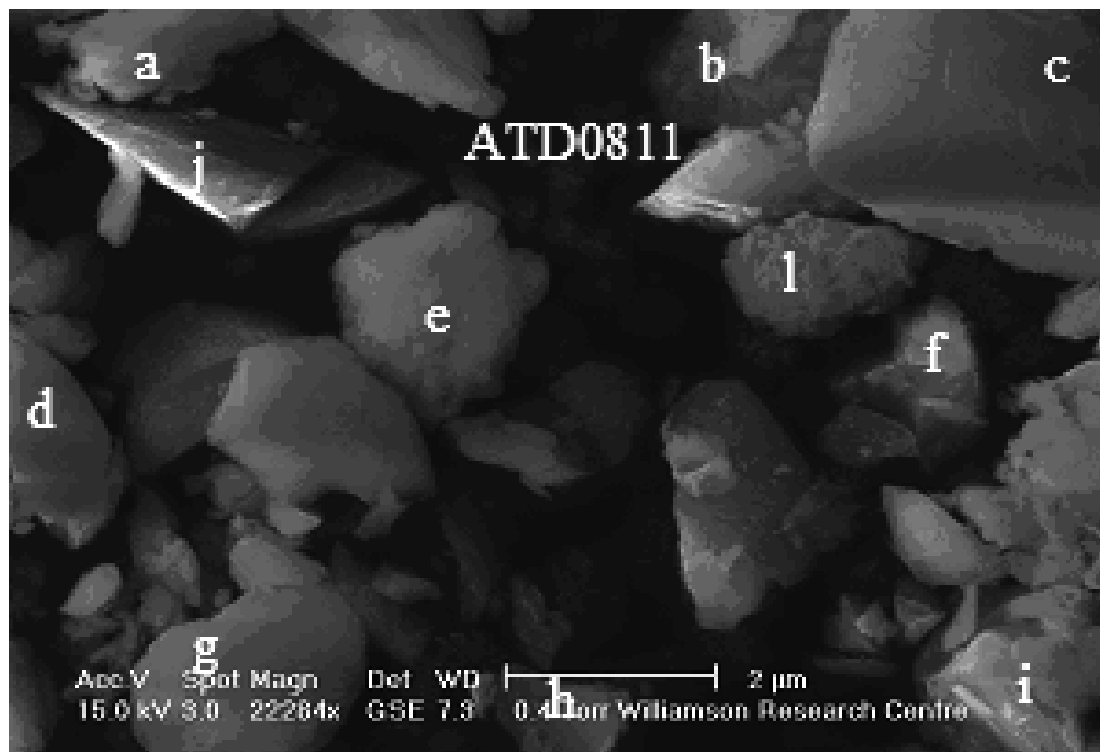
Fig. 12. ATD ESEM image (Sample ATD0811) showing both granular (or shocked, e.g. “l”) and smooth faceted morphologies. Particles labelled “a” to “j” represent selected locations for EDX spot elemental analysis (scale 2 \mu\text{m} ).
