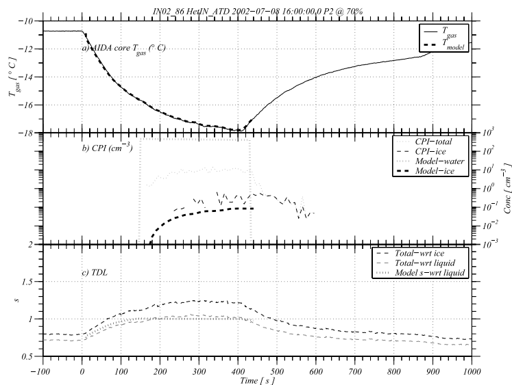
Fig. 5. Experiment IN02_86 showing freezing on ATD at -16^{\circ}\text{C} . (a) shows the measured (black line) and modelled air temperature (thick black dashed line); (b) shows the CPI measured total concentration (grey dotted line) and ice (black solid line), the modelled liquid and ice concentrations are shown by the thicker dotted grey and dashed black lines, respectively; (c) shows the measured total water content converted to an equivalent saturation ratio wrt. ice (black dashed line) and saturation wrt. liquid (grey dashed line), the thicker dotted line is the modelled RH (no TDL measurements were available for this experiment). Ice crystal images observed are shown on the right.
