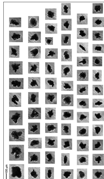
Fig. 11. Experiment IN05_58 showing freezing on SD2 at -26^{\circ}\text{C} . Plot captions are as for Fig. 8.
