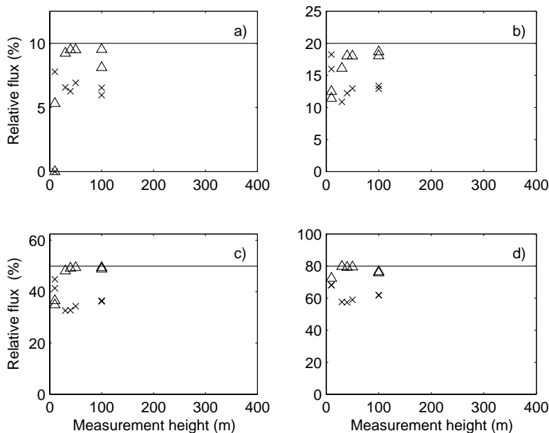
Fig. 8. The relative fluxes from the LES (crosses) and FW (triangles) predictions from (a) \Omega_{10}^N , (b) \Omega_{20}^N , (c) \Omega_{50}^N and (d) \Omega_{80}^N in the case 2 (neutral). Results shown only for selected grid resolutions (see Sect. 2.4 for criteria).
