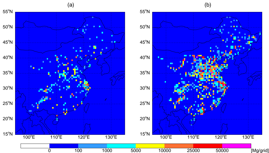
Fig. 5. NO x emission increase from China's power plants. (a) NO x emission change from China's power plants between 2001 and 1996. (b) NO x emission change from China's power plants between 2006 and 2001 (units: Mg per grid).
