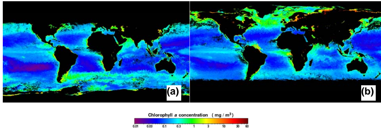
Figure S1. Chlorophyll a concentrations for a) January and b) July, 2001 from SeaWiFS ( http://oceancolor.gsfc.nasa.gov/cgi/13 ).
