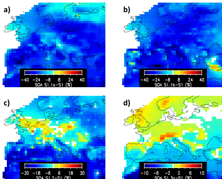
Fig. 1. Relative differences of surface SOA between sensitivity cases and the reference simulation S1 over Europe for JJA 2002: (a) S1.1a, using MEGAN isoprene emissions; (b) S1.1b, using European isoprene standard emission factors from Karl et al. (2008); (c) S1.2, applying the \text{NO}_x dependence of isoprene SOA; (d) S1.3a, applying \Delta H_{\text{vap}} = 72.7 \text{ kJ mol}^{-1} for the temperature dependence of K for isoprene oxidation products; (e) S1.5, replacing the BC/POC fossil fuel/biofuel emission inventory with a detailed technology based European inventory; (f) S2, using the combination of parameters according to current state of knowledge. Changes are only plotted for areas where SOA surface concentrations are above 0.25 \mu\text{g m}^{-3} . Thus white colors either indicate low concentrations or small changes.
