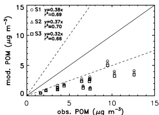
Fig. 4. Comparison of yearly averaged (July 2002 to June 2003) modelled (S1) and observed particulate organic matter (POM) for 13 surface stations during the 2002/2003 EMEP campaign on OC/EC. Measured OC concentrations were converted to POM using the station specific OM/OC ratios ranging from 1.4 to 1.8, provided by Yttri et al. (2007). Yearly average of modelled POM is based only on those days when measurements were done at the EMEP stations. Model results from the base simulation S1 (circle), S2 (triangle) and from the simulation without SOA formation from isoprene, S3 (square).
