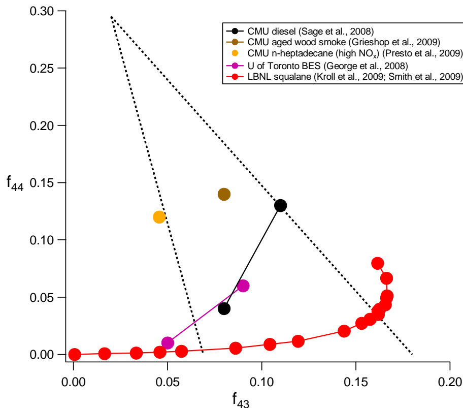
Fig. 8. Chamber and flow tube data from the photooxidation/heterogeneous oxidation of POA. The LBNL squalane data and CMU n-heptadecane data are HR data (the m/z 43 data shown are from the C_2H_3O^+ fragment). For diesel and wood smoke (Sage et al., 2008; Grieshop et al., 2009), the data shown here are from the residual mass spectra (i.e. spectra in which the POA contribution has been excluded). The LBNL squalane data starts from zero because the experiment starts with HOA. The two dotted lines are the same as those in Fig. 4.
