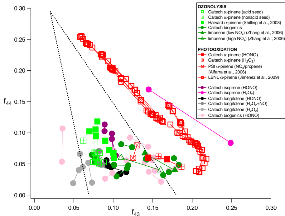
Fig. 6. f_{44} vs. f_{43} for SOA formed by the ozonolysis/photooxidation of a suite of biogenic precursors from chamber experiments, including isoprene, terpenes, and sesquiterpenes (Gao et al., 2004ab; Bahreini et al., 2005; Kroll et al., 2006; Lee et al., 2006a,b; Ng et al., 2006, 2007a). Also shown in this figure are flow tube data of the heterogeneous oxidation (by OH radicals) of SOA formed from \alpha -pinene photooxidation (LBNL data). The lines connecting the data points indicate the range of f_{44} and f_{43} observed in each experiment. For \alpha -pinene ozonolysis, only the values at the end of the experiment are shown to avoid crowding the plot. The two dotted lines are the same as those in Fig. 4.
