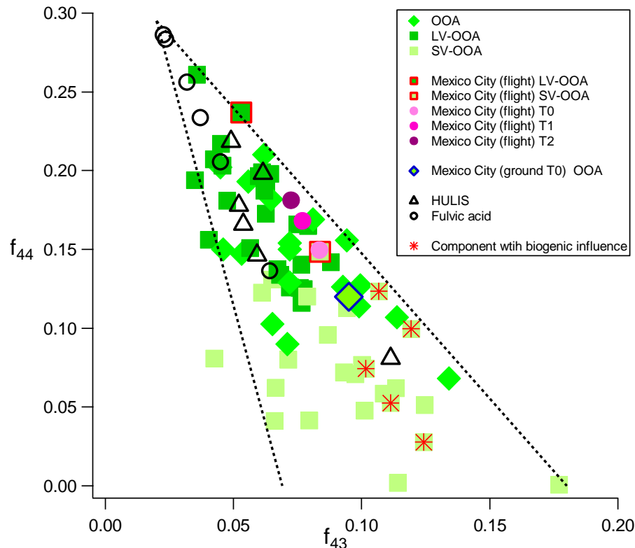
Fig. 4. f_{44} vs. f_{43} for all the OOA components from different sites, including Mexico city ground and flight data (Aiken et al., 2009; Jimenez et al., 2009), as well as various HULIS (humic-like substances) and fulvic acid samples. The dotted lines are added to guide the eye and define the triangular space where ambient OOA components fall. Coordinates for the line on the left hand side are (0.02, 0.295) and (0.069, 0); coordinates for the line on the right hand side are (0.02, 0.295) and (0.18, 0). Uncertainties in f_{44} and f_{43} of these components are discussed in the text.
