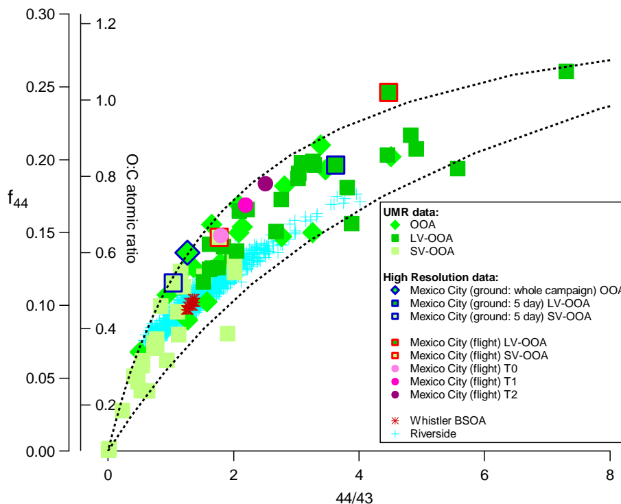
Fig. 5. f_{44} and O:C vs. 44/43 for all the OOA components from different sites, including Mexico city ground (whole campaign and 5 day) (Aiken et al., 2008, 2009) and flight data (Jimenez et al., 2009). Also shown are the time-dependent data of the OOA components at Riverside, as well as data obtained during a biogenics SOA event at Whistler. For the UMR data, O:C is estimated using the f_{44} of the PMF-resolved factor mass spectra and the correlation derived by Aiken et al. (2008); for the HR data the O:C is directly determined by elemental analysis (hence the f_{44} axis does not apply to the HR data). The two dotted curves represent the mathematical transformation of the two lines in Fig. 4.
