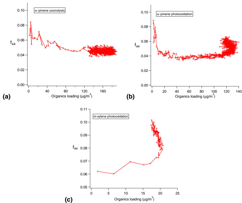
Fig. 11. (a) Change in f_{44} as a function of organics loading over the course of a typical \alpha -pinene ozonolysis experiment. (b) Change in f_{44} as a function of organics loading over the course of a typical \alpha -pinene photooxidation experiment (low- \text{NO}_x ). (c) Change in f_{44} as a function of organics loading over the course of a typical m -xylene photooxidation experiment (low- \text{NO}_x ).
