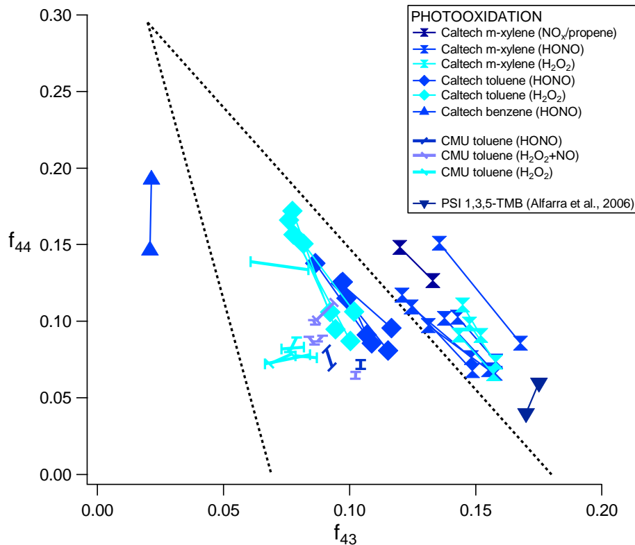
Fig. 7. Chamber data from the photooxidation of a series of aromatic hydrocarbons, including m -xylene, toluene, benzene, and 1,3,5-trimethylbenzene (Ng et al., 2007b; Hildebrandt et al., 2009). The lines connecting the data points indicate the range of f_{44} and f_{43} observed in each experiment. The two dotted lines are the same as those in Fig. 4.
