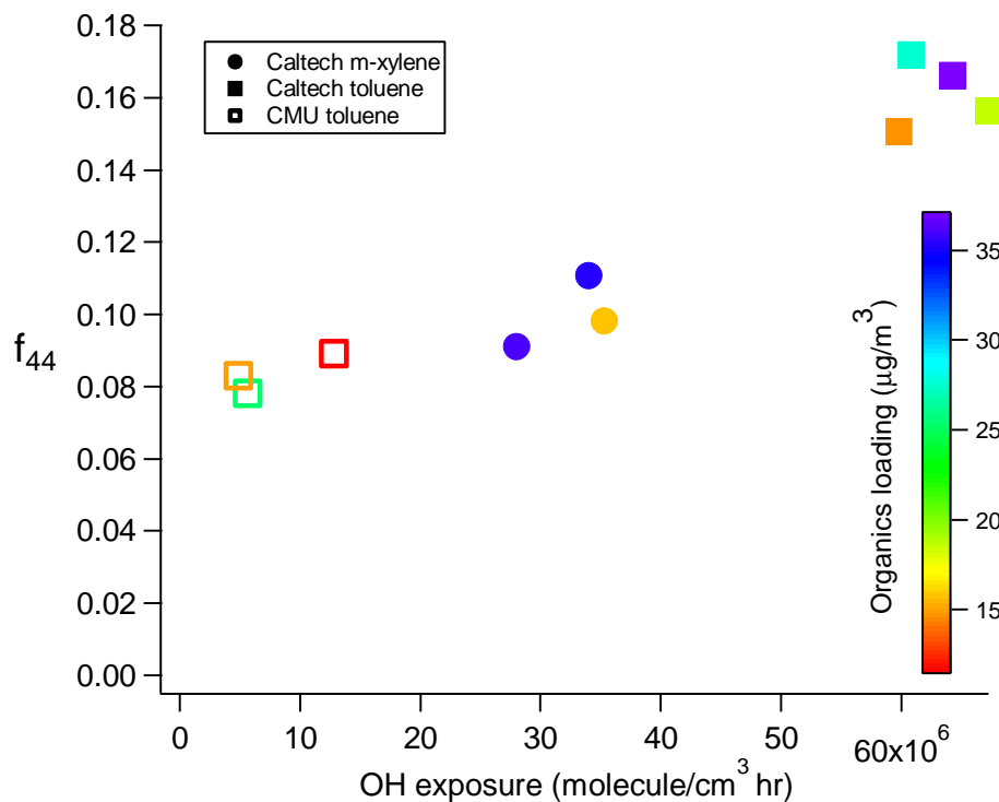
Fig. 10. f_{44} (highest f_{44} observed in the experiment) vs. the OH exposure for SOA formed from the photooxidation of m -xylene and toluene under low- \text{NO}_x ( \text{H}_2\text{O}_2 ) conditions (Ng et al., 2007b; Hildebrandt et al., 2009). Each data point is colored according to the loading of that particular experiment.
