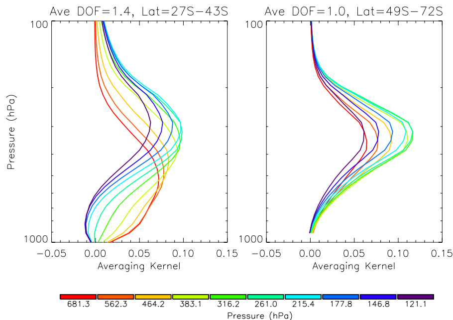
Fig. 3. Mean TES Averaging Kernels of selected observations, 12–19 December 2006. Profile selection criteria: cloudOD <2.0, CO >120 ppb at 215 hPa or 681 hPa. Profiles used for the left panel are in latitude band of 27° S–43° S (num of profiles for averaging=15). Profiles used for the right panel are in latitude band of 49° S–72° S (num of profiles for averaging=12).
