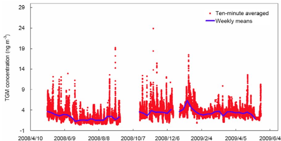
Fig. 2. Time series of total gaseous mercury (TGM) in Mt. Leigong.
