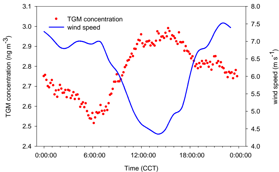
Fig. 7. Averaged diurnal variations of TGM and wind speed in Mt. Leigong.
