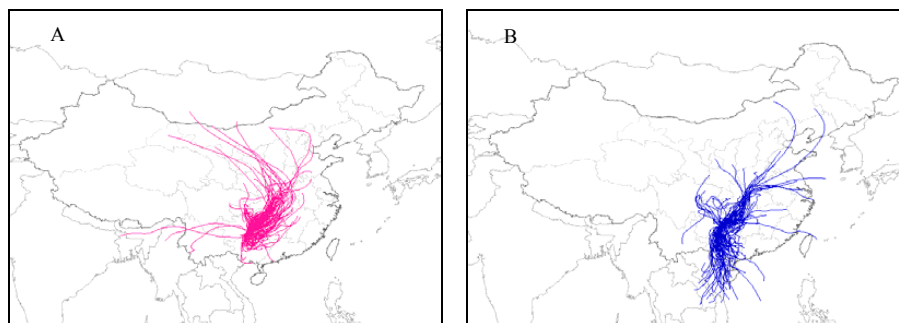
Fig. 6. 72-h back trajectories of air masses in Mt. Leigong in (A) cold seasons (October, November, December, and January) (B) warm seasons (May, June, July, and August).
