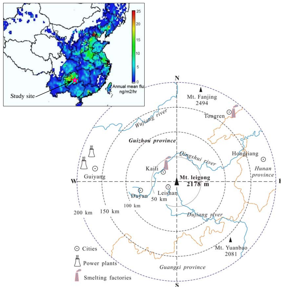
Fig. 1. Map showing the distribution of girded anthropogenic Hg emission (Shetty et al., 2008, and reference therein) and sampling site.
