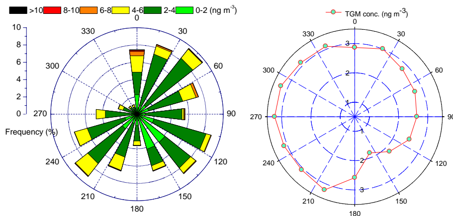
Fig. 8. Pollution roses showing (A) frequency of wind direction and TGM (B) TGM concentrations during daytime.
