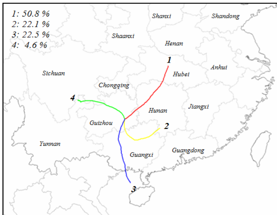
Fig. 9. Four types of 3-day back trajectories arriving at the study site.
