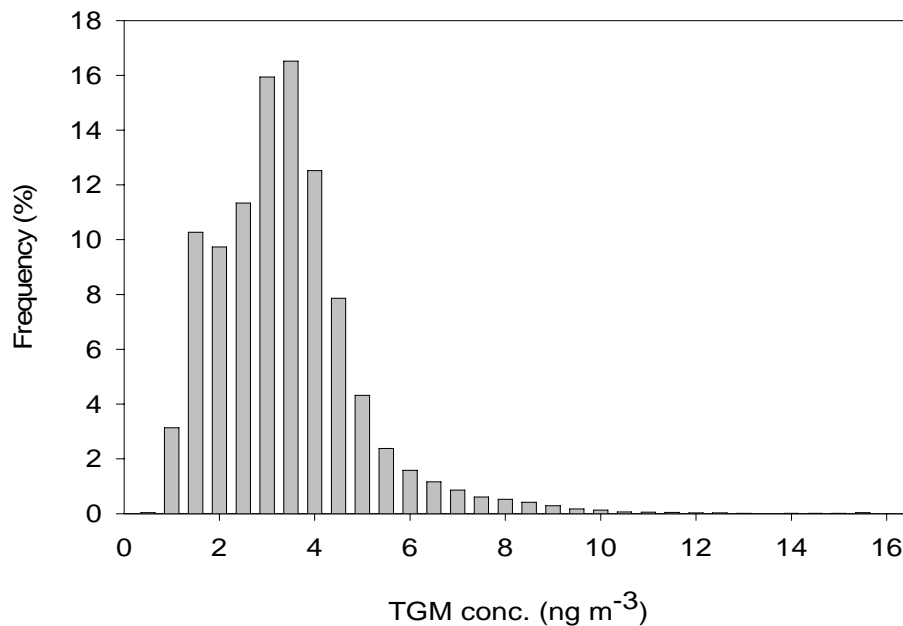
Fig. 3. Frequency distribution of TGM covered the whole period.
