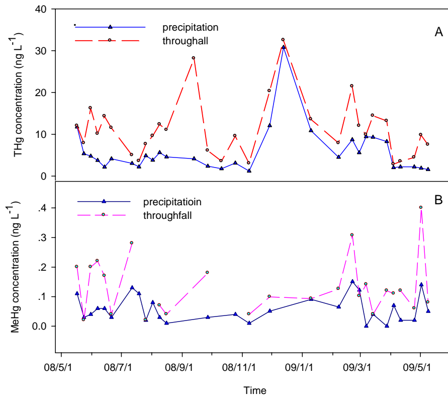
Fig. 4. Weekly concentrations of (A) THg and (B) MeHg in precipitation and throughfall collected in Mt. Leigong from May 2008 to May 2009.
