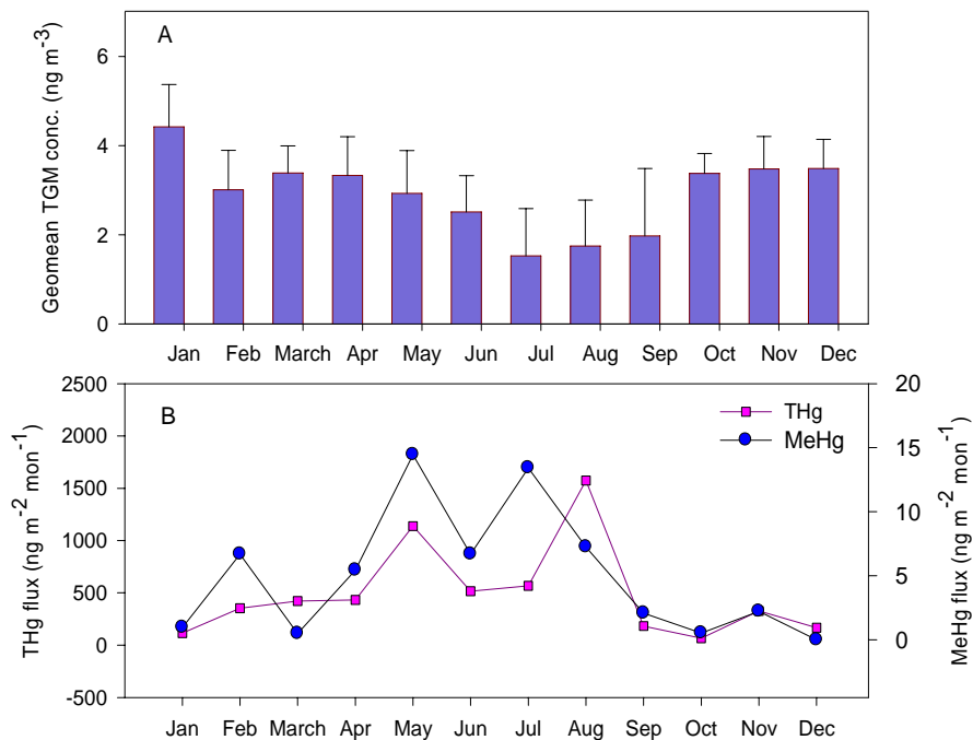
Fig. 5. Monthly variations of (A) TGM and (B) THg and MeHg direct wet deposition fluxes in Mt. Leigong.
