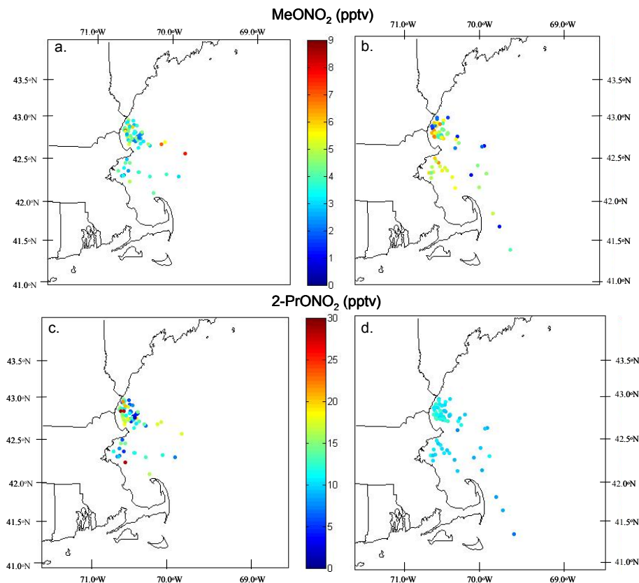
Fig. 8. Air and surface seawater samples (pptv) collected in the Gulf of Maine onboard the NOAA Ship Ronald H. Brown during NEAQS 2002 throughout 30 July–6 August 2002: (a) ambient air and (b) surface seawater mixing ratios of MeONO 2 ; (c) ambient air and (d) surface seawater mixing ratios of 2-PrONO 2 .
