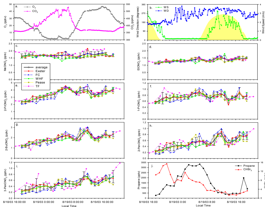
Fig. 9. (a) 10 min average O 3 (ppbv) and CO 2 (ppmv) mixing ratios and (b) wind speed (m/s), wind direction, and J_{\text{NO}_2} (yellow shaded curve) at Thompson Farm from 18 August at 16:00 to 19 August 2003 at 22:00 (LT). Alkyl nitrate mixing ratios (pptv) at four sites throughout the Great Bay estuary and at Thompson Farm: (c) MeONO 2 , (d) EtONO 2 , (e) 2-PrONO 2 , (f) 1-PrONO 2 , (g) 2-BuONO 2 , (h) 2-PeONO 2 , (i) 3-PeONO 2 , and (j) hourly average propane and CHBr 3 mixing ratios (pptv) for the five sampling sites. (c–i) The black line is the average \pm standard deviation mixing ratio of all 5 sites each hour.
