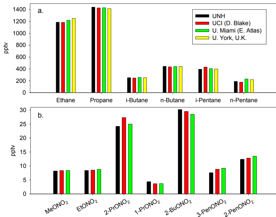
Fig. 2. Alkyl nitrate and NMHC measurement intercomparison between the University of New Hampshire, University of California-Irvine, University of Miami, and University of York, UK (NMHCs only) laboratories. Each bar is the average mixing ratio (pptv) of four canister samples analyzed by each laboratory.
