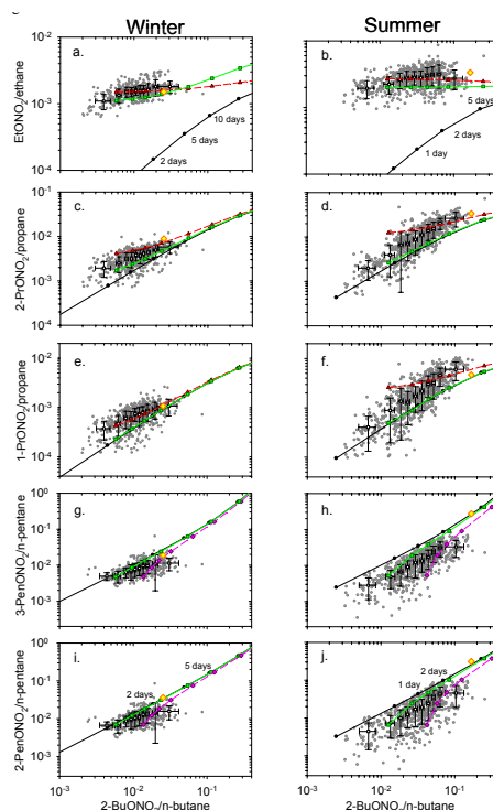
Fig. 10. Alkyl nitrate/parent hydrocarbon ratios versus 2-BuONO 2 / n -butane for Winter (left) and Summer (right) 2002: (a) and (b) EtONO 2 /ethane, (c) and (d) 2-PrONO 2 /propane, (e) and (f) 1-PrONO 2 /propane, (g) and (h) 3-PenONO 2 / n -pentane, and (i) and (j) 2-PenONO 2 / n -pentane. The white squares are averages each containing 10% of the data. Error bars represent \pm 1 standard deviation of the 2-BuONO 2 / n -butane ratio in the x -direction and \pm 1 standard deviation of the RONO 2 /RH ratio in the y -direction. Solid black line and circles: [RONO 2 ] o /[RH] o =0, the black dots correspond to the number of days since the parent alkane was emitted; (a–f) red dashed line with triangles: [RONO 2 ] o /[RH] o =seasonal mean and [2-BuONO 2 ] o /[ n -butane] o =seasonal background; green lines with squares: [RONO 2 ] o /[RH] o and [2-BuONO 2 ] o /[ n -butane] o =seasonal background; (g–j) pink dashed lines with diamonds: [PenONO 2 ] o /[ n -pentane] o =seasonal background and [2-BuONO 2 ] o /[ n -butane] o =seasonal mean. See Table 5 for initial ratio values. The yellow diamonds are RONO 2 /RH ratios from samples collected at remote sites along the US west coast in December 2001 and June 2002.
