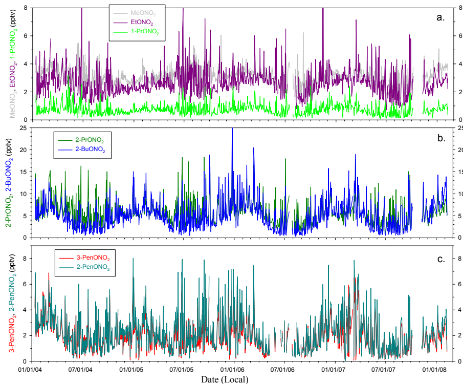
Fig. 4. Time series of (a) MeONO 2 , EtONO 2 , 1-PrONO 2 , (b) 2-PrONO 2 , 2-BuONO 2 , and (c) 2-PenONO 2 , 3-PenONO 2 (pptv) from daily canister samples collected at Thompson Farm during 12 January 2004 to 8 February 2008.
