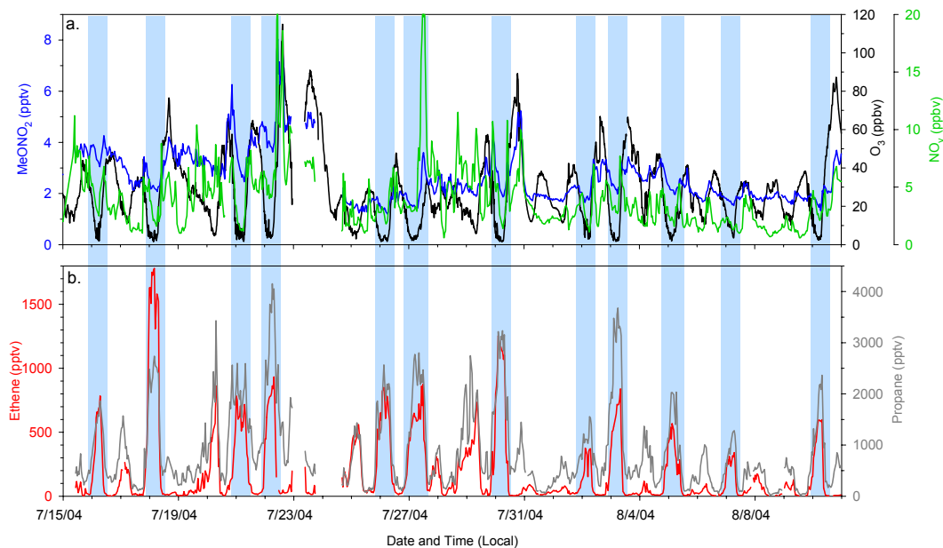
Fig. 7. Time series of (a) MeONO 2 (pptv), O 3 (ppbv), NO y (ppbv) and (b) ethene and propane (pptv) at Thompson Farm during 15 July to 11 August 2004. Shaded regions are nights with O 3 ≤ 5 ppbv and wind speed < 0.5 m/s indicating that a strong and stable inversion layer had developed.
