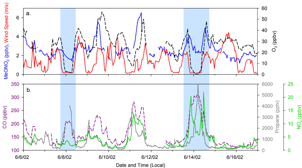
Fig. 6. Time series of (a) MeONO 2 (pptv), O 3 (ppbv) and wind speed (m/s) and (b) CO (ppbv), propane (pptv) and NO y (ppbv) at Thompson Farm during 6–16 June 2002. Shaded regions are the nights of 8 and 14 June.
