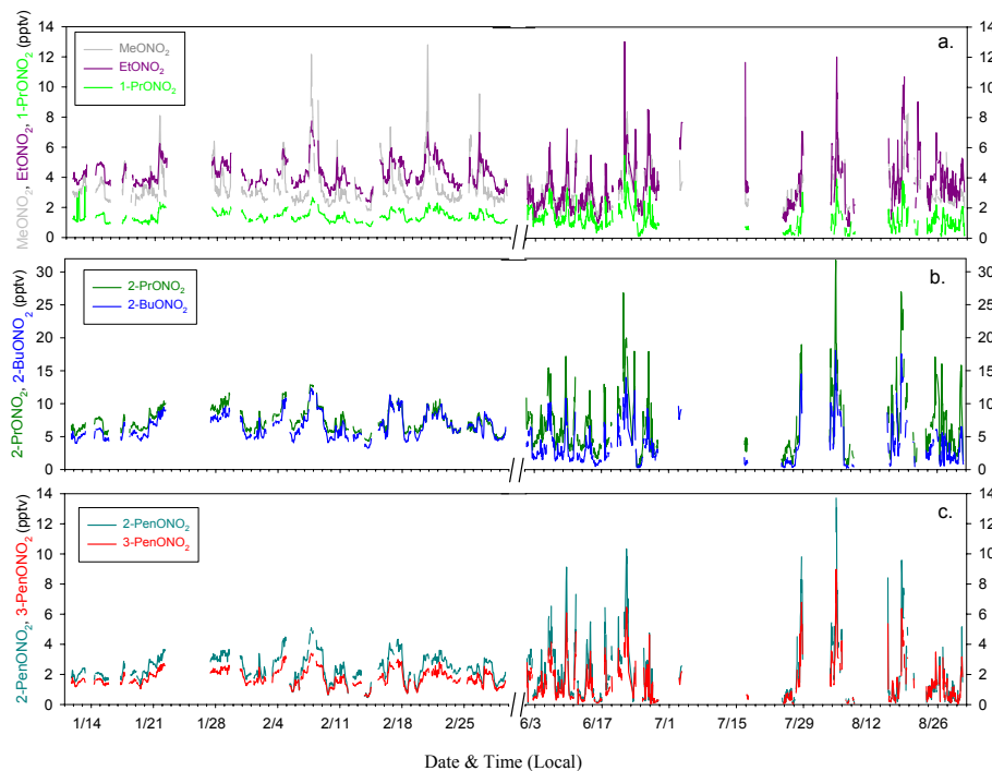
Fig. 3. Time series of (a) MeONO 2 , EtONO 2 , 1-PrONO 2 , (b) 2-PrONO 2 , 2-BuONO 2 , and (c) 2-PenONO 2 , 3-PenONO 2 (pptv) during winter (11 January–1 March) and summer (1 June–31 August) 2002. Note: there is a break in the x-axis during March–May 2002.
