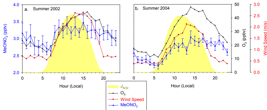
Fig. 5. Hourly average (LT) O 3 (ppbv), wind speed (m/s), J_{\text{NO}_2} (yellow shaded curve), and MeONO 2 ( \pm standard error) (pptv) using all data during (a) 1 June to 31 August 2002 and (b) 1 July to 15 August 2004 at Thompson Farm.
