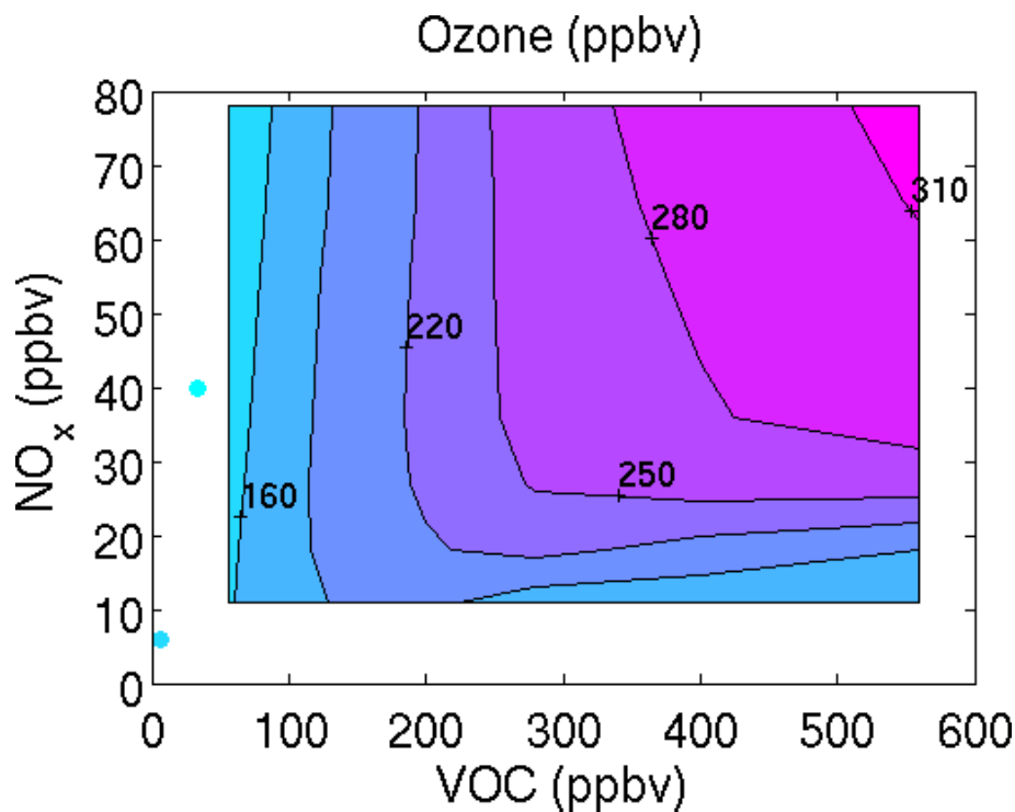
Fig. 8. Isopleths of the ozone concentrations as a function of NO x and VOCs concentrations. This is interpolated from the calculation of 49 sensitivity tests using the box model as done for the so called additional petrochemical accident run.
