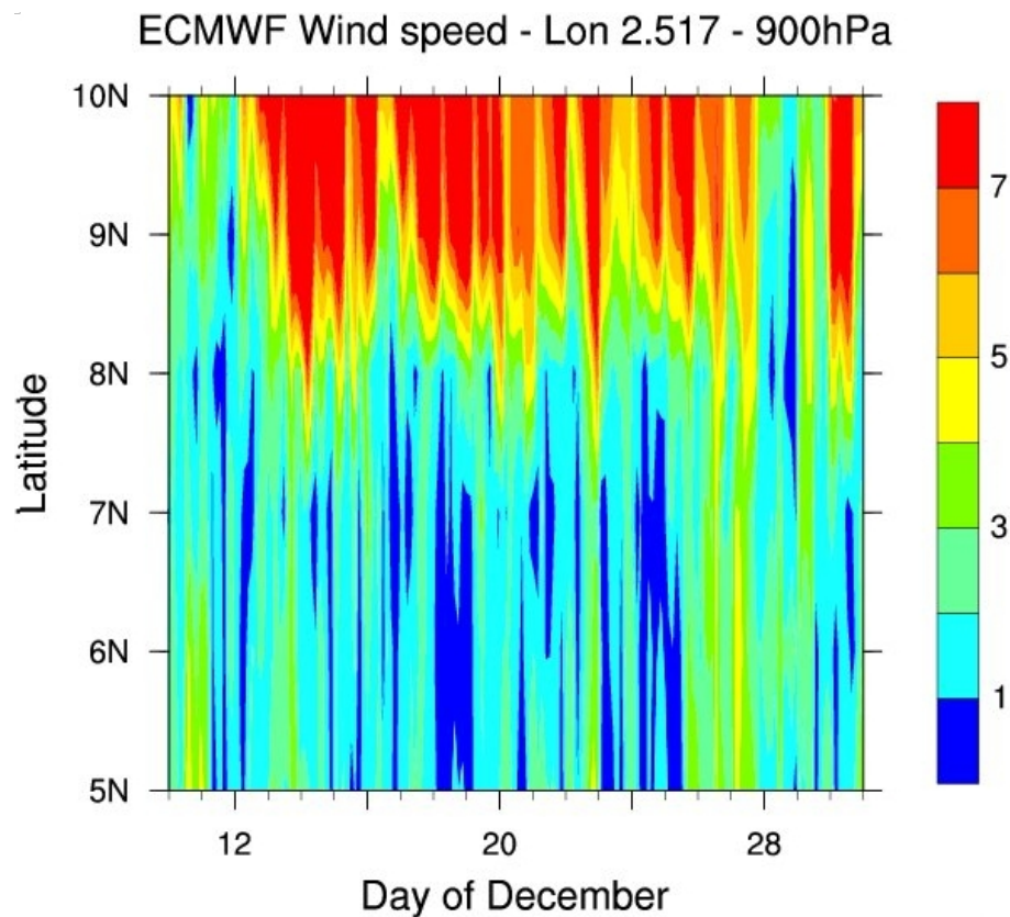
Fig. 5. Hovmoeller diagram of the wind speed ( \text{m s}^{-1} ) at 900 hPa at the longitude of Cotonou ( 2.5^\circ \text{ E} ) from ECMWF analysis.
