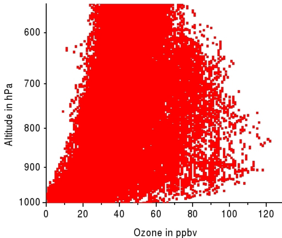
Fig. 3. Scatter plots of ozone over Lagos based on 361 MOZAIC vertical profiles.
