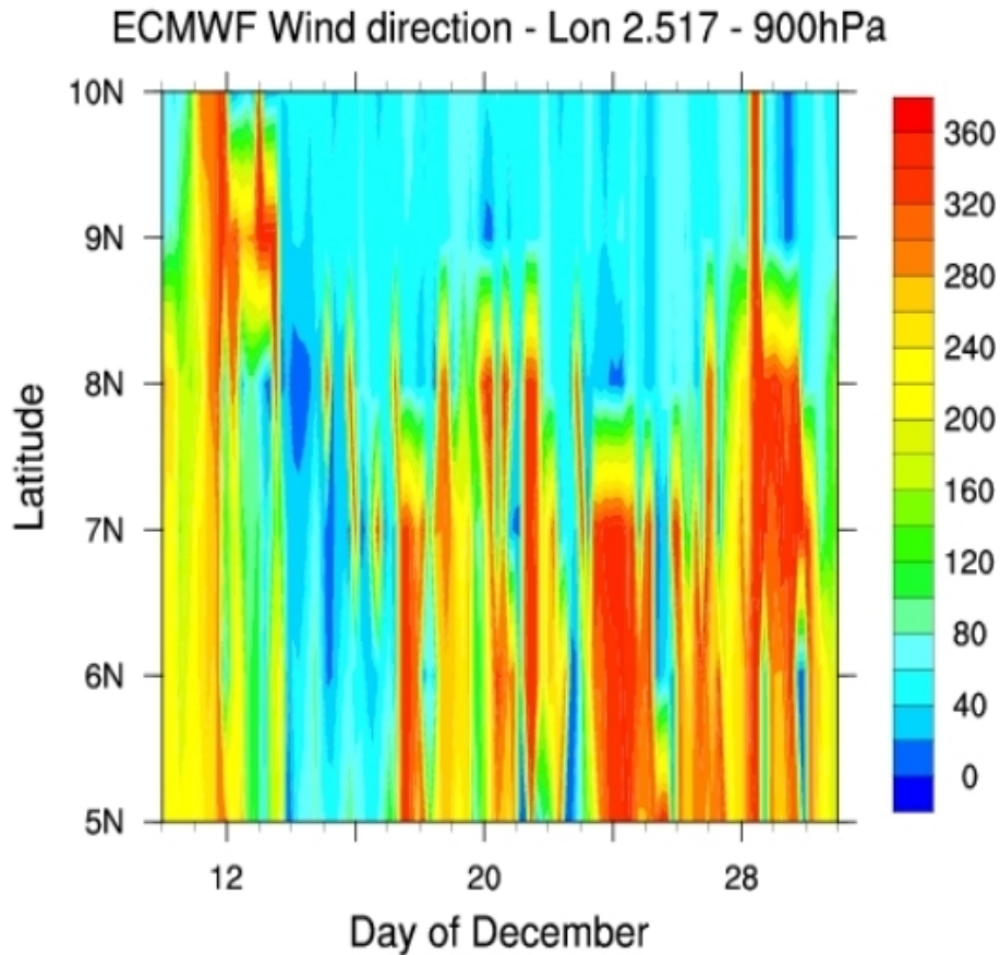
Fig. 4. Hovmoeller diagram of the wind direction (degrees) at 900 hPa at the longitude of Cotonou (2.5° E) from ECMWF analysis.
