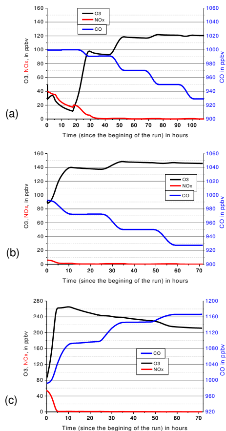
Fig. 7. Time evolution of the ozone (black), CO (blue) and NO x (red) concentrations simulated by the Master Mechansim box model for the three simulations: (a) biomass burning, (b) additional Lagos and (c) additional petrochemical accident.
