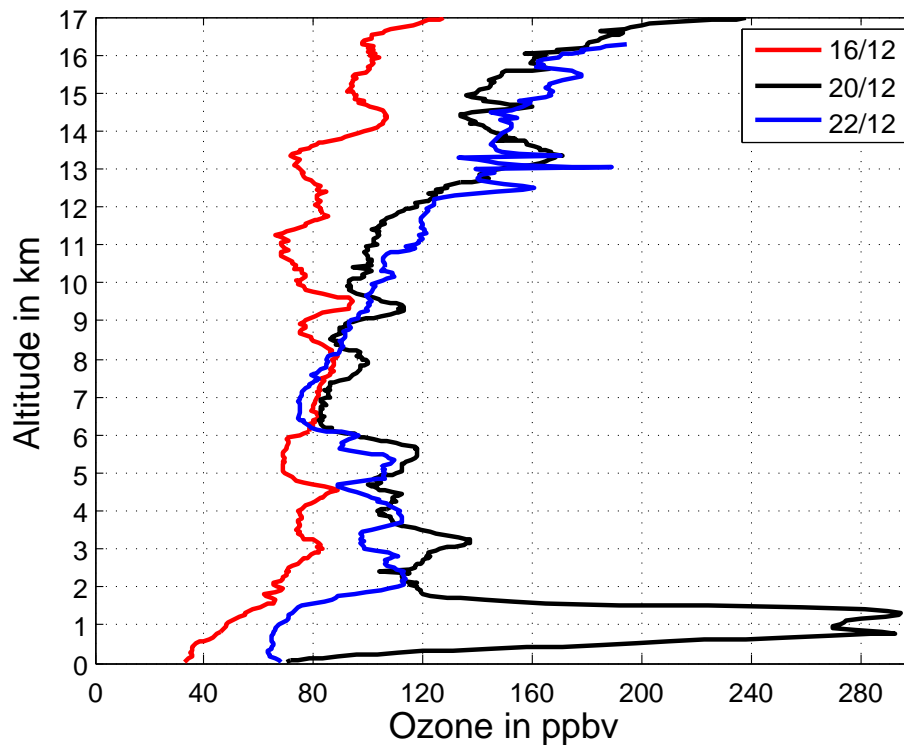
Fig. 1. Vertical profiles of ozone up to 17 km over Cotonou provided by the three soundings performed in December 2005: on 16 (red), 20 (black) and 22 (blue).
