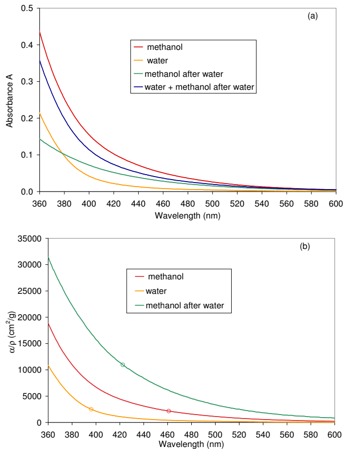
Fig. 5. (a) Spectra of absorbance and (b) absorption per mass for sample oak.M.270, of methanol extract, water extract, and methanol extract after water extraction.
