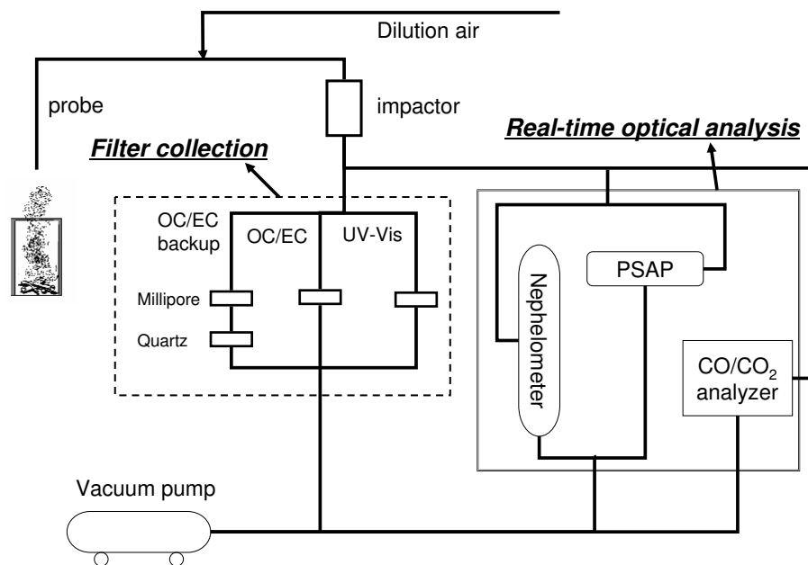
Fig. 1. Schematic of sampling system.
