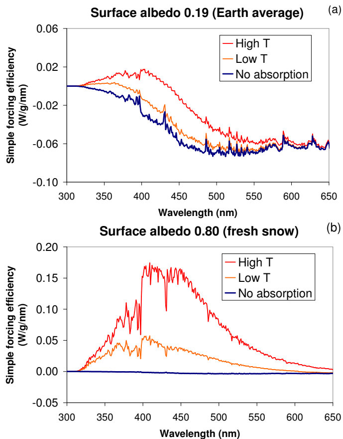
Fig. 11. Simple forcing efficiency of particles above an average albedo (a) and snow (b) . Integrated forcing for average and snow albedo, respectively: High T, -12 and 23 W/g Low T, -16 and 6.3 W/g; no absorption: -18 and -0.92 W/g.
