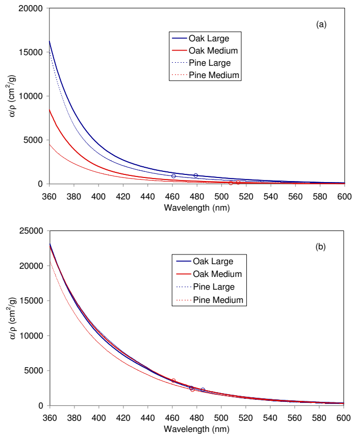
Fig. 7. Effect of wood type and size on absorption per mass ( \alpha/\rho ) of methanol extracts. (a) 210°C, (b) 360°C (note the scale change for two figures).
