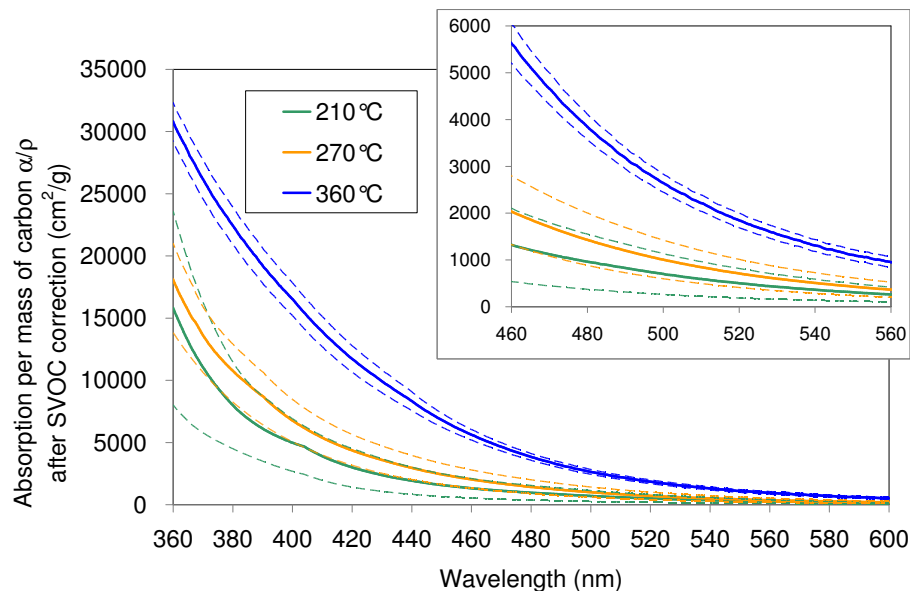
Fig. 10. Averaged absorption per mass of carbon \alpha/\rho after correction for SVOC. Dashed lines with the same color indicate upper and lower range.
