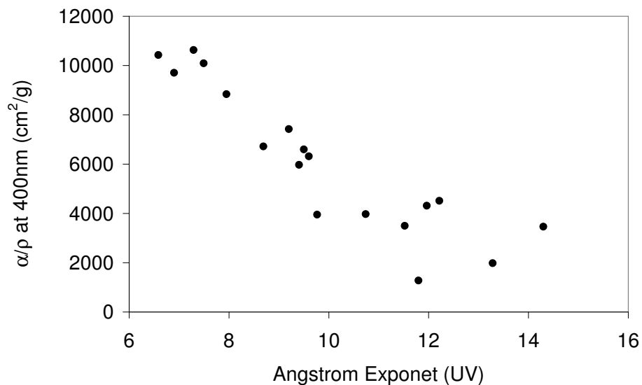
Fig. 8. \text{\AA}_{\text{ap}} at UV range vs. \alpha/p at 400 nm.
