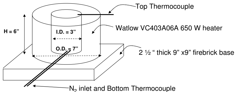
Fig. 2. Detailed Diagram of Combustor.
