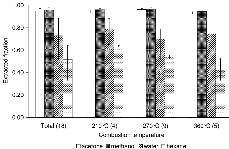
Fig. 3. Extracted fraction of OC by different solvents. The numbers in the parentheses indicate the number of samples analyzed at each temperature.
