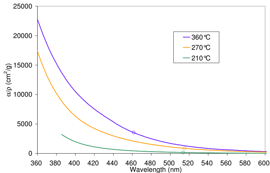
Fig. 6. Generation temperature dependence of absorption per mass ( \alpha/\rho ) of methanol extracts (medium size oak wood).
