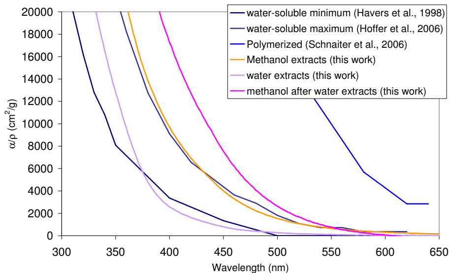
Fig. 9. Comparison with other results, generation condition: oak_L_360.
