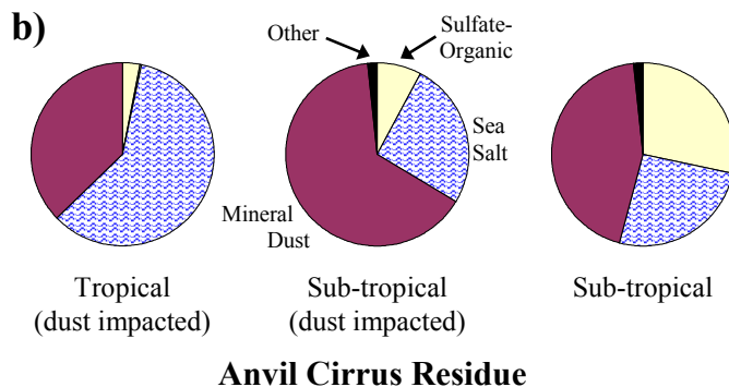
Fig. 4. Aerosol types in the tropical tropopause region. (a) Subvisible cirrus residues from the 2 February SVC layer at 16.0–17.4 km are compared to unfrozen aerosols. (b) Residues from several anvil cirrus encounters at lower altitudes, 12–14 km. Anvil ice crystal residues have different compositions than tropopause level cirrus and showed disproportionately high mineral dust and sea salt compared to the background aerosol (not shown, similar to a). Subtropical data are reproduced from Cziczo et al. (2004b). See Table 1 for statistics.
