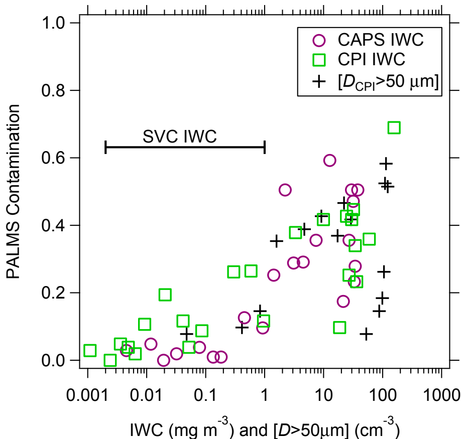
Fig. 2. Fraction of cloud residue particles showing contamination signatures for all ice clouds above 6 km. Low ice water content (IWC), and ultimately, low concentrations of ice crystals >50 µm limited shattering artifacts within SVC. WB-57 aircraft speeds were 150 m/s at 10 km altitude, increasing to 200 m/s above 15 km.
