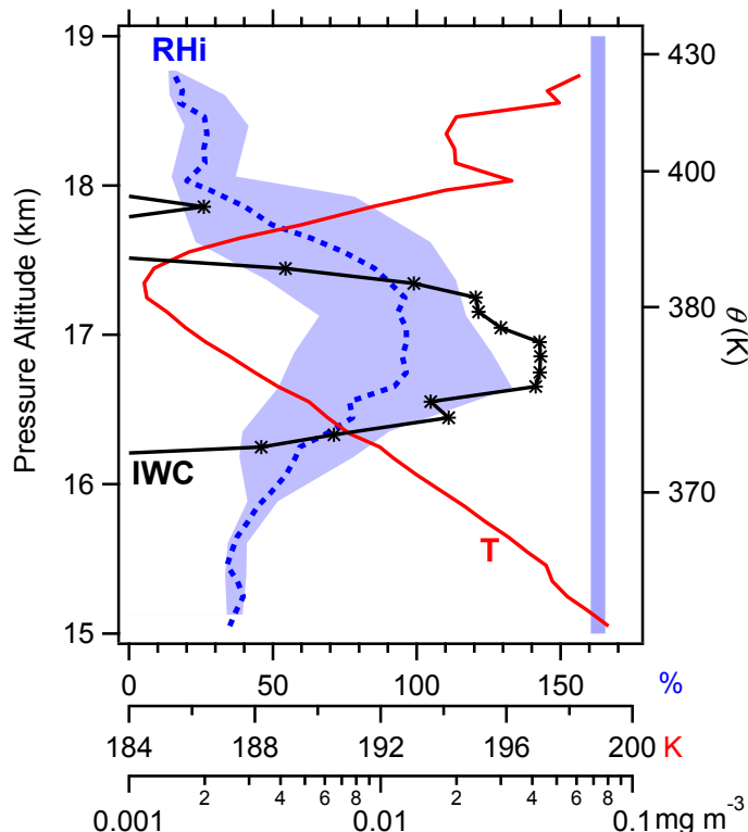
Fig. 3. Average vertical profile for an extensive subvisible cirrus system encountered by the aircraft on 2 February 2006. SVC ice water content (IWC, starred line) is calculated from both 2D-S channels. Mean RH i (dashed line) is calculated from JLH water vapor using Murphy and Koop (2005), and the shaded region encompasses the full range of measurements. The homogeneous freezing limit (vertical bar) is shown for soluble 300 nm aerosols (Koop et al., 2000). T and RH i data include regions both within and outside cloud.
