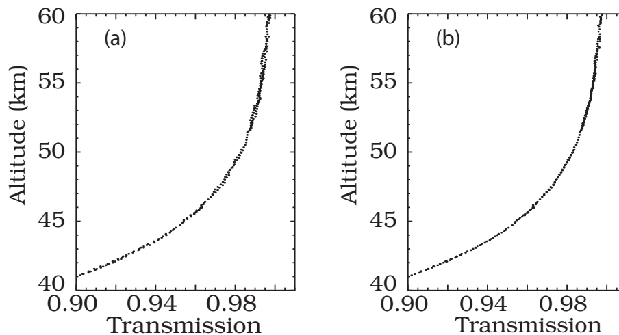
Fig. 8. Unbinned transmission is shown in the ozone channel (600 nm) between 40 and 60 km after all other transmission processing. In frame (a), no time dependent I-zero correction was made, while data in frame (b) employs the correction as described in Sect. 3.4. The measurement event depicted here occurred on 1 May 2005 at (36.0° N, 58.8° E).
