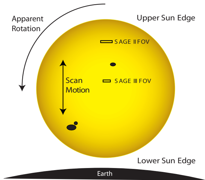
Fig. 2. A schematic of how the Sun appears to a SAGE instrument including to-scale representations of the field of view (FOV) for SAGE II and SAGE III. The scan direction is centered along the center axis of the Sun normal to the Earth's surface. Dark circles represent sunspots. In this coordinate system, the Sun appears to rotate such that solar features may either rotate into or out of the instrument's FOV.
