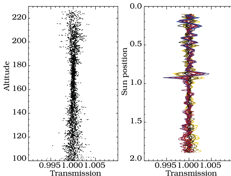
Fig. 3. Transmission is shown as a function of altitude (left) and apparent position on the face of the sun (right) for a SAGE II measurement event on 21 July 2000. Measurements from the 386 nm wavelength channel are displayed. The vertical axis in the right panel is position along a vertical line bisecting the solar image, represented in arbitrary units from 0 (top of the sun as seen from the spacecraft) to 2 (bottom of sun). The data shown here are for slant paths entirely above the atmosphere (minimum altitude is 100 km). At position approximately 1.1, there is a signature of a large sunspot, which has not been filtered for this demonstration. Variations in transmission away from unity are due to errors in the limb-darkening curve used for calibration, as well as instrument noise. Calibration errors are correlated from scan to scan and are hypothesized to be due to rotation of the scan plane.
