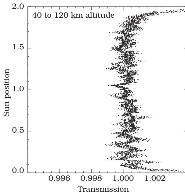
Fig. 5. Simulated transmissions are shown as a function of position on the face of the sun. The biases in transmission near the edges of the sun result from faulty edge matching, due to the image of the sun not being round. Since all scan data are generated from the same image, deviations from one (except at the edges) are indicative of the amount of variation that can be expected from rotation of the scan plane alone.
