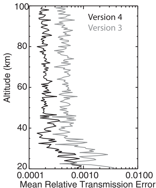
Fig. 9. Mean short wavelength transmission error for a single event in October 2003 for Version 4 (black) and Version 3 (grey). For this event, the uncertainty is reduced by approximately 50%.
