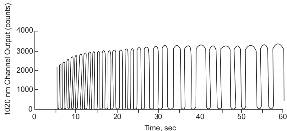
Fig. 1. The time history of sunrise SAGE event at a single wavelength (1020 nm in this example). The sinusoid-like structure is due to the vertical scanning across and off the Sun. The alternating narrow and wide “waves” are the result of scanning either with or against the effective direction of the Sun’s motion. For sunrise events, the narrow waves are downward (toward the Earth) scans whereas the wide waves are upward scans.
