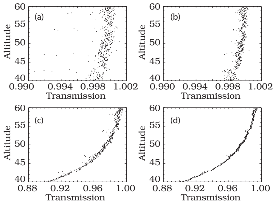
Fig. 7. Unbinned transmission is shown as a function of altitude between 40 and 60 km for SAGE II channels 1 at 1020 nm and channel 7. Frames (a) and (b) show uncorrected and corrected channel 1 while frames (c) and (d) show uncorrected and corrected channel 7. Left and right panels depict transmission before and after the correction, respectively. The specific SAGE II measurement event shown here occurred on 1 May 1989.
