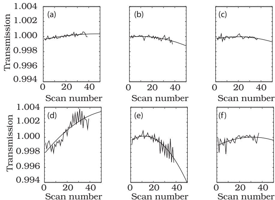
Fig. 6. Transmission, calculated by normalizing the SAGE II measurements against the exoatmospheric measurements, and then re-normalized for this experiment by dividing by an average transmission profile, is shown as a function of scan number. The measurement event shown here occurred on 1 May 1989. The panels show the transmission within a narrow range of Sun position for channels 1 and 7. Specifically, frames (a)–(c) show channel 1 (1020 nm) for Sun positions 0.5, 1.0, and 1.5, respectively while frames (d) through (f) show channel 7 (386 nm) for the same Sun positions. Broad scale variation, highlighted by overlaid quadratic fits, is attributed to apparent changes in the solar structure (granulation, solar faculae) due to movement of the scan track over the course of the event.
