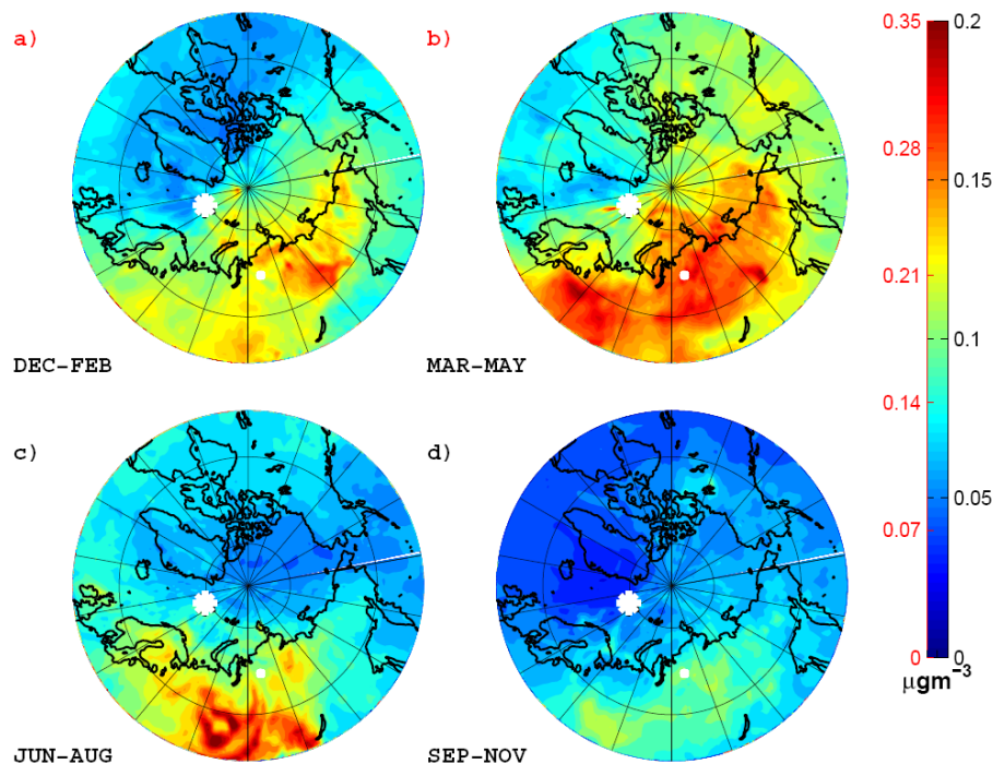
Fig. A4. The complete set of calculated emission sensitivity fields, each weighted with the associated NSS sulphate concentrations measured at Zepplin during the years 2000–2006, for December–February (upper left), March–May (upper right), June–August (lower left) and September–November (lower right). The left colour bar applies to (a) and (b), right scale applies to (c) and (d). The location of the Zepplin station is marked by a large white asterisk, and a small white dot marks the location of Norilsk.
