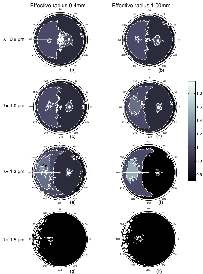
Fig. 9. Anisotropy factor R(\theta_v, \phi) computed with SnowRAT (Picard et al., 2008) for cylinders with random orientation. Incident angle is 30^\circ .
