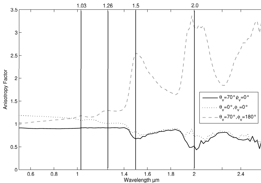
Fig. 3. S3 Anisotropy factor, R(\lambda) for different viewing angles in the principal plane. Incident angle is 30^\circ . Vertical lines are the same as in Fig. 2.
