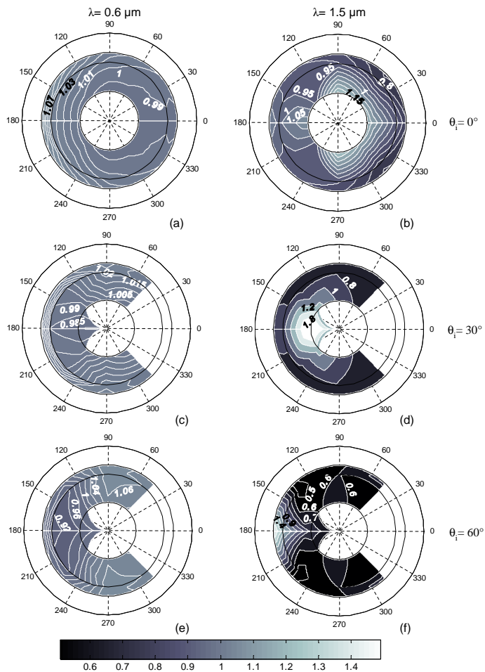
Fig. 5. Ratio of the anisotropy factor R between samples S1 and S3 \left(\frac{R(S1)}{R(S3)}\right) at 0, 30 and 60° incident beam and for several wavelengths.
