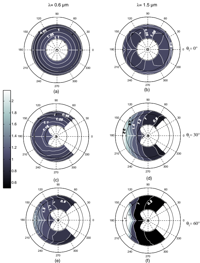
Fig. 4. S3 Anisotropy factor, R(\theta_v, \phi) , at 0.6 and 1.5 \mu\text{m} for zenith incident angles 0^\circ , 30^\circ and 60^\circ . The polar angle corresponds to the relative azimuth, \phi , between the viewing and the incident azimuth and the polar radius to the viewing angle, \theta_v . The incident beam comes from the right and the forward direction is toward left. The three circles inside each plot represent viewing zenith angles of 30^\circ , 60^\circ and 70^\circ . The crosses show the measurements used to generate the isolines.
