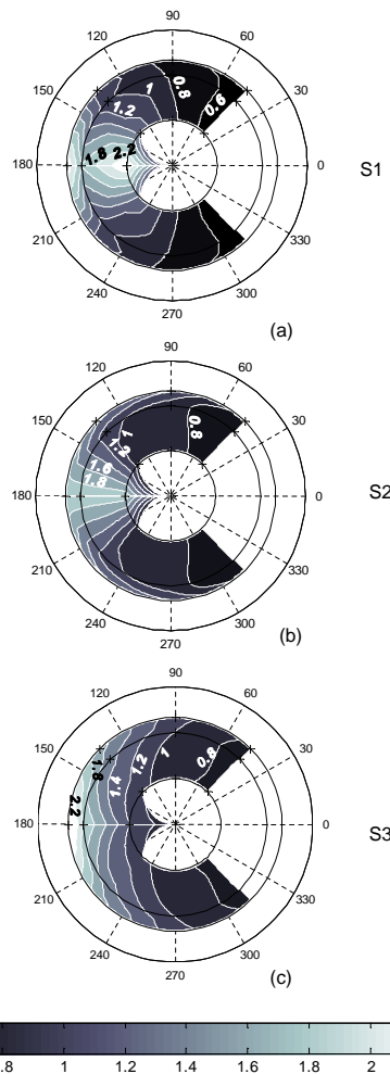
Fig. 6. Anisotropy factor R(\theta_v, \phi) at 1.5 \mu\text{m} and \theta_i = 30^\circ for three snow samples. (a) S1; (b) S2; (c) S3.
