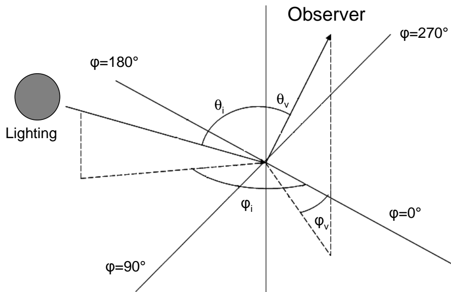
Fig. 1. Lighting and viewing configuration.
