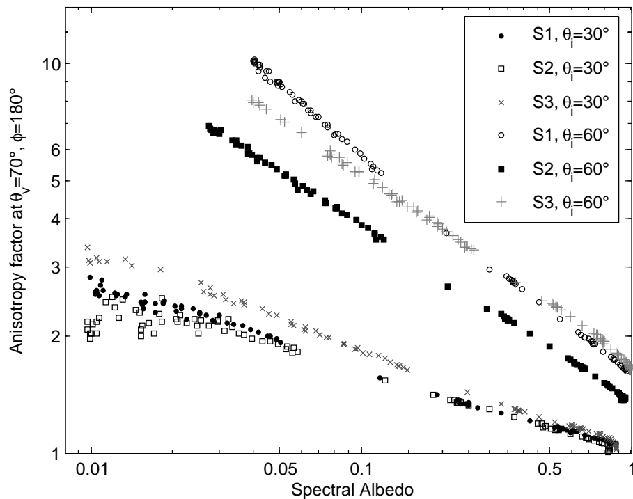
Fig. 7. Anisotropy factor R(\theta_v=70^\circ, \phi=180^\circ) versus spectral albedo (log-log plot) for the three samples and two incident angles ( 30^\circ and 60^\circ ).
