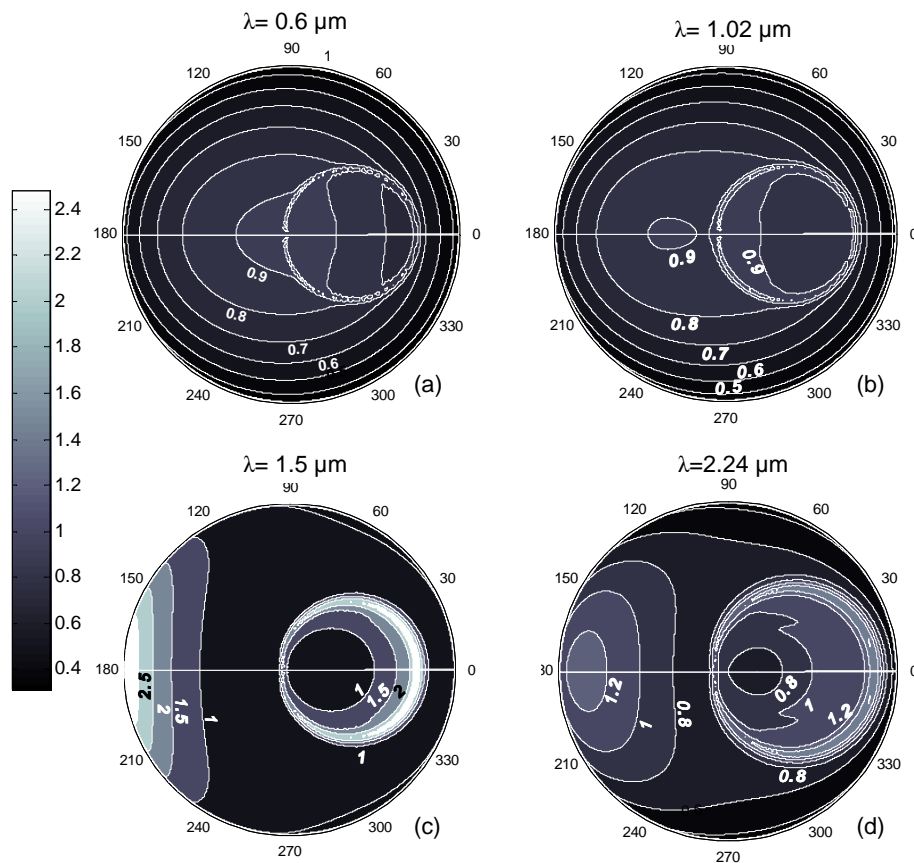
Fig. 8. Anisotropy factor R(\theta_v, \phi) (Mishchenko model, Mishchenko et al., 1999) for spheres with power law distribution of size. Incident angle is 30^\circ . Effective radius is 0.1 \text{ mm} and effective variance of grain size distribution is 0.2 \text{ }\mu\text{m} .
