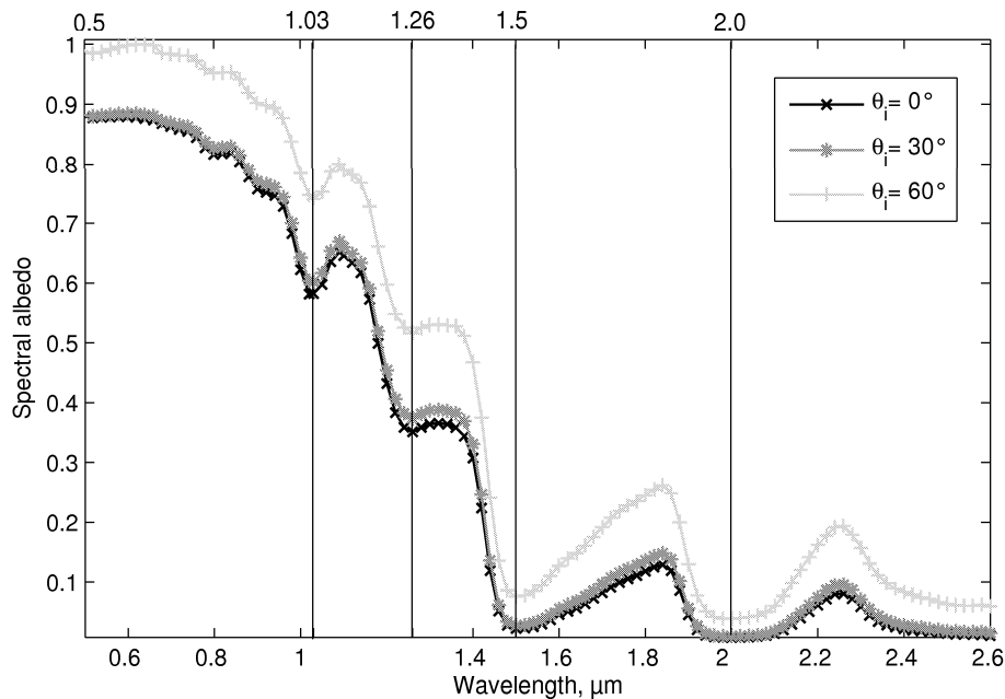
Fig. 2. S3 spectral albedo \alpha(\lambda, \theta_i) calculated from BRDF measurements for three incident zenith angles. Vertical lines are located at spectral albedo minima.
