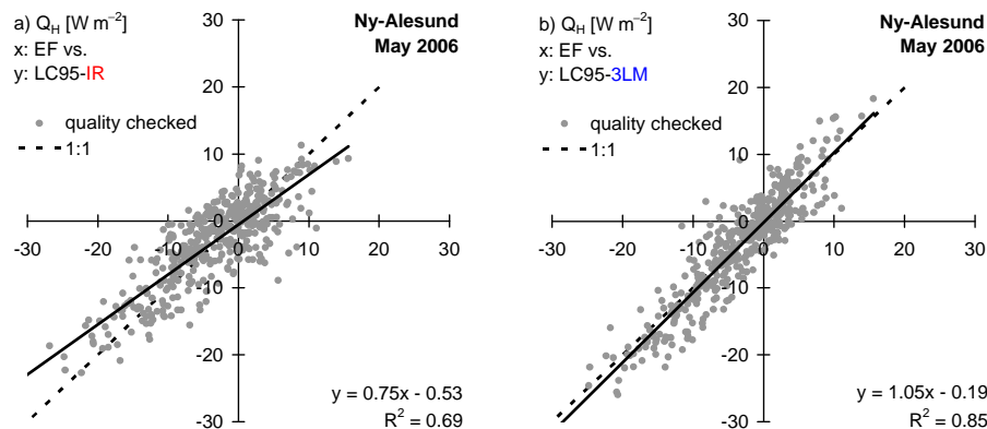
Fig. 3. Linear correlation of the sensible heat flux Q_H [ \text{W m}^{-2} ] measured with a sonic-anemometer applying the eddy-covariance method (EF), and calculated with the LC95-parameterization (Launiainen and Cheng, 1995) over a snow surface using (a) the IR-derived (IR) and (b) the 3-layer-model-extrapolated (3LM) surface temperature T_{(0)} as input. Quality checked values, elimination of the periods with snowdrift or precipitation effects on the sonic-anemometer, 7 May to 19 May 2006. Ny-Ålesund (Svalbard), ARCTEX-2006.
