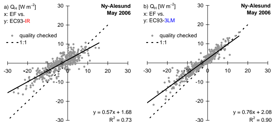
Fig. 4. Linear correlation of the sensible heat flux Q_H [ \text{W m}^{-2} ] measured with a sonic anemometer applying the eddy-covariance method (EF), and calculated with the EC93-parameterization (Ebert and Curry, 1993) over a snow surface using (a) the IR-derived (IR) and (b) the 3-layer-model-extrapolated (3LM) surface temperature T_{(0)} as input. Quality checked values, elimination of the periods with snowdrift or precipitation effects on the sonic-anemometer, 7 May to 19 May 2006. Ny-Ålesund (Svalbard), ARCTEX-2006.
