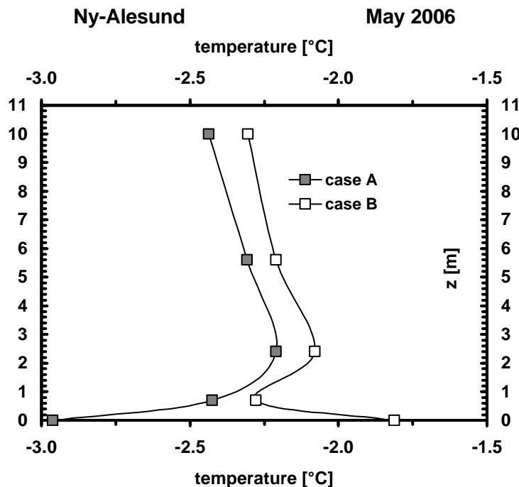
Fig. 1. Vertical profiles of temperature for two separate cases A and B between 7 May and 19 May 2006, as observed at the UBT meteorological gradient tower MT2. Case A reflects strong surface cooling and a sharp thermocline inversion within just 1 or 2 m above ground mostly occurring between 5 and 8 o'clock or 17 and 22 o'clock CET. Case B occurs mostly around noon (9 to 16 CET) indicating a disturbed profile caused by surface warming. Ny-Ålesund (Svalbard), ARCTEX-2006 campaign.
