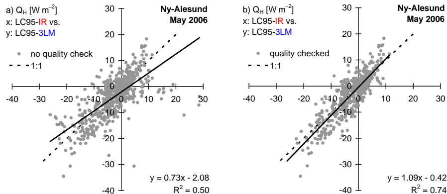
Fig. 2. Linear correlation between sensible heat flux Q_H [ \text{W m}^{-2} ] calculated with the LC95-parameterization (Launiainen and Cheng, 1995) using the IR-derived (IR) or the 3-layer-model-extrapolated (3LM) surface temperature T_{(0)} as input: (a) unfiltered values, (b) quality checked values, elimination of the periods with snowdrift or precipitation effects on the sonic anemometer from 7 May to 19 May 2006. Ny-Ålesund (Svalbard), ARCTEX-2006 campaign.
