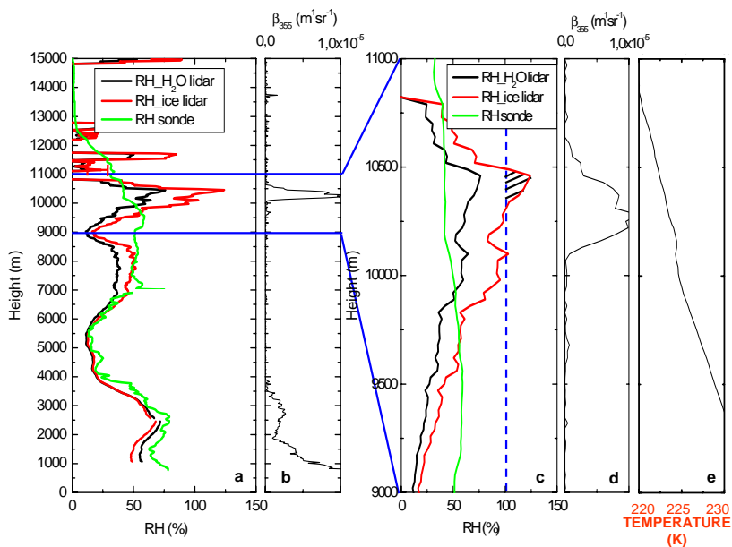
Fig. 5. 10 min average profiles for the time interval 19:05–19:15 UTC: (a) lidar profiles of RH (black line) and RHI (red line) and radionsonde profile of RH (green line); (b) particle backscatter profile at 355 nm; (c) magnification of panel (a) in the vertical region the 9–11 km (a.s.l.); (d) magnification of panel (b) in the vertical region the 9–11 km; (e) lidar profile of atmospheric temperature in the vertical region the 9–11 km.
