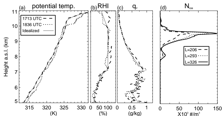
Fig. 9. Panel (a, b, c): The atmospheric profiles measured at 17:13 (dashed) and 18:36 (dotted) UTC versus altitude a.s.l. The gray curves indicate the idealized profiles used as the initial conditions for the 1-D simulations. Panel (d): The profiles of ice number concentration, N_{ice} , retrieved using the lidar backscatter profile measured at 17:32 UTC. In the calculation, the modified gamma distribution is used, is set to 7 and three values of L (326, 293, 206 \text{cm}^{-1} ) are tested.
