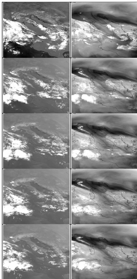
Fig. 1. Sequence of images from MSG SEVIRI: channel IR108 (centered at 10.8\ \mu\text{m} ) on left column and channel WV62 (centered at 6.25\ \mu\text{m} ) on the right column. The timing (from top to bottom) is: 13:12:44, 17:12:45, 18:42:44, 19:42:43 and 21:27:43 UTC).
