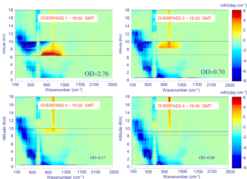
Fig. 7. Spectral cooling/heating rate profiles in correspondence of the 4 Proteus overpasses over BASIL . The time sequence is 1st overpass: upper left, 2nd overpass: upper right, 3rd overpass: lower left and 4th overpass: lower right panel. In the firsts 3 panels the lidar measured cloud optical depths (in the short-wave) are also reported. Altitude in km (from 0 to 18) a.s.l. is reported on Y-axis and wave number (from 100 to 2500) in \text{cm}^{-1} on X-axis. For visual purposes, spectral cooling/heating rates are averaged on a spectral widow of 20 \text{ cm}^{-1} .
