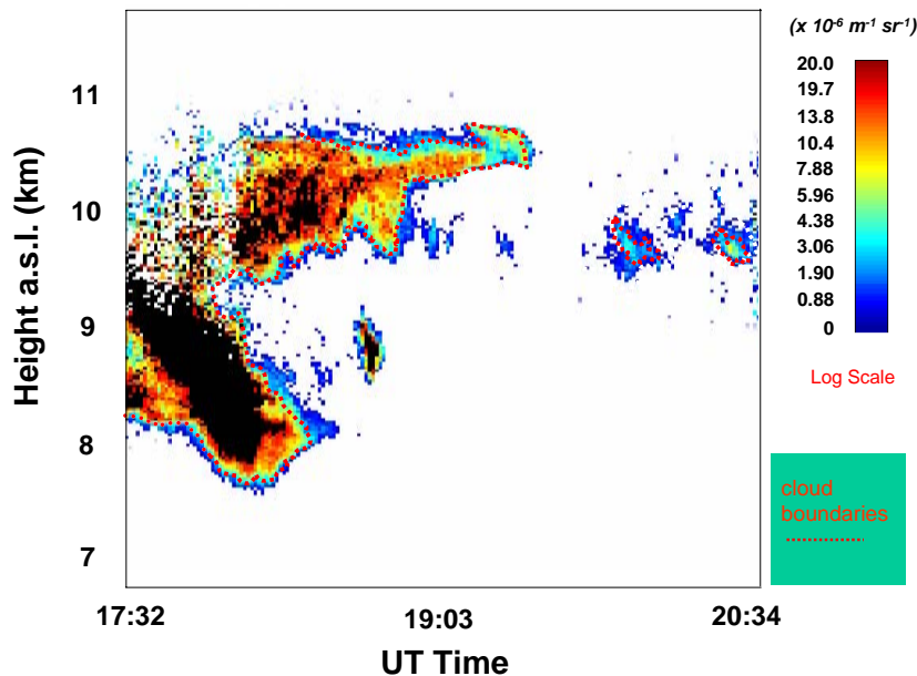
Fig. 2. Time evolution of particle backscattering coefficient at 355 nm from 17:32 to 20:34 UTC on 6 September 2004. Here and in the following figures, height is expressed in km above mean sea level (a.s.l.).
