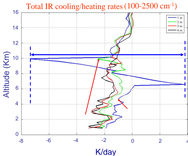
Fig. 8. Vertical profiles of total infrared cooling/heating rates in correspondence of the 4 Proteus overpasses over BASIL .
