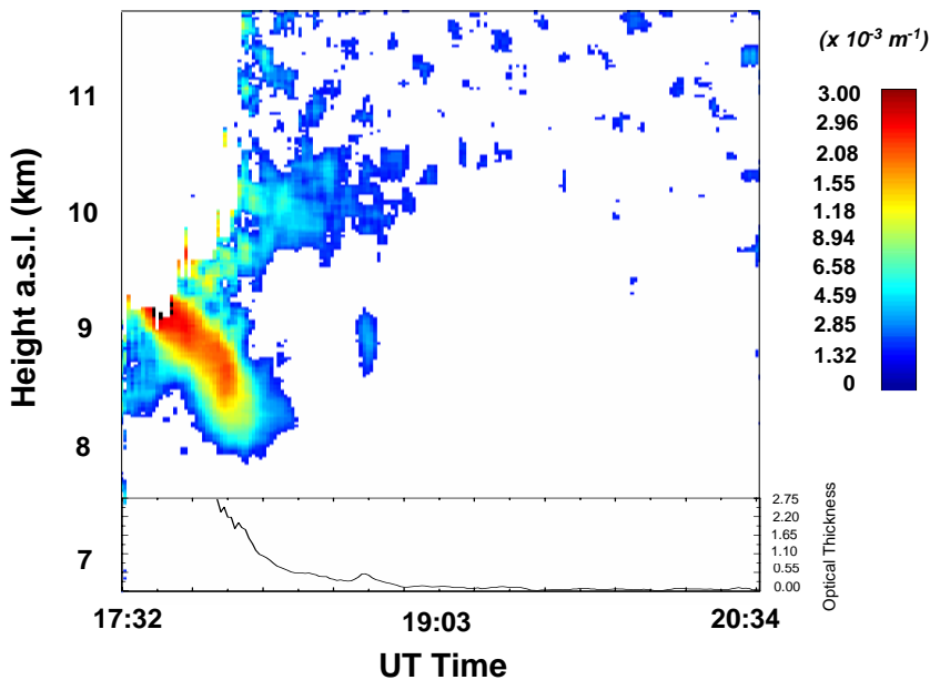
Fig. 3. Time evolution of the particle extinction coefficient (same time-frame as Fig. 2). The lower panel shows the evolution with time of total cloud optical thickness.
