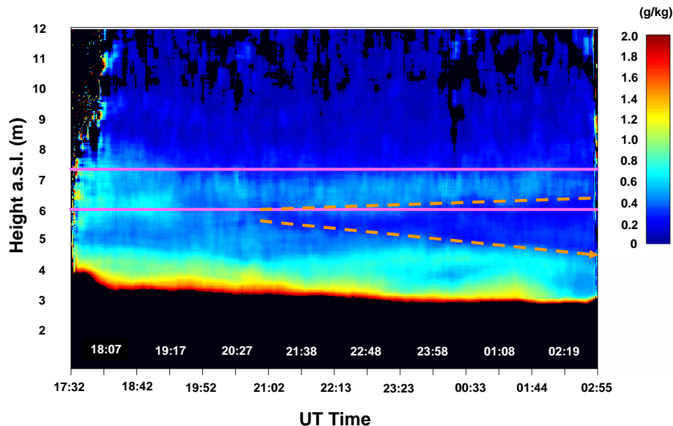
Fig. 6. Time evolution of water vapour mixing ratio over the time period of approx. 9.5 h from 17:32 UTC on 6 September 2004 to 02:55 UTC on 7 September 2004. A humid layer is present between 6 and 7.5 km a.s.l. (included between the two horizontal violet lines).
