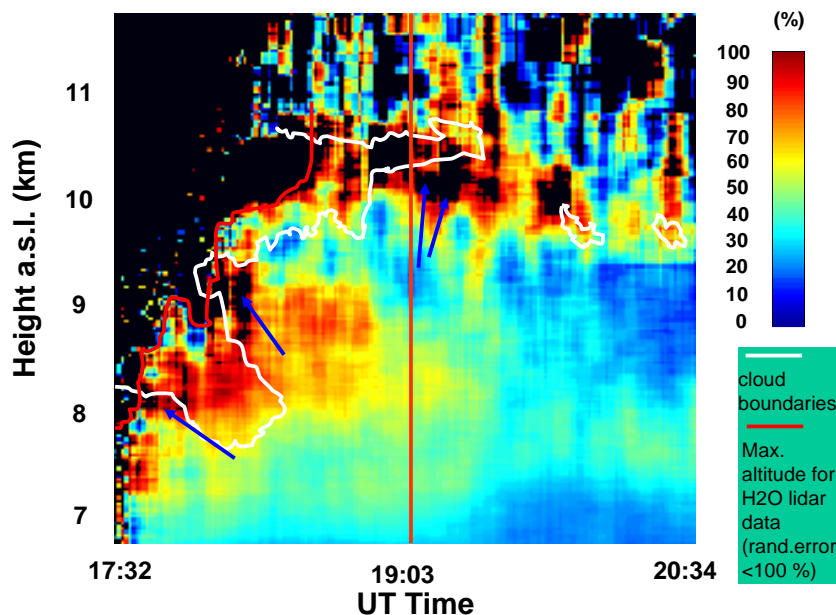
Fig. 4. Time evolution of RH on 6 September 2004. White lines represent cloud boundaries, while red lines represent the maximum reached altitude for water vapour lidar measurements. The red vertical line identifies the 10 min average profiles (19:05–19:15 UTC) considered in Fig. 5. Large relative humidity values beneath the clouds (blue arrows) are associated with upper tropospheric humidification caused by the sublimation of precipitating ice crystals.
