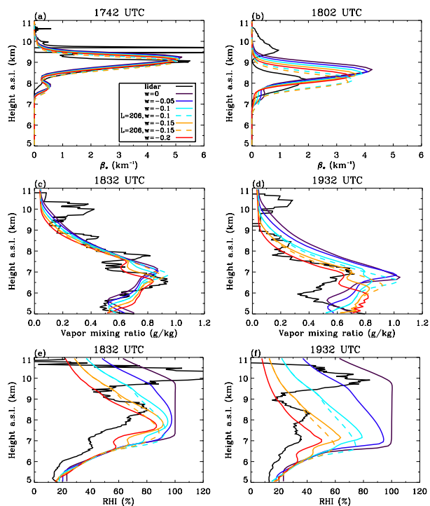
Fig. 10. Lidar measurements vs 1-D simulations at selected times. Panels (a, b) are the profiles of the volume extinction coefficient; (c, d) are the profiles of the vapor mixing ratio, and (e, f) are the RHI. In the simulations, L is 326 \text{ cm}^{-1} except where otherwise noted.
