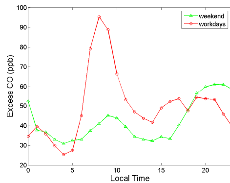
Fig. 7. Diurnal variation of excess hydrogen (a) and carbon monoxide (b) mixing ratios during workdays and weekends in September–October 2007.
