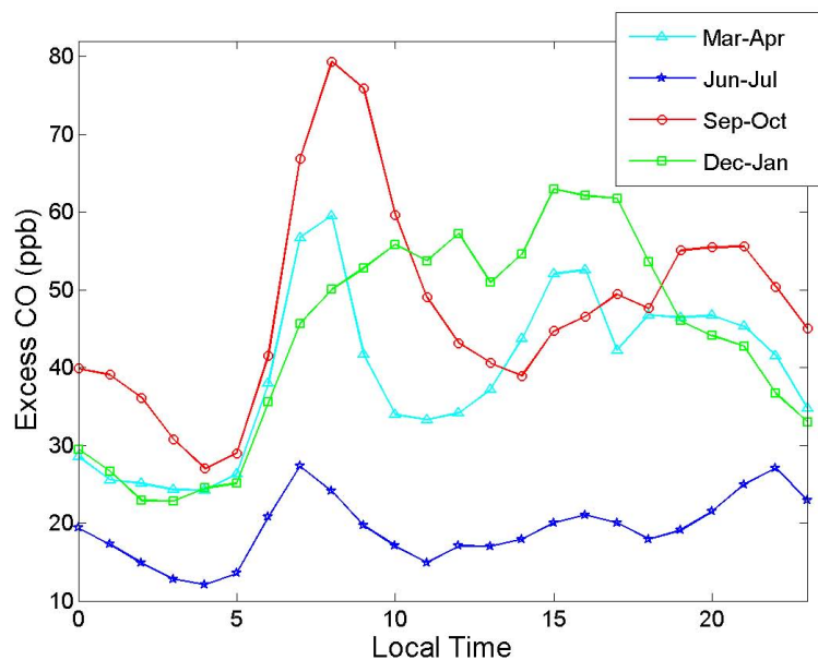
Fig. 6. Diurnal variation of excess carbon monoxide mixing ratios at Kumpula site in Helsinki during the four seasons.
