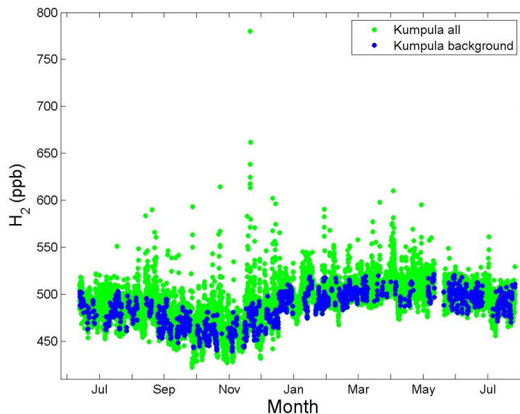
Fig. 2. Hydrogen mixing ratios at Kumpula site in Helsinki. All refers to all hourly mean values and background to selected hourly values.
