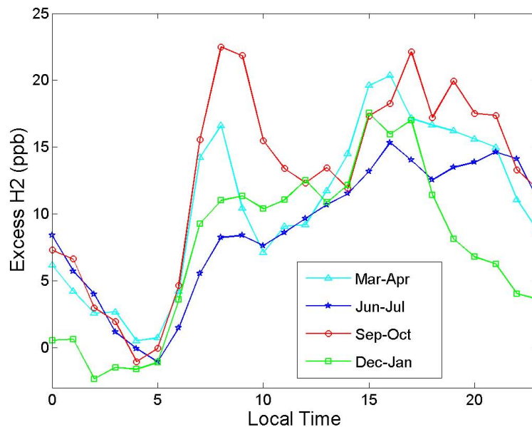
Fig. 5. Diurnal variation of excess hydrogen mixing ratios at Kumpula site in Helsinki during the four seasons.
