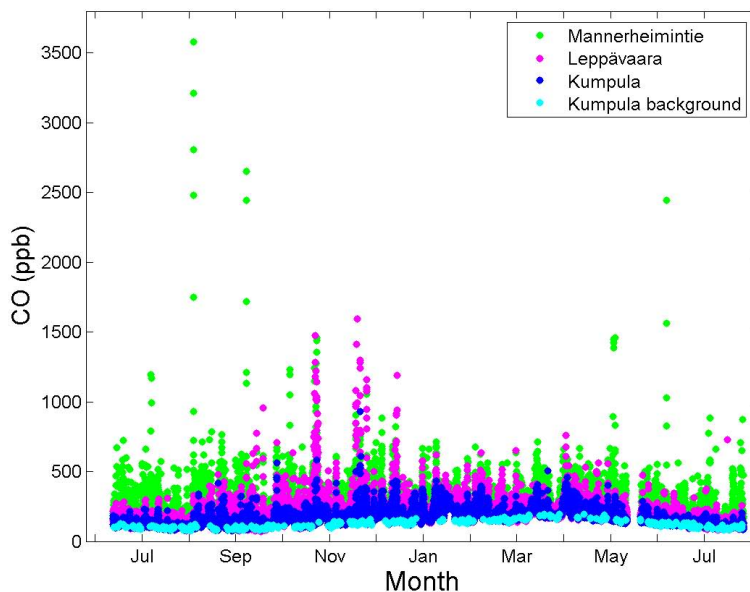
Fig. 3. Hourly means of carbon monoxide mixing ratios at three sites in Helsinki region. Kumpula background refers to selected hourly values. Mannerheimintie and Leppävaara data provided by YTV Helsinki Metropolitan Area Council.
