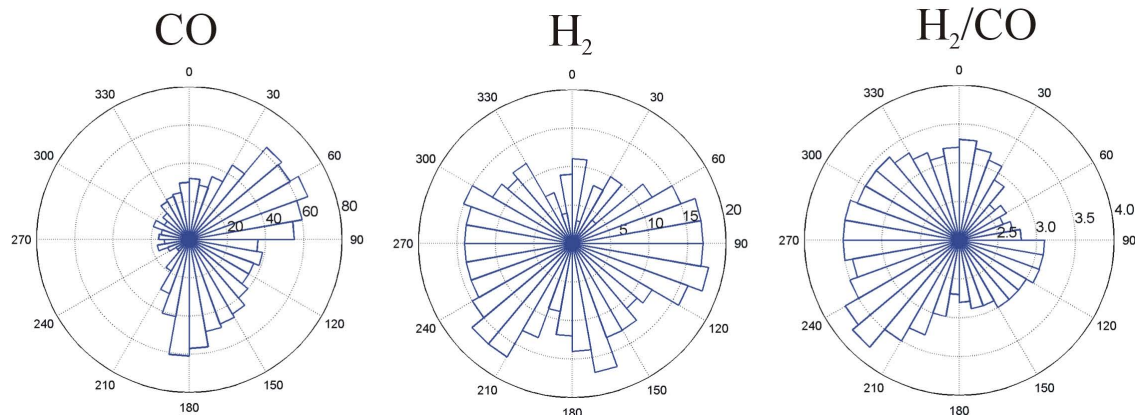
Fig. 4. Hydrogen and carbon monoxide in air masses arriving from the direction indicated by the 360 degree circle. 0 refers to winds arriving from north, and 90 east. The length of each 10 degree sector wedge is indicated by the numerical values inside the circle, either in ppb for CO and H 2 or in ppb (H 2 )/ppb (CO) for H 2 /CO. The value refers to difference between the mean mixing ratio (or H 2 /CO ratio) in current sector and minimum of all 10 degree sectors.
