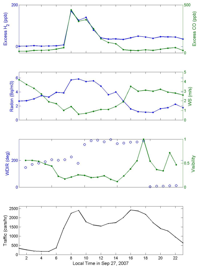
Fig. 8. Excess hydrogen and carbon monoxide mixing ratios, radon activity and weather parameters (wind speed, wind direction, visibility) at Kumpula, site and traffic flow at nearby Hämeentie bridge on 27 September 2007.
