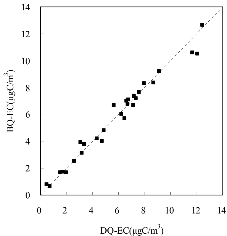
Fig. 3. Comparison of DQ-EC and BQ-EC.
