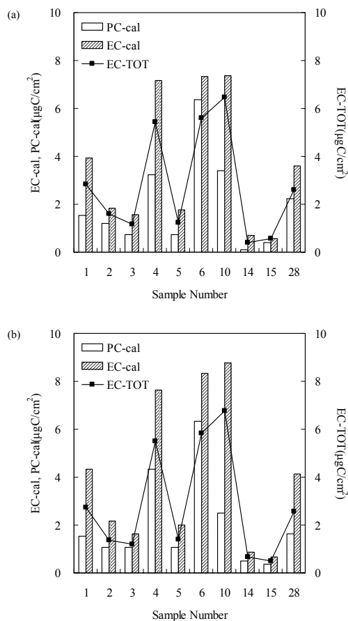
Fig. 7. Comparison of calculated EC concentration (EC-cal) and TOT-split-EC (EC-TOT) for (a) denuded samples, and (b) un-denuded samples. Calculated PC concentration (PC-cal) is also shown.
