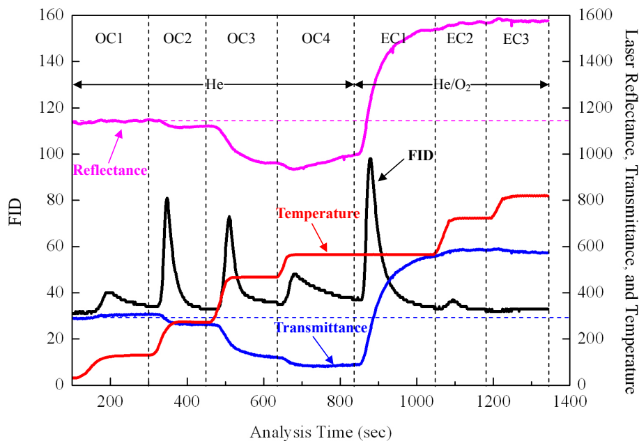
Fig. 2. Example thermogram ( TC=16.27 \mu\text{g C}/\text{cm}^2 ) for IMPROVE-A protocol.
