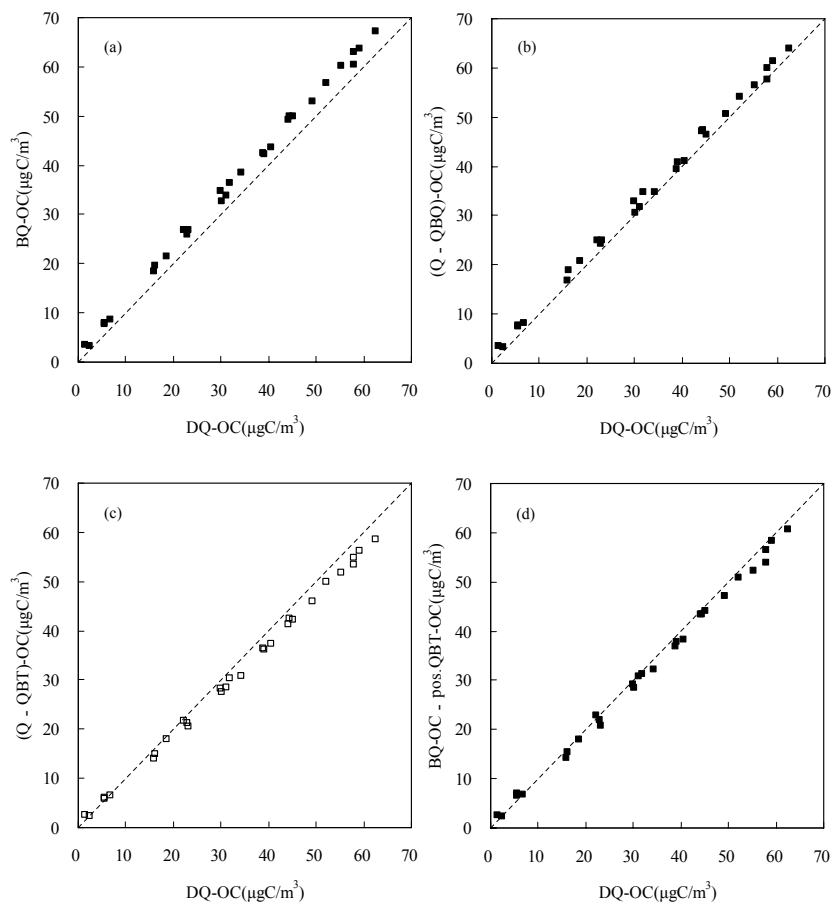
Fig. 5. Comparison of different OC estimations with OC determined by the denuded quartz filter (DQ).
