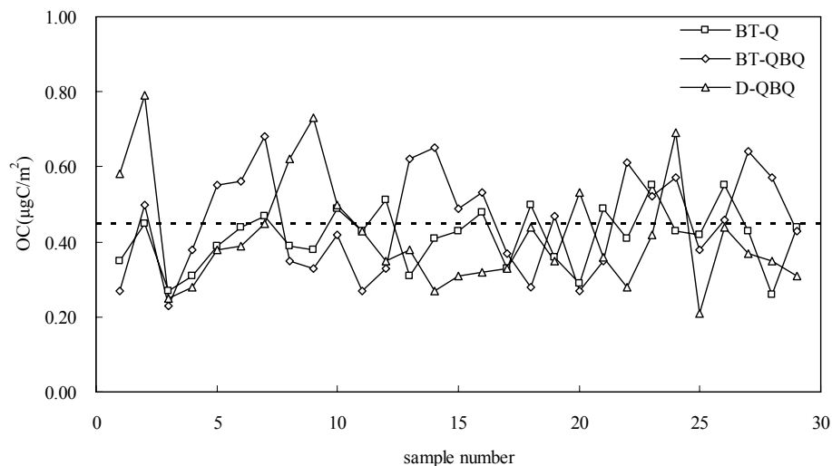
Fig. 4. OC concentrations determined by the front (BT-Q) and backup (BT-QBQ) quartz filter in the breakthrough channel, and by the denuded backup quartz filter (D-QBQ) in channel 1. Dashed line indicates average of blanks. Paired t-test showed that OC determined by BT-Q, BT-QBQ and D-QBQ were not significantly different at a 95% level of confidence; and independent t-test showed they were also not significantly different from the 14 blank values.
