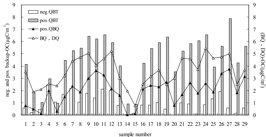
Fig. 6. Negative artifact-contributed QBT-OC (neg. QBT), and different estimations of positive artifact: positive artifact-contributed QBT-OC (pos. QBT), positive artifact-contributed QBQ-OC (pos. QBQ), and the difference between BQ and DQ ((BQ-DQ)-OC).
