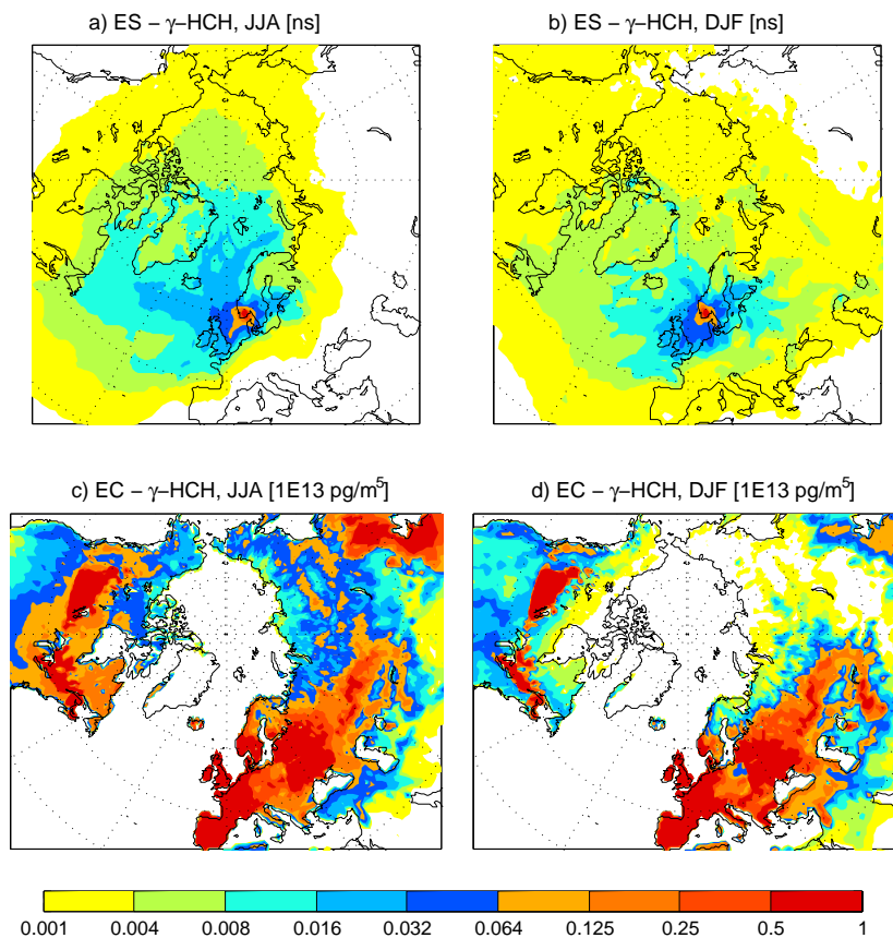
Fig. 11. Same as Fig. 12 but for \gamma -HCH.
