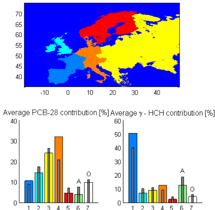
Fig. 12. Contributions (%) of different regions to the total simulated PCB-28 and \gamma -HCH concentrations at Birkenes. The regions used are shown in the upper panel using the same color scheme as in the lower panel, Birkenes station is marked with a white circle on the map. Region 1, Western Europe; 2, UK and Ireland; 3, Eastern Europe; 4, Central Europe; 5, Scandinavia; 6, America (denoted with A); 7, other countries (denoted with O). The grey bars show the contributions when they are weighted by the ratio of the measured/modelled concentrations.
