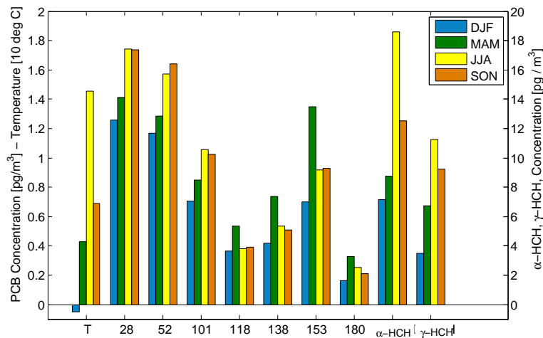
Fig. 3. Temperature ( T ) and concentrations of seven PCB congeners, \alpha -HCH and \gamma -HCH [ \text{pg}/\text{m}^3 ] measured at Birkenes in the period 2004–2007 and averaged over the four seasons DJF (December to February), MAM (March to May), JJA (June to August) and SON (September to November). Note the different scales for PCBs and HCHs.
