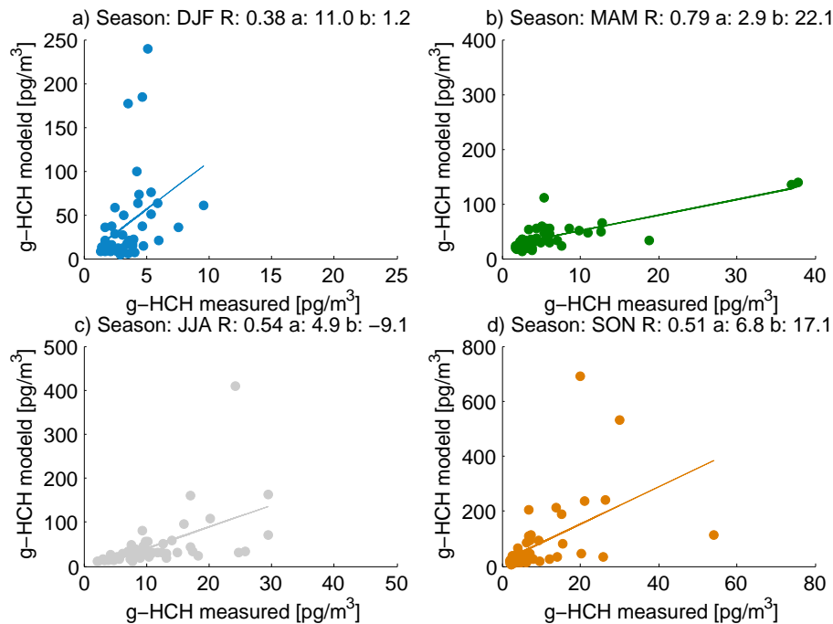
Fig. 9. Same as Fig. 8 but for \gamma -HCH.
