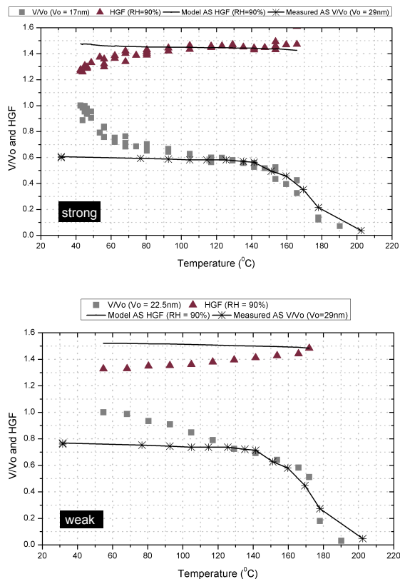
Fig. 9. VHTDMA scans completed during a strong (top) and weak (bottom) nucleation event. V/V_o is volume fraction remaining and HGF (RH=90%) is the growth factor at 90% RH for the atmospheric particles. The solid black lines indicate measured volatility curve of ammonium sulphate (AS) particles normalised to the apparent volume fraction of the more hygroscopic component and theoretical, dry size dependent ammonium sulphate growth factors.
