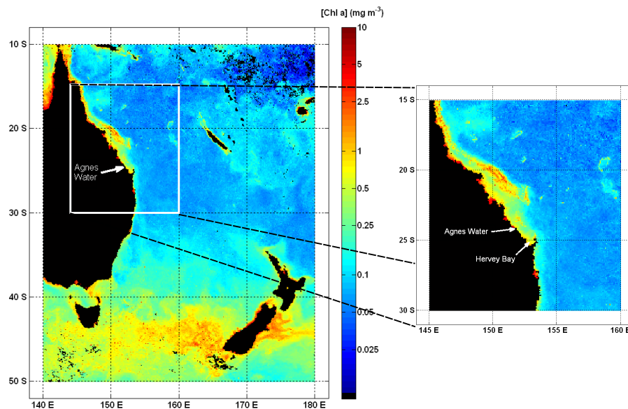
Fig. 10. SeaWiFS derived surface chlorophyll concentrations off the east Australian coast averaged over the month of March 2007.
