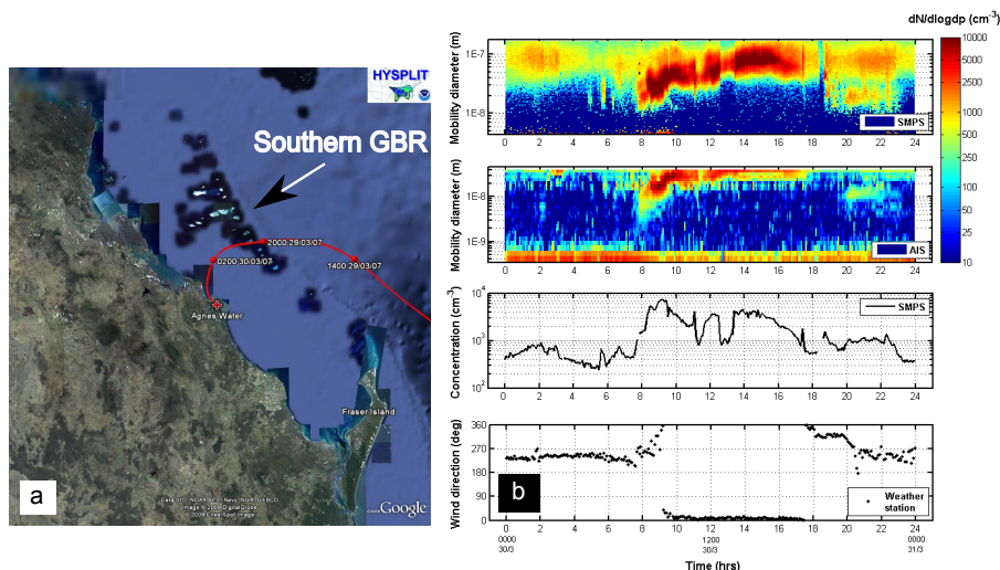
Fig. 5. (a) HYPLIT back trajectory for air mass arriving at Agnes Water at an altitude of 100 m at 08:00 on 30 March 2007. The trajectory clearly shows the air mass crossing the southernmost reefs and islands of the Great Barrier Reef (GBR) on the previous night; (b) Contour plots of the AIS and SMPS data plus time series of particle concentration ( 4 < d < 165 nm) and wind direction for 30 March 2007. Legends indicate the instrument used to measure each data set.
