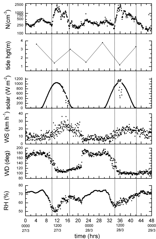
Fig. 6. Time series of particle concentration ( 4 < d < 165 nm), N ( \text{cm}^{-3} ); tide height at Agnes Water, tide hgt (m); solar intensity, solar ( \text{W m}^{-2} ); wind speed, WS ( \text{km h}^{-1} ); wind direction from true north, WD (deg); and relative humidity, RH (%) for 27 and 28 March 2007. Dashed lines indicate the occurrence of 2 strong nucleation events.
