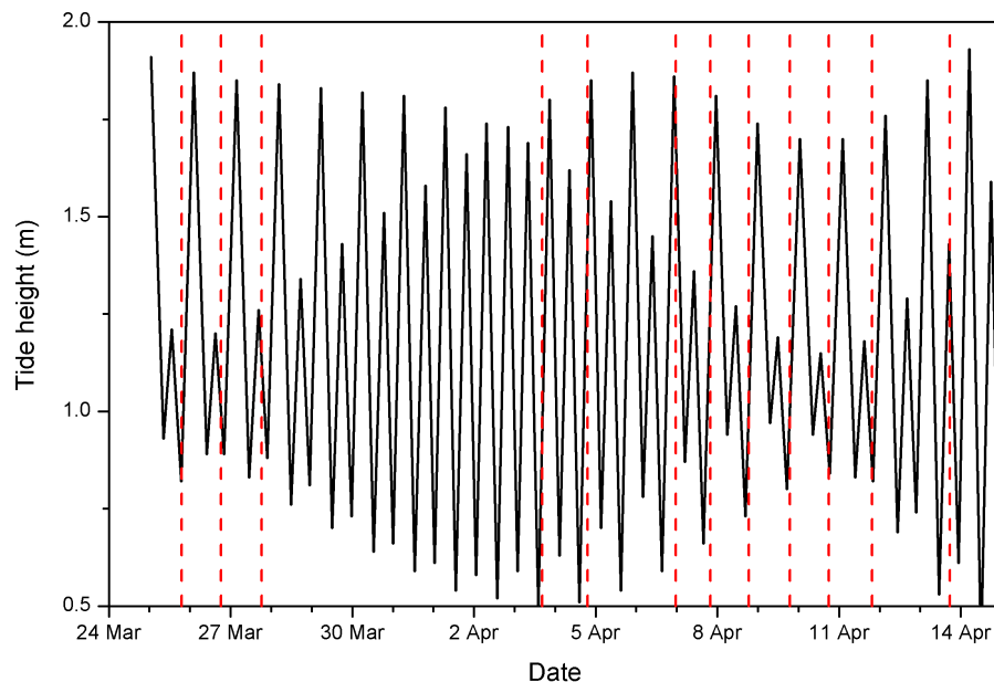
Fig. 8. Tidal height at Fraser Island, a coastal area \sim 15 km upwind from the Agnes Water measurement site. Red dashed lines indicate the times when air masses that contained nucleation mode particles crossed this coastal region.
