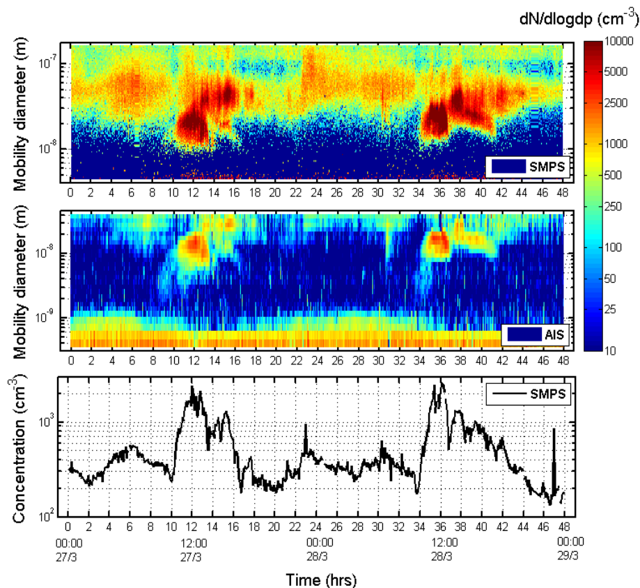
Fig. 4. Contour plots of the AIS and SMPS data and a time series of particle concentration ( 4 < d < 165 nm) for 27 and 28 March 2007. Legends indicate the instrument that measured the data in each graph. AIS data shown is for negative ions, the graph for positive ions looks very similar.
