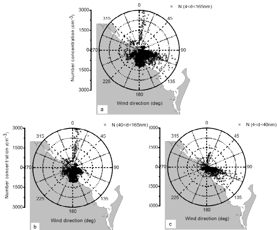
Fig. 2. Polar plots of number concentration against wind direction for particles in the size range (a) 4–165 nm, (b) 40–165 nm and (c) 4–40 nm.
