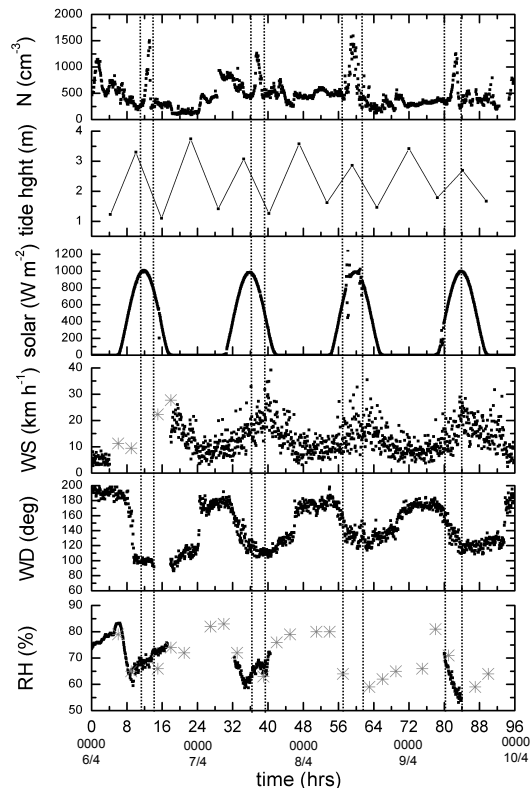
Fig. 7. Time series of particle concentration ( 4 < d < 165 \text{ nm} ), N ( \text{cm}^{-3} ); tide height at Agnes Water, tide hgt (m); solar intensity, solar ( \text{W m}^{-2} ); wind speed, WS ( \text{km h}^{-1} ); wind direction from true north, WD (deg); and relative humidity, RH (%) for 06 to 09 April 2007. Dashed lines indicate the occurrence of 4 weak nucleation events. Grey asterisks represent data collected from a nearby (Town of 1770) Australian Bureau of Meteorology weather station.
