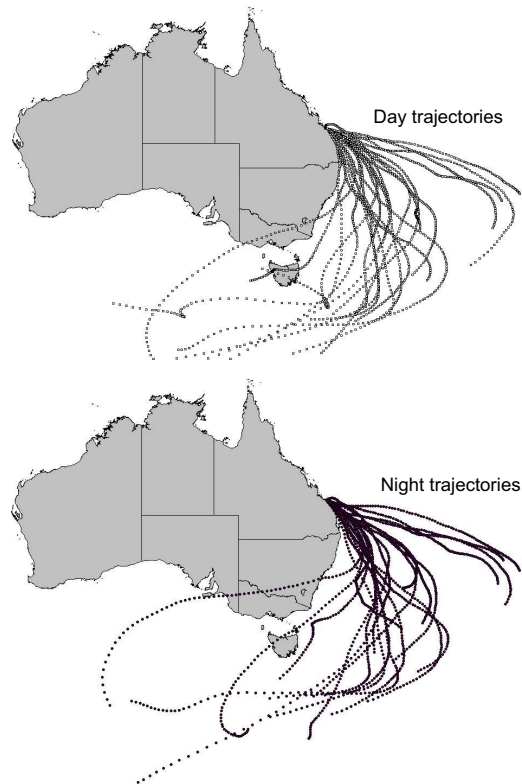
Fig. 3. HYSPLIT 96-h back trajectories for air masses arriving at Agnes Water at an altitude of 100 m on each day (12:00 local time) and night (02:00 local time) of the campaign. Note that there was no significant between these trajectories and the trajectories of air masses arriving at altitudes of 10 m and 1000 m.
