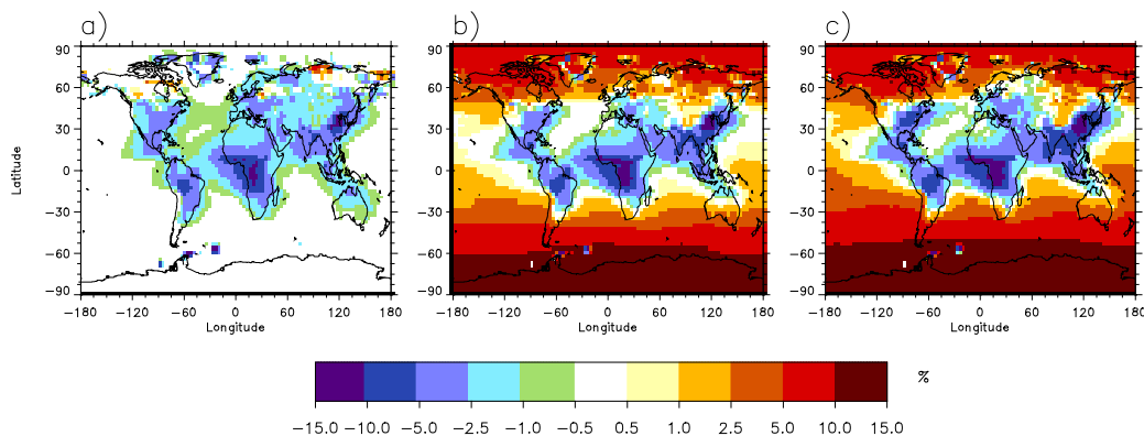
Fig. 8. Percentage change in estimated annual mean total change for three UV-bands. The changes are shown for (a) UVA, (b) UVB and (c) UV-E radiation at the surface since pre industrial time (1750–2000).
