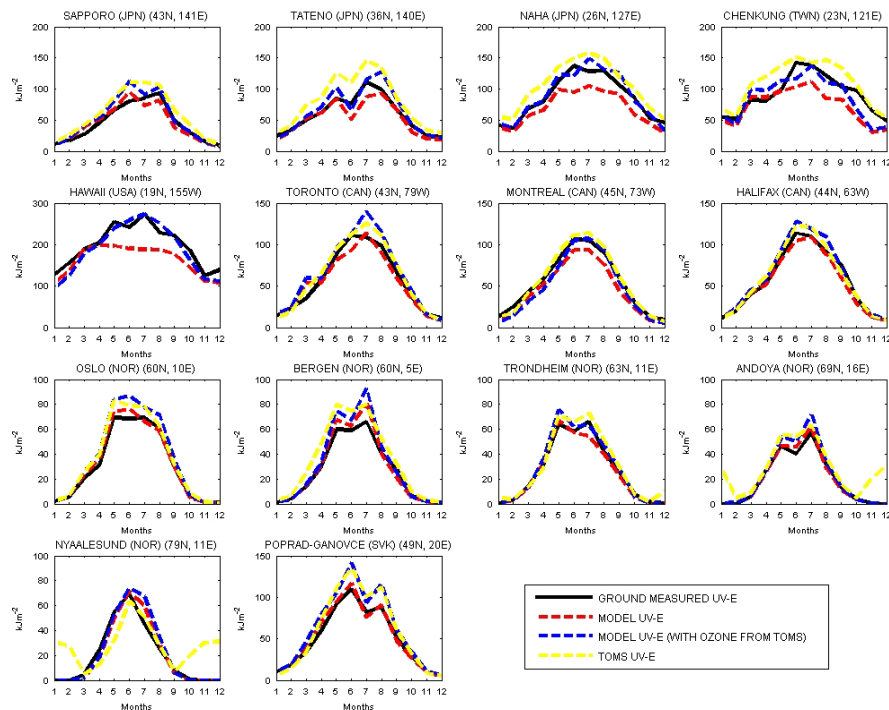
Fig. 2. Monthly surface UV-E doses at 14 sites for year 2000. Black – ground based measurements, red – model, blue – model including ozone data from TOMS, and yellow – TOMS surface UV-E retrieval. The UV observations from nine sites were obtained from the World Ozone and Ultraviolet Radiation Data Centre (WOUDC). The Norwegian institute for Air Research hosts the five Norwegian UV observations.
