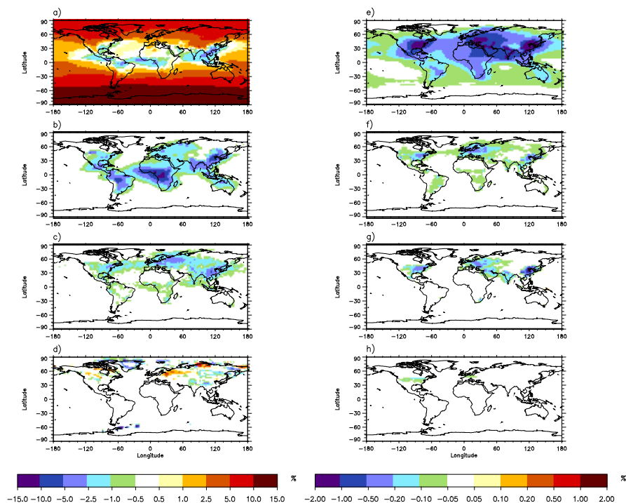
Fig. 5. Percentage change in estimated annual mean UV-E at the surface since 1750. The UV-E changes are due to (a) ozone (both tropospheric and stratospheric), (b) carbonaceous aerosols, (c) cloud albedo effect (first indirect effect) of aerosols, (d) surface albedo, (e) sulphate aerosols, (f) \text{NO}_2 , (g) \text{SO}_2 , and (h) aviation induced contrails and cirrus. Note the different color scale for the left and right panels.
