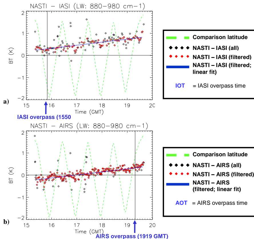
Fig. 19. Time series representation of (a) NAST-I – IASI and (b) NAST-I – AIRS for a long-wave spectral interval (880–980 cm -1 ). Space coincidence is achieved for each comparison point whereas time coincidence is only achieved at satellite overpass times.
