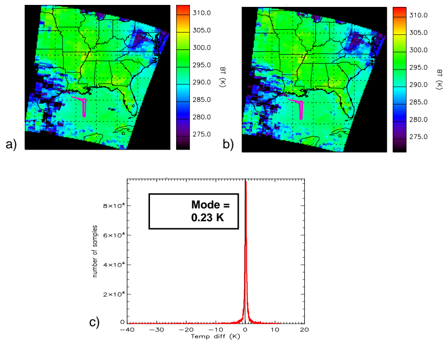
Fig. 5. IASi versus IASi imager for the Metop-A scene over the 29 April 2007 JAIVEx flight mission: (a) imager degraded to IASi spatial resolution over IASi scene, (b) IASi degraded through application of IASi imager spectral response function, and (c) histogram of scene (a) – scene (b).
