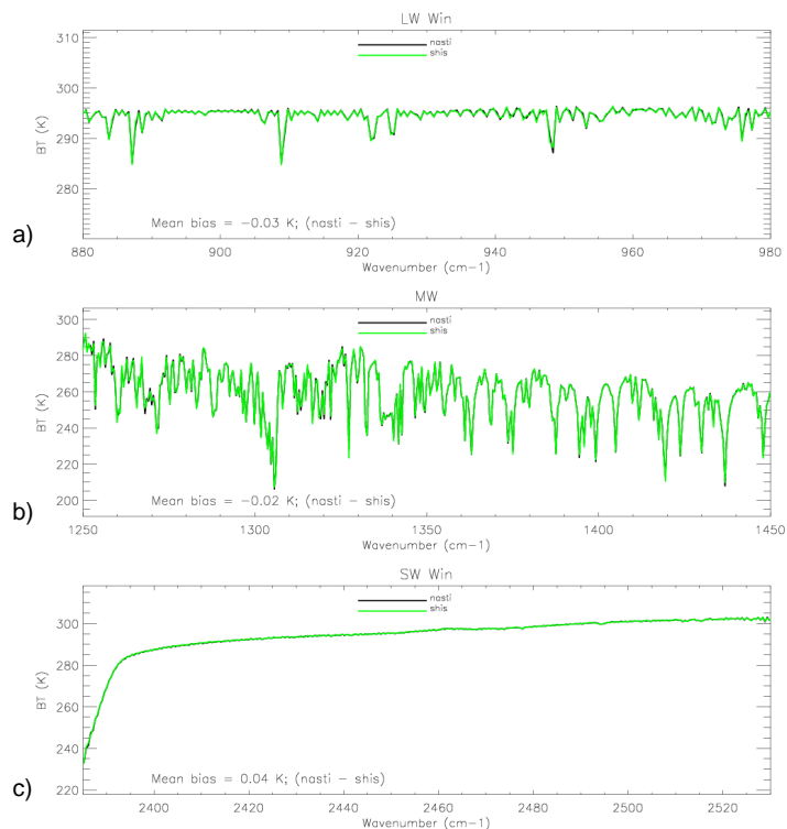
Fig. 7. Average NAST-I versus S-HIS spectra for collocated scenes during the 29 April 2007 JAIVEx flight mission, for the (a) longwave window (880–980 cm -1 ), (b) midwave (1250–1450 cm -1 ), and (c) shortwave window (2385–2530 cm -1 ) spectral regions. Note that the higher-resolution NAST-I data have been reduced to the S-HIS spectral resolution.
