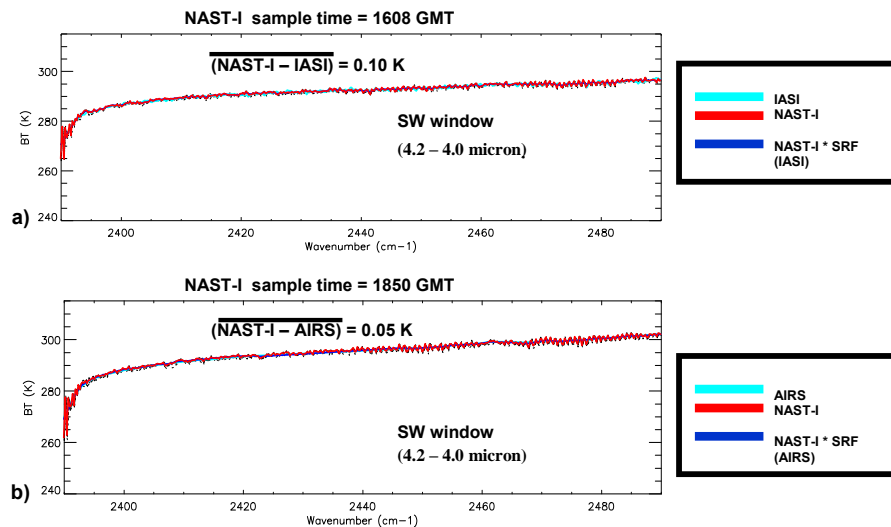
Fig. 14. Example infrared spectral radiance inter-comparisons for the shortwave window 2390–2490 cm -1 spectral region showing space and time coincident NAST-I relative to (a) IASI and (b) AIRS measurements.
