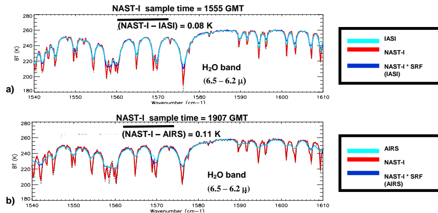
Fig. 13. Example infrared spectral radiance inter-comparisons for the water vapor 1540–1610 \text{cm}^{-1} spectral region showing space and time coincident NAST-I relative to (a) IASI and (b) AIRS measurements.
