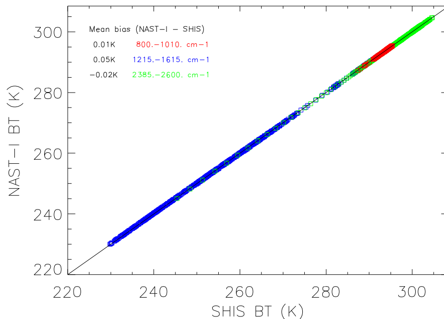
Fig. 8. Scatter plot of NAST-I versus S-HIS for average spectra shown in Fig. 7. The higher-resolution NAST-I data have been reduced to the S-HIS spectral resolution and spectra have been smoothed over 10\text{ cm}^{-1} to better facilitate radiometric calibration inter-comparison. As indicated in the Figure, the 800–1010, 1215–1615, and 2385–2600 \text{cm}^{-1} spectral regions are shown.
