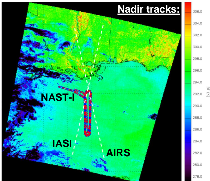
Fig. 17. Nadir tracks of IASI, AIRS, and NAST-I superimposed over the IASI imager scene of the JAIVEx flight region.
