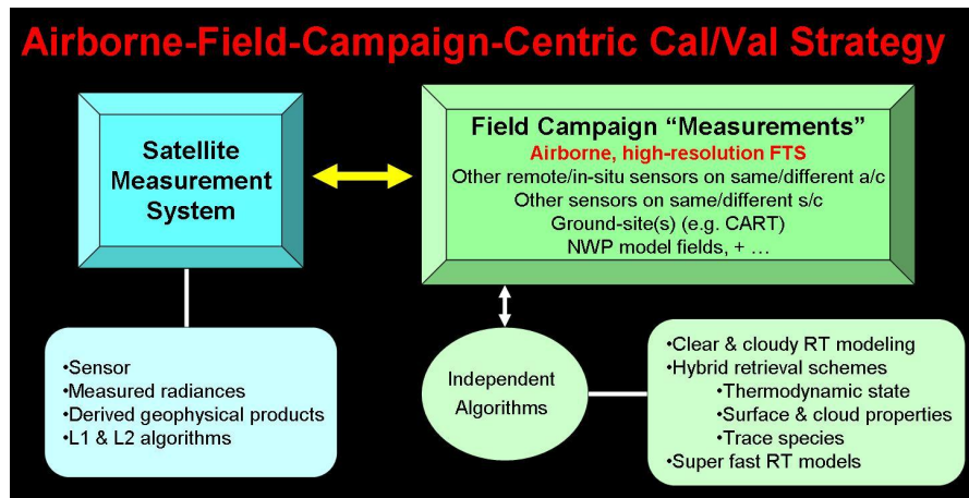
Fig. 3. Calibration/Validation strategy employed by LaRC team for the conduct of NAST-I field experiments.
