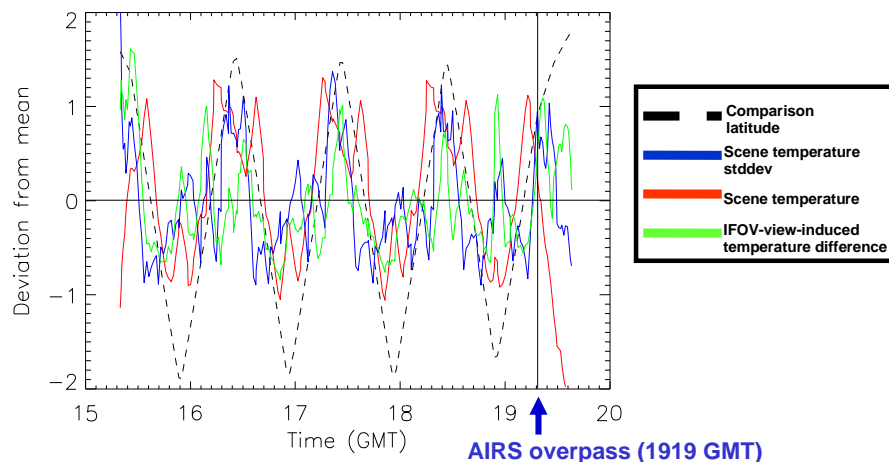
Fig. 18. Latitudinal variability of geophysical field as observed in aircraft/spacecraft measurement comparison. Sub-pixel Modis data are used to represent scene characteristics within AIRS IFOV positions and for view-induced differences relative to comparisons with NAST-I. Latitude, scene temperature and standard deviation, and IFOV-view-induced differences (i.e. between a/c and s/c geometries) are shown for comparison sample positions as a function of NAST-I sample time.
