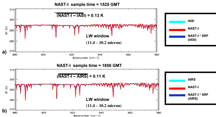
Fig. 12. Example infrared spectral radiance inter-comparisons for the longwave window 880–980 \text{cm}^{-1} spectral region showing space and time coincident NAST-I relative to (a) IASI and (b) AIRS measurements.
