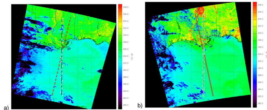
Fig. 9. Nadir and common cross-section lines extracted for first-order direct comparison of IASI and AIRS, \pm 5 degrees latitude from sub-satellite intersection point of the satellite ground tracks for (a) IASI and (b) AIRS. Tracks are shown on top of platform imager scenes, i.e., IASI imager and Modis B31, respectively.
