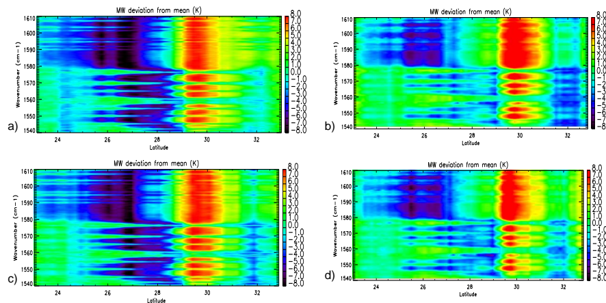
Fig. 10. Water vapor band ( 1540\text{--}1610\text{ cm}^{-1} ) latitudinal cross-sections (deviation from mean, K) along sub-satellite nadir for (a) IASI, (b) AIRS, and along a common cross-section for (c) IASI and (d) AIRS. Nadir cross-sections have point-in-space coincidence while common cross-sections have line-in-space coincidence.
