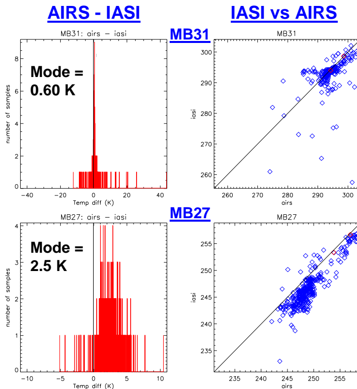
Fig. 11. Direct comparison of IASI and AIRS coincident IFOVs within the JAIVEx 29 April 2007 flight domain. Select Modis spectral response functions have been applied (to the IASI and AIRS spectral radiances) to illustrate scene evolution (between satellite overpasses) from a broadband difference perspective. Longwave window (MB31) and midwave water vapor (MB27) regions are shown in the top and bottom plots, respectively.
