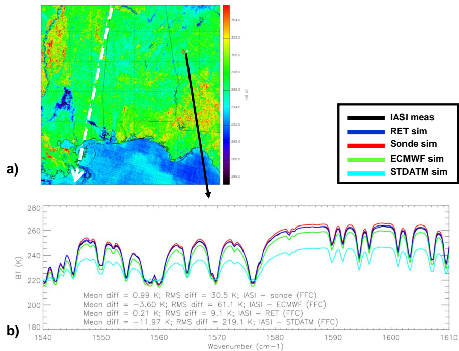
Fig. 4. IASI measured spectra versus simulation for a select IFOV on the 29 April 2007 JAIVEx region overpass at 15:50 GMT. Selected IFOV position shown within the IASI imager scene data in (a) along with the sub-satellite track (white-dashed arrow).
