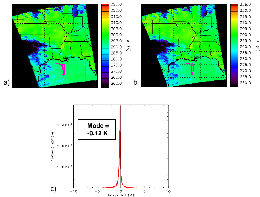
Fig. 6. AIRS versus Modis Band 31 (MB31) for the Aqua scene over the 29 April 2007 JAIVEx flight mission: (a) MB31 degraded to AIRS spatial resolution over AIRS scene, (b) AIRS spectrally degraded through application of MB31 spectral response function, and (c) histogram of scene (a) – scene (b).
