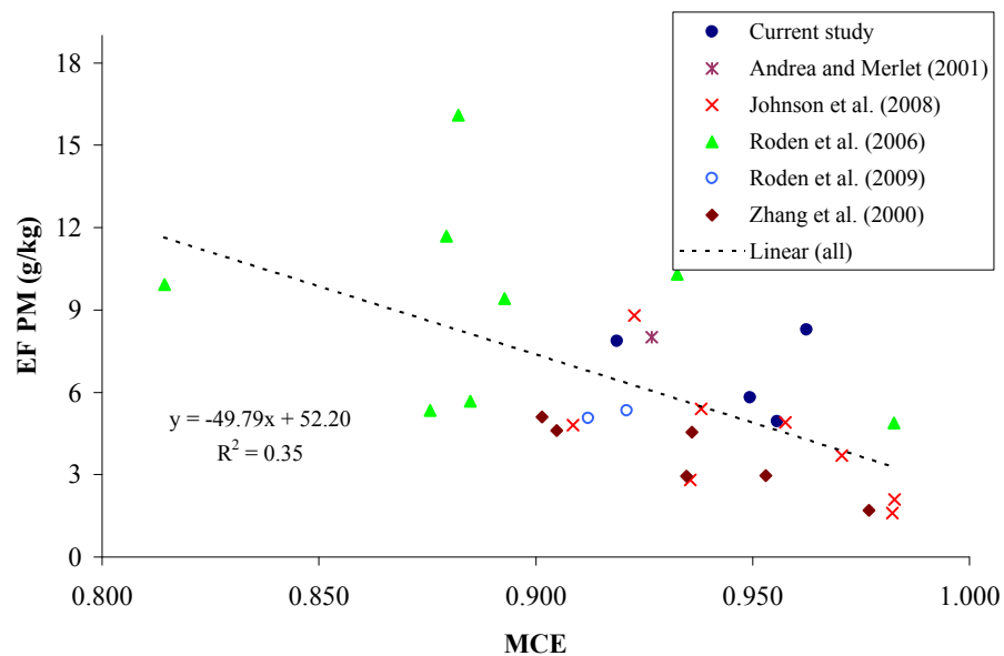
Fig. 3. Variation of the particle emission factor with MCE for open wood cooking fires.
