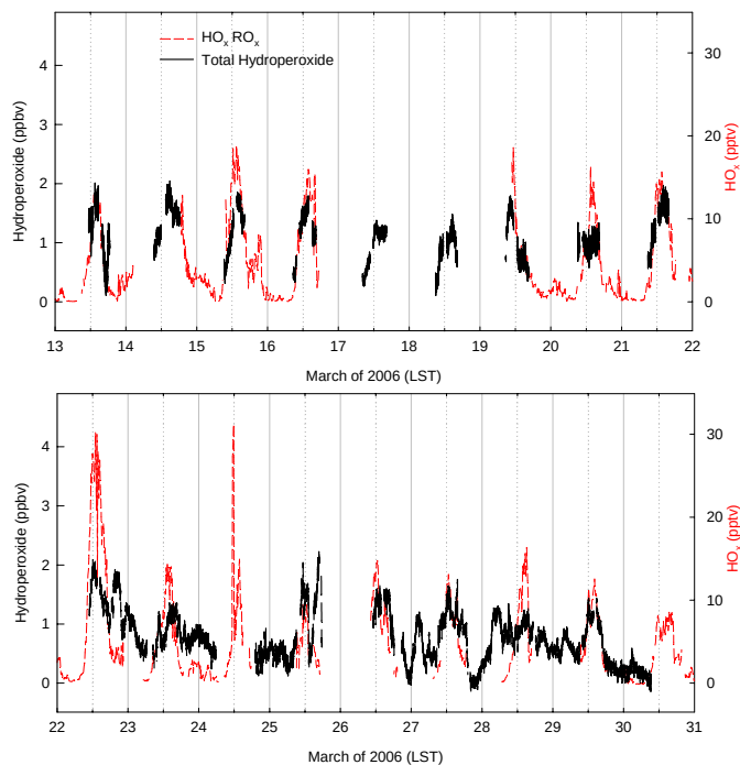
Fig. 11. Time series of hydroperoxides (black) along with \text{HO}_2 radicals (red) at Tecamac University.
