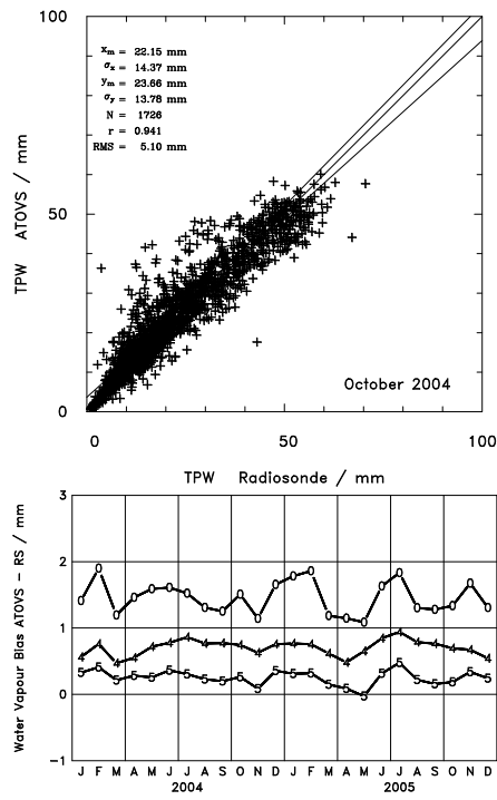
Fig. 5. Global comparison of daily averages of vertically integrated water vapour for October 2004 (top) and global mean bias error for the total column (curve denoted by 0) and the layers 1000–850 (denoted by 5) and 850–700 hPa (denoted by 4) (bottom).
