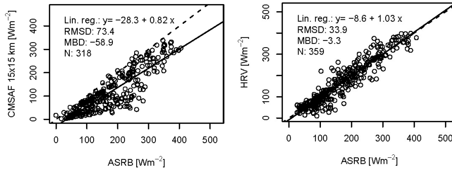
Fig. 11. Comparison of daily solar incoming radiation derived from SEVIRI solar channels (left panel) and the SEVIRI HRV channel (right panel) against ground-based measurements taken at Weissfluhjoch (Switzerland) for the period August 2004–July 2005.
