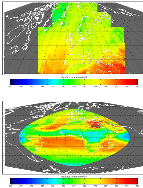
Fig. 1. Monthly mean cloud-top temperature for September 2007 derived from AVHRR observations (top panel) and from Meteosat9/SEVIRI (lower panel).
