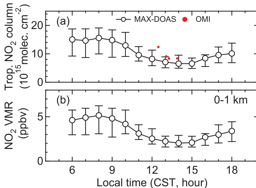
Fig. 7. (a) Median diurnal variation of the tropospheric NO 2 columns measured by MAX-DOAS at Tai'an over the period from 29 May to 29 June 2006. Error bars represent 67% ranges. Daily mean OMI data obtained within 0.1° latitude and longitude of Tai'an are also plotted in red. The local time is the Chinese standard time. (b) Same as (a), but for the mean MAX-DOAS NO 2 VMR values for the 0–1-km layer above the surface.
