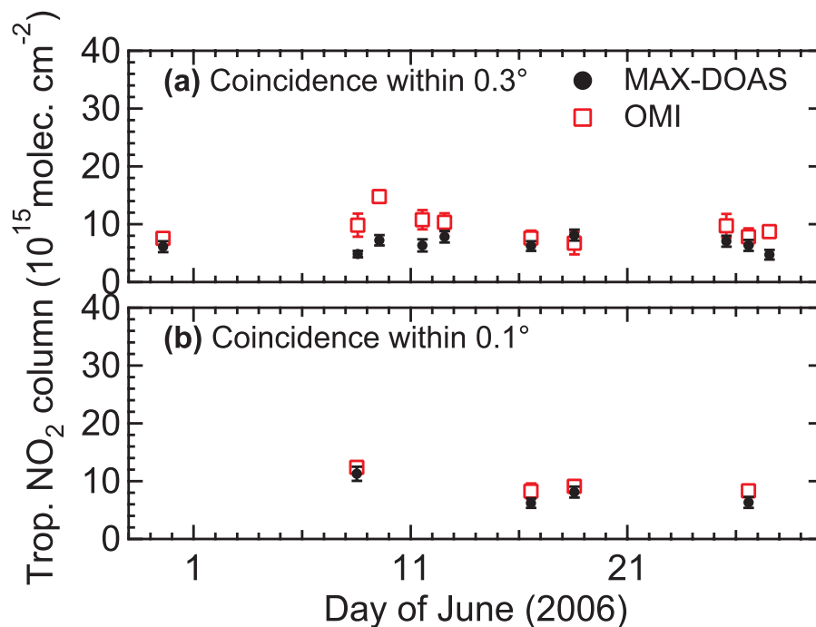
Fig. 8. Coincident pairs of Tai'an MAX-DOAS (black) and OMI (red) selected with coincident location criteria of (a) 0.3° and (b) 0.1°. Daily mean OMI data over Tai'an are plotted. Error bars represent 1 \sigma standard deviations.
