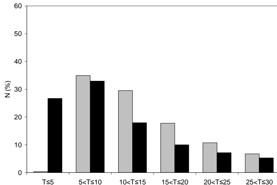
Fig. 4. Histogram of the percentage of the occurrences when the time required for an exposure of 1/3 MED due to diffuse (grey bar) and global (black bar) UV_{ery} falls within a certain time range provided in units of minutes.
