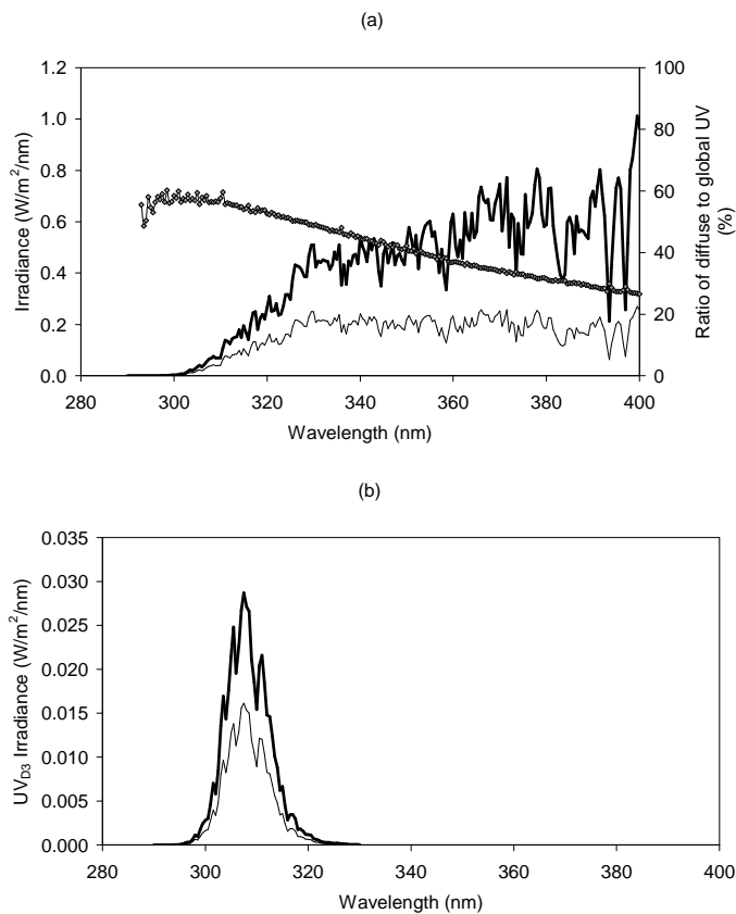
Fig. 1. Diffuse (light line) and global (heavy line) spectral UV irradiances taken on 17 August 2005 at approximately 11:00 EST and the spectral ratio of diffuse to global UV (a) ; and global and diffuse spectral irradiances from (a) weighted with the pre-vitamin D 3 action spectrum (CIE, 2006).
