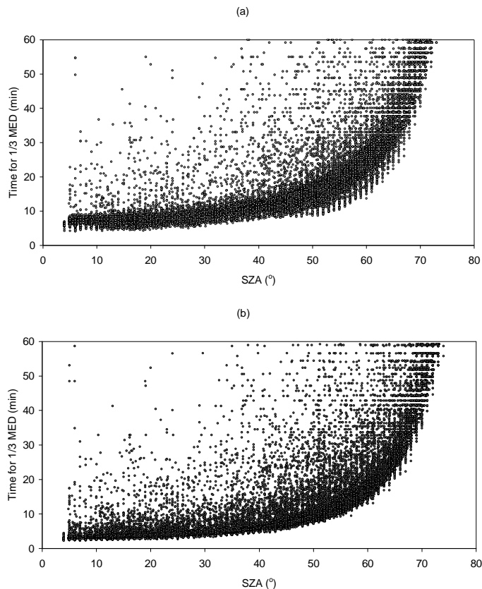
Fig. 2. The times required for an exposure of 1/3 MED due to diffuse UV ery (a) and global UV ery (b) as a function of SZA for all sky conditions during 2003.
