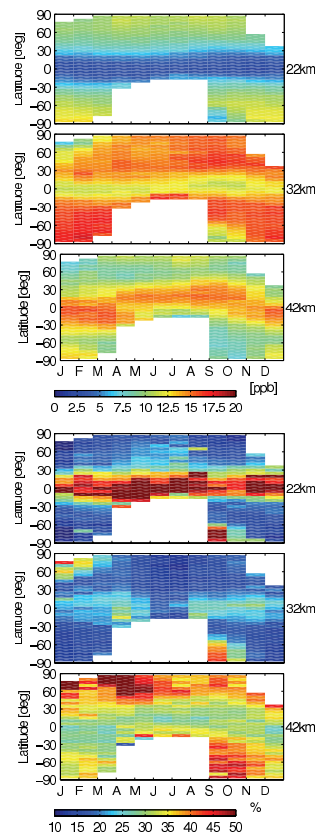
Fig. 8. Annual variation of NO y mean volume mixing ratio [ppb] (upper plot) and 1 \sigma standard deviation [%] (lower plot) of the Odin proxy climatology at three different altitude levels as a function of latitude [deg]. White regions represent periods and regions without data coverage.
