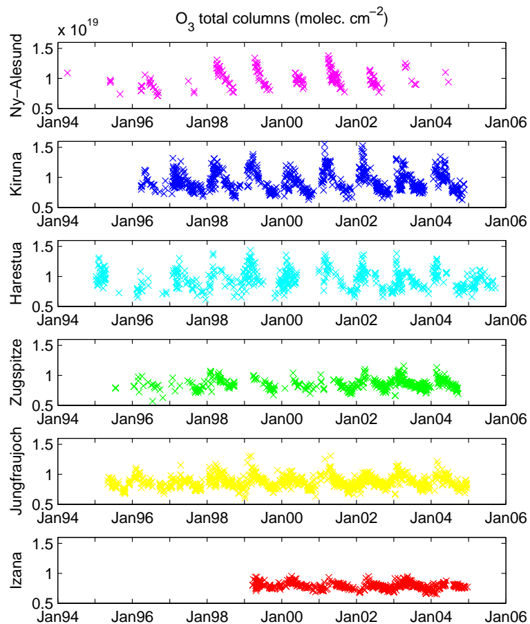
Fig. 5. Time series of \text{O}_3 total columns at each station.
