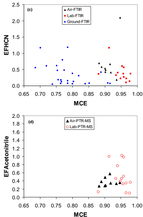
Fig. 4. (c) and (d) The EF for HCN or acetonitrile did not show a strong dependence on MCE over the range of measurements obtained in TROFFEE. Thus, our study-average EF likely represent both the lofted and the initially unlofted emissions produced by tropical deforestation fires. Since these compounds are thought to be emitted mainly by biomass burning and the EF is relatively MCE-independent, the average EF can be used for source apportionment without great concern that the often-undersampled initially-unlofted emissions actually contribute a significantly different EF. On the other hand, the large variability in EF at all MCE limits the precision of estimates.
