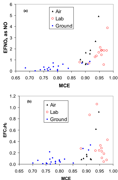
Fig. 3. Presentation of all the emission factors measured during TROFFEE from ground-based, airborne, and laboratory platforms for NO x (a) and C 2 H 2 (b). Despite differences in fuels between the experiments, these compounds show a consistent trend of increasing emissions with increasing MCE indicating production mainly by weakly fuel-dependent flaming combustion. There is also a large range in the EF observed (factor of ~20).
