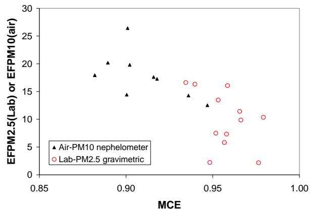
Fig. 5. The gravimetric PM_{2.5} measurements in the lab and the nephelometer based PM_{10} measurements from the airborne campaign are consistent with each other. Both data sets indicate that an emission factor for fine particles in the range of 20–30 g/kg would be reasonable at a fire integrated MCE of 0.861, which is appropriate for pasture maintenance fires (Sect. 3.2).
