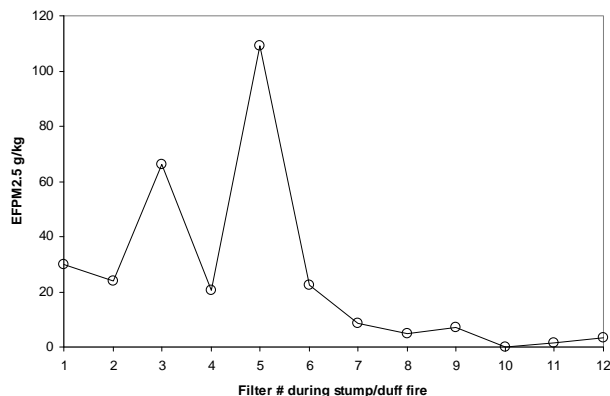
Fig. 6. A series of gravimetric determinations of \text{EFPM}_{2.5} acquired over the course of a laboratory fire described by Bertschi et al. (2003a). The first 6 samples were taken while a woody stump accounted for all the fuel consumption. Filters 7–9 sampled a mix of burning roots and duff. Samples 10–12 were of burning duff. The mass-loss weighted average EF for the woody stump is about 30 g/kg. This indicates that a similar \text{EFPM}_{2.5} could be appropriate for the smoldering logs, which account for nearly all the unlofted emissions from residual smoldering combustion in Brazil.
