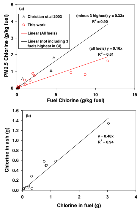
Fig. 1. Partitioning of fuel chlorine to PM 2.5 and ash. The upper trend line (black) in (a) is a regression fit to the data from Christian et al. (2003) and this study excluding the three fuels from this study with the highest chlorine content. The lower (red) trend line in (a) includes all the data from both studies. Panel (b) shows all the measurements (all made in this study) of the fraction of fuel chlorine remaining in the ash.
