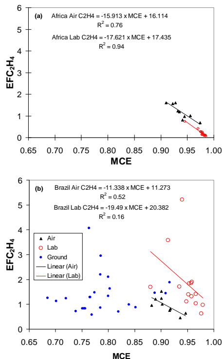
Fig. 4. (a) The relevant range of fire-integrated MCE for savanna fires is about 0.90–0.98. For C_2H_4 , over this range, the EF from airborne measurements of African savanna fires and the lab EF measured using savanna fuels are in good agreement with each other and highly correlated with MCE. (b) The agreement between the lab and air and the correlation with MCE decreases for tropical forest fire EF. Including the ground-based field data indicates that EFC_2H_4 may be fuel dependent (lower from woody material than foliage) and/or not uniquely identified with either flaming or smoldering combustion.
