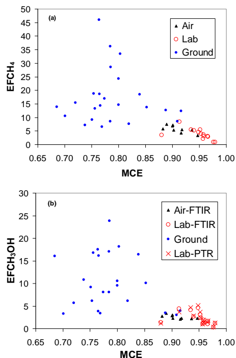
Fig. 2. Presentation of all the emission factors measured during TROFFEE from ground-based, airborne, and laboratory platforms for CH 4 (a) and CH 3 OH (b). Despite differences in fuels between the experiments, these compounds show a consistent trend of increasing emissions with decreasing MCE indicating fuel-independent production largely by smoldering combustion. There is also a large range in the EF observed (factor of ~20).
