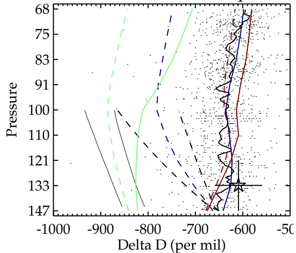
Fig. 5. The black points are ACE FTS measurements of \delta D between 12^\circ S to 12^\circ N for 2005 and 2006. The mean of the ACE-FTS \delta D is overlaid (black line). The CCT-TTL model runs for the same time period are (blue) SA, (green) C-NOICE, and (red) CSD01-ICE. The CCT-TTL model runs including tropical mixing are shown as solid lines and without extratropical mixing as dashed lines. The star is an average of TTL measurements made during CRYSTAL-FACE by ALIAS with the vertical bar representing the altitude coverage of the average and the horizontal bar representing vertical accuracy. The thin solid black lines are Rayleigh distillation curves representing the seasonal extremes in temperature from the surface. The thick dashed black lines are Rayleigh distillation curves representing the seasonal extremes beginning at the prescribed \delta D for the lower TTL boundary.
