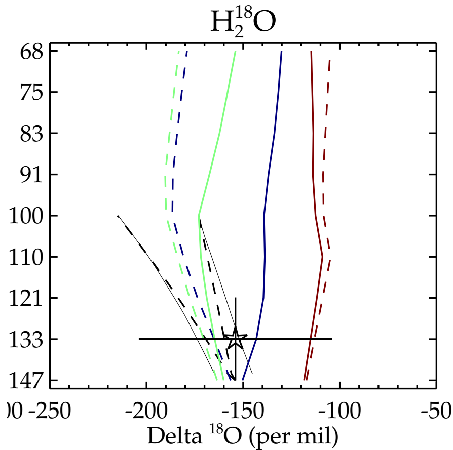
Fig. 7. Same as Fig. 5 but for \delta^{18}\text{O} .
