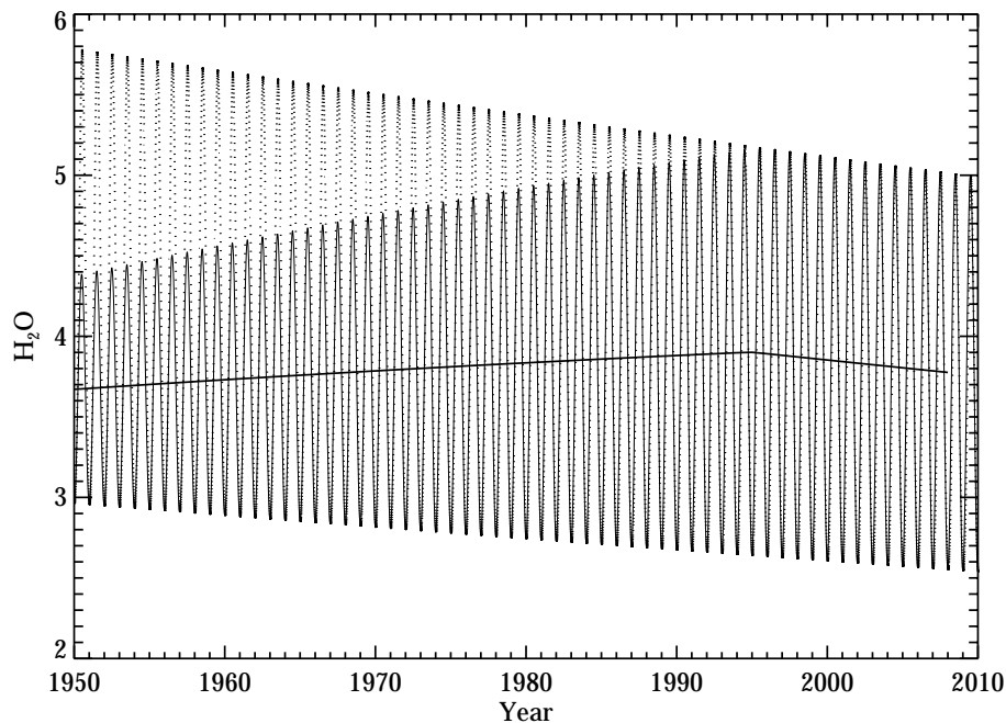
Fig. 8. A schematic representation of how \text{H}_2\text{O} can show the observed trend as described in the text. The dots are the SMR under cold trap temperature control assuming -0.15 K/decade tropopause temperature trend (Lanzante et al., 2003). The thin line is \text{H}_2\text{O} under increasing convective influence assumed here to reduce the time the tropics is subsaturated by 1% per year. The thick line is a hypothetical entry \text{H}_2\text{O} trend.
