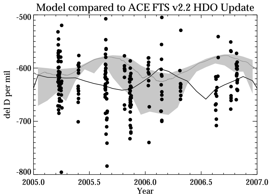
Fig. 6. ACE-FTS \delta D measurements between 12^\circ S and 12^\circ N between 100 and 80 hPa (solid circles) shown as a function of time. The black solid line is a temporally smoothed mean of the ACE-FTS data. The grey shading represents the longitudinal variation of \delta D from the CSD01-ICE run. Dark grey is the mean of the CSD01-ICE \delta D .
