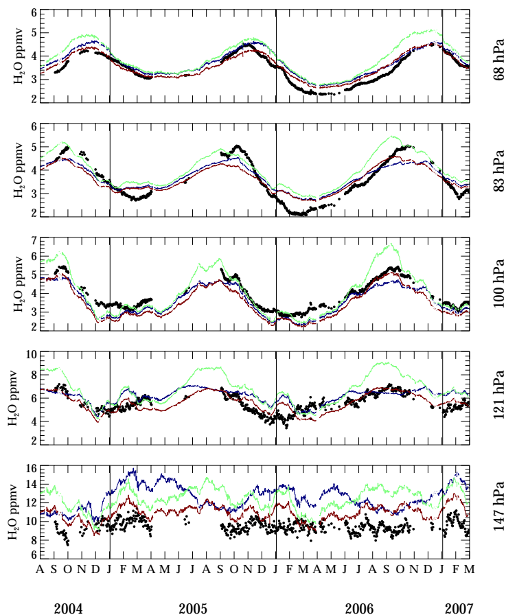
Fig. 3. Same as Fig. 2 except it shows v2.21 Aura MLS \text{H}_2\text{O} and the model runs are smoothed by the Aura MLS forward model smoothing function and v2.2 averaging kernel (Read et al., 2007).
