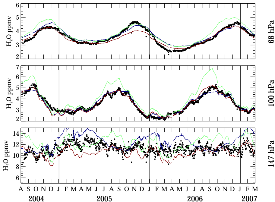
Fig. 2. (black points) H 2 O time series at 147, 100, and 68 hPa, for Aura MLS v1.5, CCT-TTL model runs, (blue) SA, (green) C-NOICE, and (red) CSD01-ICE. The Aura MLS measurements are daily zonal means between 12° S–12° N. The model runs are smoothed by the Aura MLS forward model smoothing function and v1.5 averaging kernel (Read et al., 2007).
