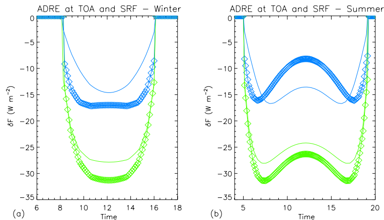
Fig. 9. Diurnal cycle of the aerosol direct radiative effect, computed for the reference bin ( \tau_a \approx 0.21 ) for 15 January (a) and July (b). \delta F^{\text{TOA}} (blue) and \delta F^{\text{SRF}} (green) are represented for the Po Valley (line+diamonds) and the AAOT (line) cases.
