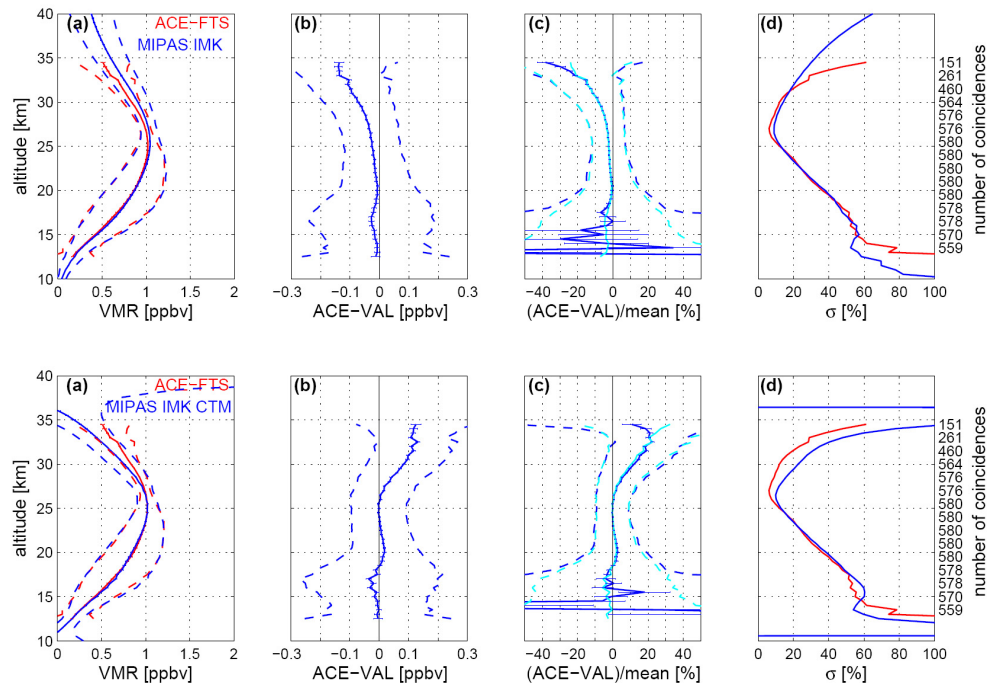
Fig. 8. Same as Fig. 2 but for \text{ClONO}_2 comparisons between ACE-FTS and the MIPAS IMK-IAA data product for coincident measurements between 30^\circ\text{N} – 90^\circ\text{N} ( \pm 9\text{h} , 800\text{km} , \pm 3 \times 10^{-6}\text{km}^2\text{kg}^{-1}\text{s}^{-1} at 475\text{K} ). Panels (c) also show the mean relative deviation from the mean, calculated using Eq. (4) (cyan solid line) with \pm 1\sigma relative standard deviation (cyan dashed line). Top row: MIPAS uncorrected data. Bottom row: MIPAS CTM-corrected data.
