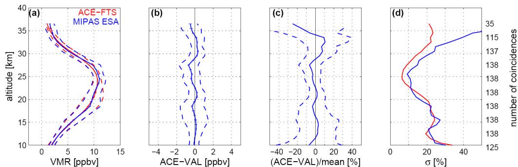
Fig. 6. Same as Fig. 2 but for \text{HNO}_3 comparison between ACE-FTS and the MIPAS ESA data product for coincident measurements between 20^\circ \text{N} and 85^\circ \text{N} ( \pm 6 \text{ h} , 300 \text{ km} ).
