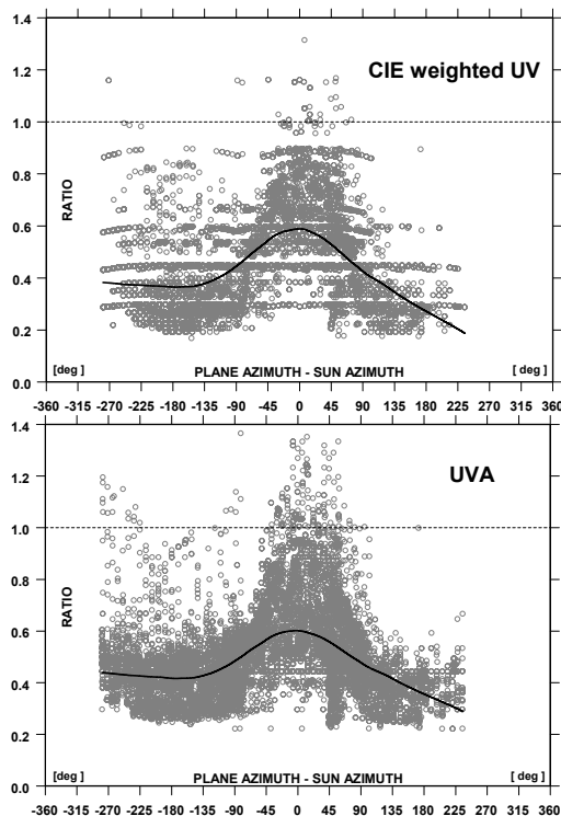
Fig. 6. Relative biologically weighted UV irradiance on rotating vertical plane measured at the ALOMAR observatory in the period 1–15 June 2007, for various configurations of the plane and action spectra : erythral data – top, integrated UVA data – bottom.
