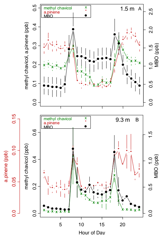
Fig. 6. Average diurnal profiles of methyl chavicol (x) , MBO (•) , and \alpha -pinene (*) (mean \pm standard error). (A) Measurements made at 1.5 m above the ground; MBO measured by PTR-MS. (B) Measurements made at 9.3 m; MBO measured by NOAA GC-MS.
