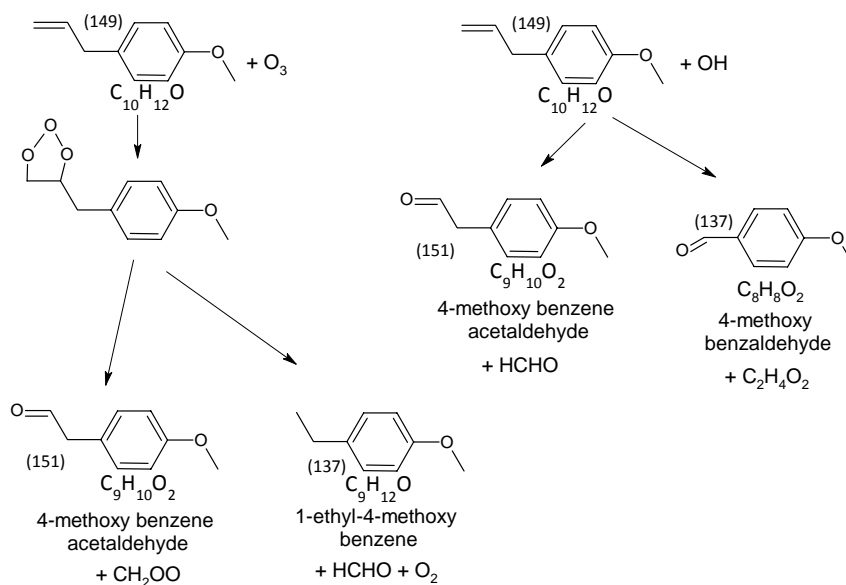
Fig. 8. Schematic of methyl chavicol oxidation products from reanalysis of laboratory methyl chavicol oxidation experiments by Lee et al. (2006a, b). Mass/charge ( m/z ) ratios detected by PTR-MS are indicated in parentheses.
