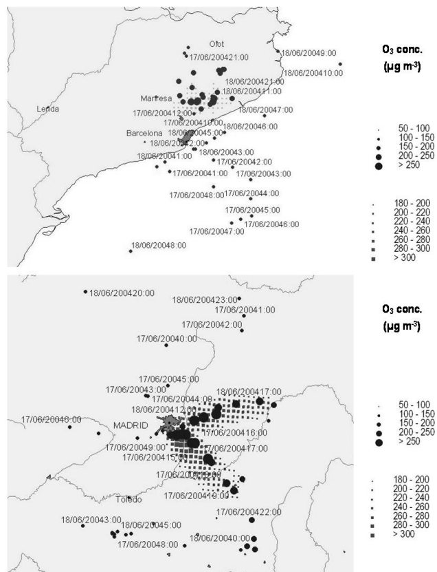
Fig. 4. Hourly maximum O 3 surface concentration location (circles) in the coastal (up) and the central (down) domains during the 17–18 June 2004 episode, simulated by WRF-ARW/HERMES-2004/CMAQ. Squares: concentrations above the EU human health protection limit (180 µg m -3 , Dir 2002/3/EC).
