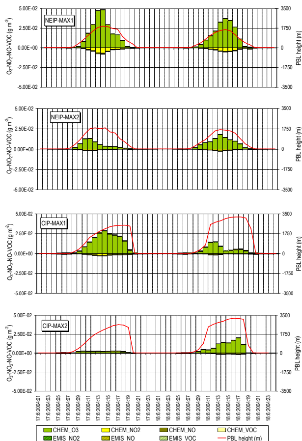
Fig. 11. Gas-phase chemistry and emissions contributions to net \text{NO}_x\text{-NMVOCs-O}_3 density ( \text{g m}^{-2} ) under the modelled PBL height (in red) during 17–18 June 2004 for the NEIP-MAX1 and MAX2 domains, and the CIP-MAX1 and MAX2 domains.
