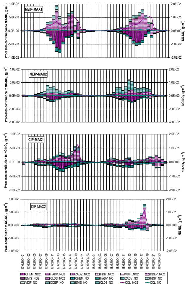
Fig. 9. Atmospheric processes contribution to net NO x density (g m -2 ) under the modelled PBL during 17–18 June 2004. A veraged contributions for the NEIP-MAX1 and MAX2 domains, and CIP-MAX1 and MAX2 domains. 18495
