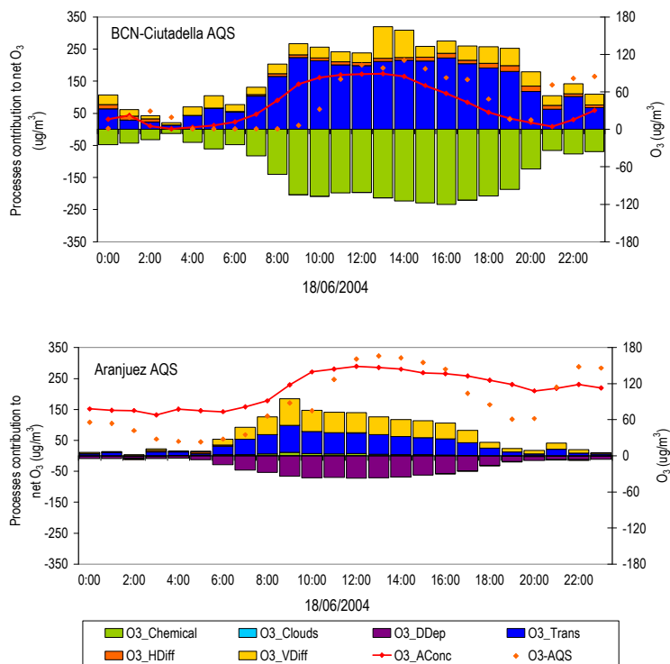
Fig. 3. Atmospheric processes contribution to net O 3 concentration in the first simulated vertical layer (0–38 m a.g.l.), O 3 hourly average concentration and O 3 measured in urban background air quality stations of the NEIP (BCN-Ciudadella AQS) and the CIP domain (down-Aranjuez AQS) during 18 June 2004.
