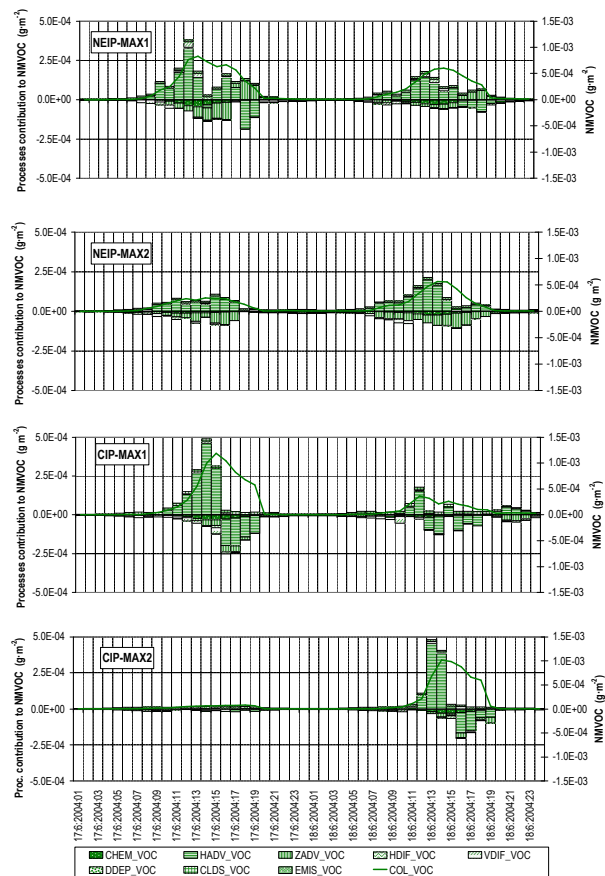
Fig. 10. Atmospheric processes contribution to net NMVOCs density ( \text{g m}^{-2} ) under the modelled PBL during 17–18 June 2004. Averaged contributions for the NEIP-MAX1 and MAX2 domains, and CIP-MAX1 and MAX2 domains.
