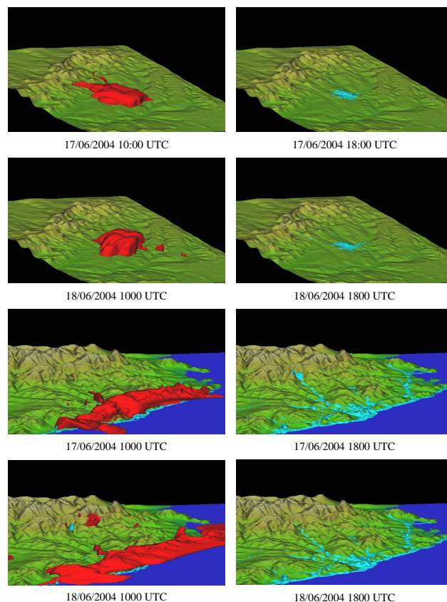
Fig. 5. 10 \mu\text{g m}^{-3} isosurface of chemical production (red) and destruction (blue) of \text{O}_3 for the CIP (up) and NEIP domains (down) at 10:00 and 18:00 UTC of 17–18 June 2004.
