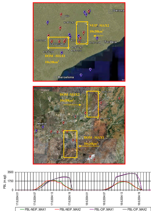
Fig. 7. Subdomains MAX1 and MAX2 (in yellow) selected in the NEIP (up) – MAX1: LAT: 41.63–41.72, LON: 2.08–2.32; MAX2: LAT: 41.67–41.85, LON: 2.42–2.54 – and CIP domains (down) – MAX1: LAT: 40.17–40.35, LON: –3.55–(–3.43); MAX2: LAT: 40.47–40.65; –3.36–(–3.24) –. Maximum hourly concentrations above 180 \mu\text{g m}^{-3} in red, concentrations below this limit in purple. Evolution of the modelled PBL height in the NEIP and CIP subdomains.
