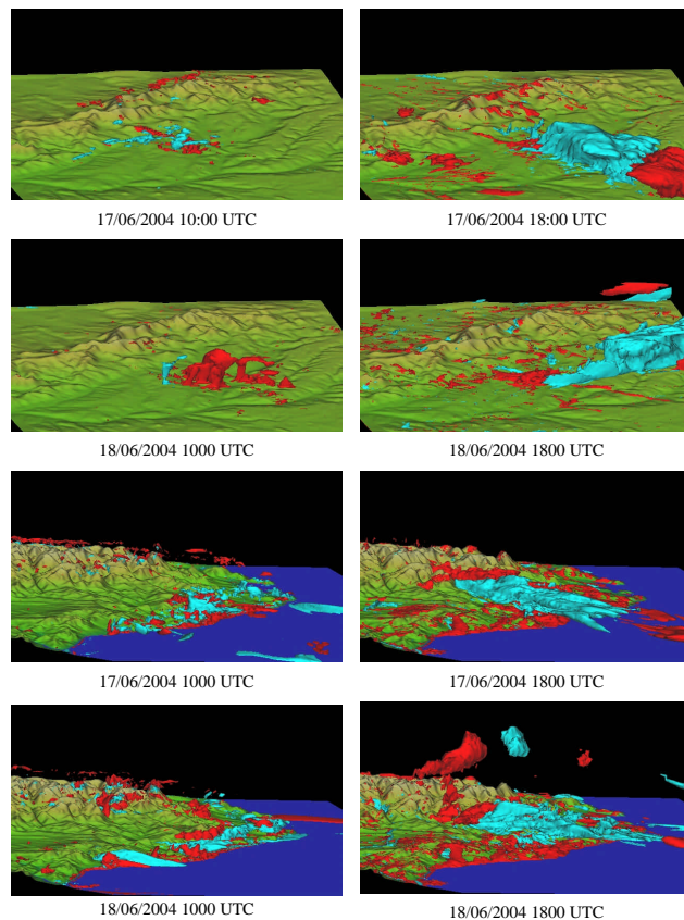
Fig. 6. 10 \mu\text{g m}^{-3} isosurface of \text{O}_3 net transport (horizontal + vertical advection) – positive contribution in red and negative contribution in blue – for the CIP (up) and NEIP domains (down) at 10:00 and 18:00 UTC of 17–18 June 2004.
