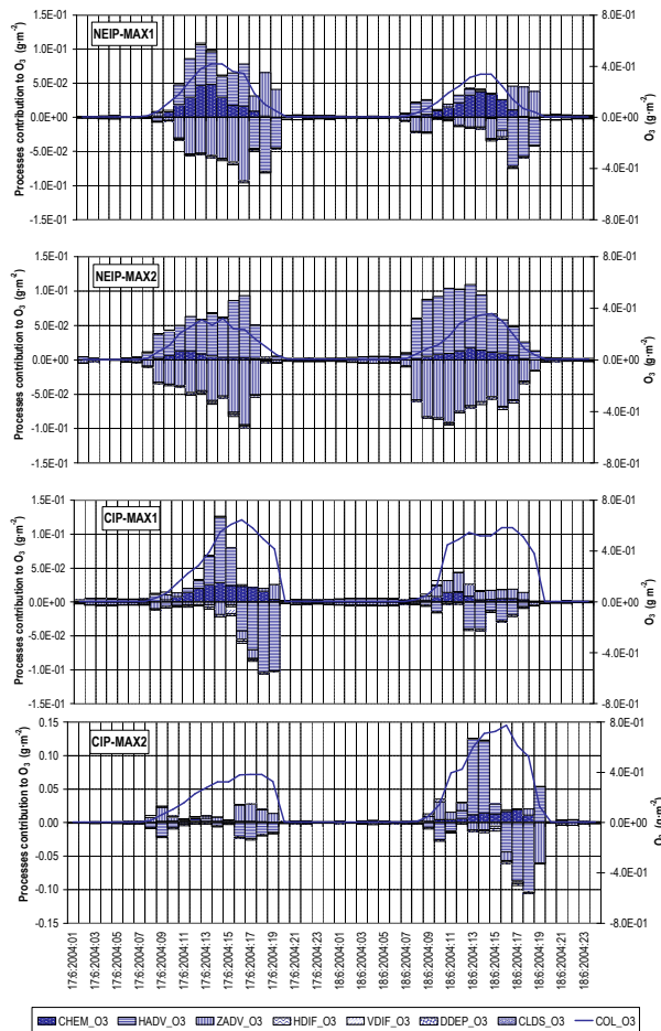
Fig. 8. Atmospheric processes contribution to net O_3 density ( g\ m^{-2} ) under the modelled PBL during 17–18 June 2004. Averaged contributions for the NEIP-MAX1 and MAX2 domains, and CIP-MAX1 and MAX2 domains.
