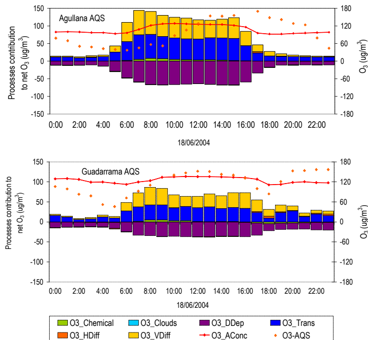
Fig. 2. Atmospheric processes contribution to net O 3 concentration in the 1st simulated vertical layer (0–38 m a.g.l.), O 3 hourly average concentration and O 3 measured in rural background air quality stations of the NEIP (up-Agullana AQS) and the CIP domain (down-Guadarrama AQS) during 18 June 2004.
