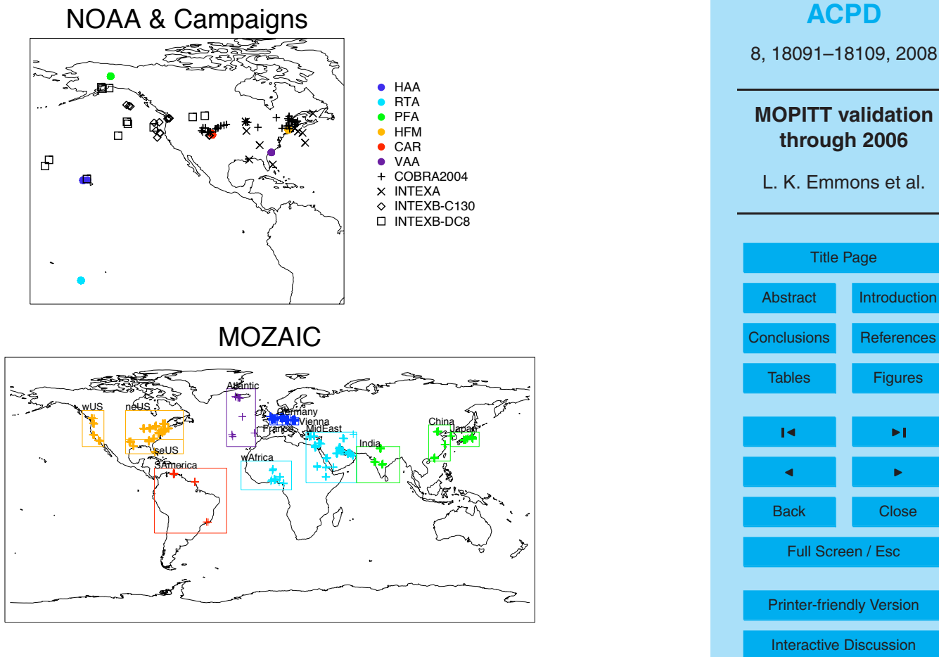
Fig. 1. Location of validation profiles used in this study. Top map shows NOAA routine sampling sites and field campaigns. Lower map shows individual profile locations and regional groupings.
