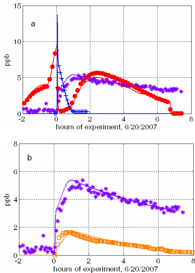
Fig. 3. Observations (symbols) and model calculations (lines) for dry \text{NO}_3 + \beta -pinene experiment. (a) \text{NO}_3 + \text{N}_2\text{O}_5 ( \bullet ), \beta -pinene ( + ), and total alkyl nitrates ( * ). (b) Total ( * ) and aerosol phase ( \square ) organic nitrate.
