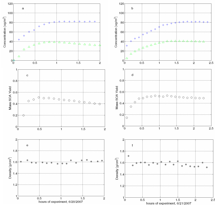
Fig. 5. Time evolution of \beta -pinene reacted ( \Delta ) and mass aerosol formed ( \bullet ) (using measured density) during the dry (a) and humid (b) experiments; mass yield (o) for dry (c) and humid (d) experiments; and density determined from comparison of AMS and SMPS measured mode diameter, for the dry (e) and humid (f) experiments. Peak mass yield (calculated immediately after all \beta -pinene is consumed) is 50% under both dry and humid conditions.
