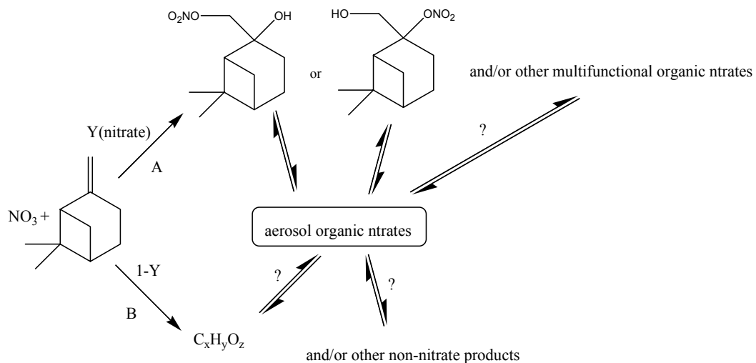
Fig. 2. \text{NO}_3 + \beta -pinene reaction mechanism. Absorptive partitioning of the two explicit \beta -pinene hydroxynitrates is included in the model mechanism. The remaining pathways identified with ? are discussed in the text.
