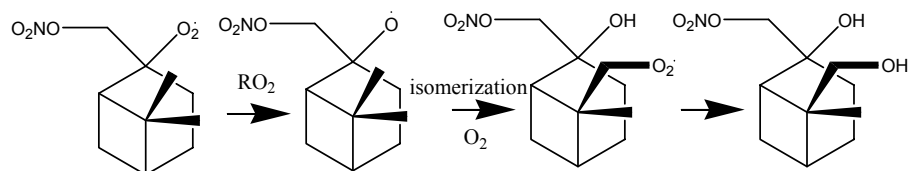
Fig. 4. Proposed isomerization mechanism for the initial nitrate-alkoxy radical leading to \beta -pinene dihydroxynitrates.
