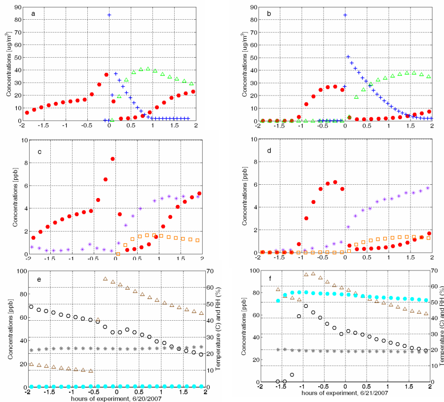
Fig. 1. Time evolution of \text{N}_2\text{O}_5 + \text{NO}_3 (•) and \beta -pinene (+) mass concentrations and total particle mass loading ( \Delta ) [ \mu\text{g}/\text{m}^3 ] (not corrected for losses), during the dry (a) and humid (b) experiments; time evolution of \text{N}_2\text{O}_5 + \text{NO}_3 (•), total alkyl nitrates (*) and aerosol nitrate ( \square ) concentrations [ppb], during the dry (c) and humid (d) experiments; and time evolution of \text{O}_3 (o) and \text{NO}_2 ( \Delta ) concentrations [ppb], temperature (*) [ ^{\circ}\text{C} ], and relative humidity ( \bullet ) [%] during the dry (e) and humid (f) experiments.
