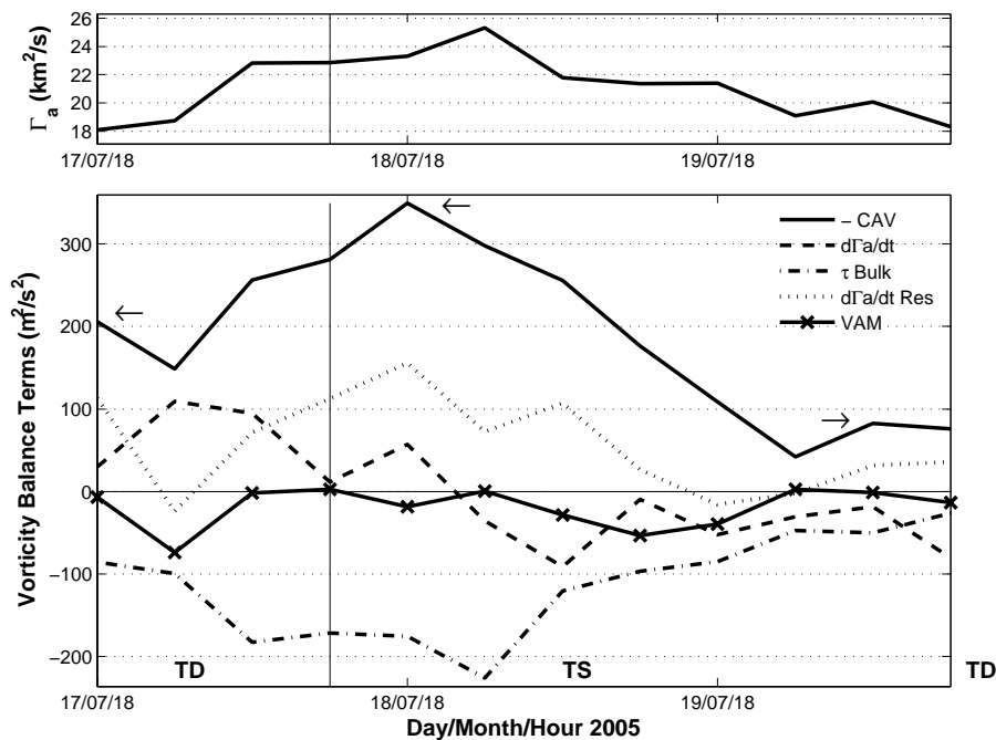
Fig. 4. Same as Fig. 3 but for tropical storm Eugene. Vertical solid lines delimit the tropical depression (TD) and tropical storm (TS) stages. Arrows indicate certain times that will be discussed in the text and in Figs. 9 and 10.
