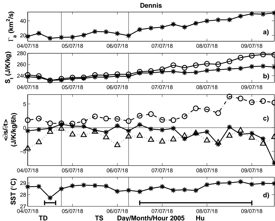
Fig. 11. Temporal distribution of (a) \Gamma_a averaged in the layer 1000–900 hPa, (b) entropy averaged over the 4^\circ \times 4^\circ domain (star) and entropy at the cyclone's center (open circle), both averaged over the depth of the troposphere (1000–100 hPa), (c) entropy tendency due to ventilation (star) and vertical advection of entropy (triangle) averaged over the 1000–100 hPa layer and the surface entropy flux (open circle) averaged over the inner points of the 4^\circ \times 4^\circ domain, and (d) sea surface temperature averaged over the 4^\circ \times 4^\circ domain for hurricane Dennis. Vertical solid lines delimit the tropical depression (TD), tropical storm (TS) and hurricane (Hu) stages. Periods when Dennis made landfall are indicated by horizontal bars.
