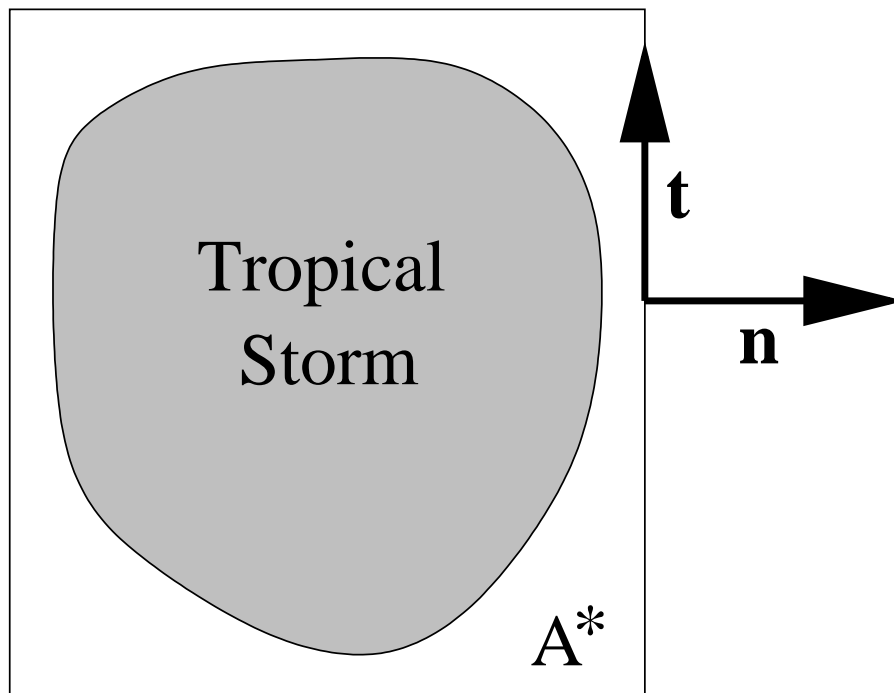
Fig. 2. Schematic representation of the tropical cyclone area (gray) and the area A^* where calculations are made at each pressure level. Vectors \mathbf{n} and \mathbf{t} are normal and tangential vectors to the periphery of A^* .
