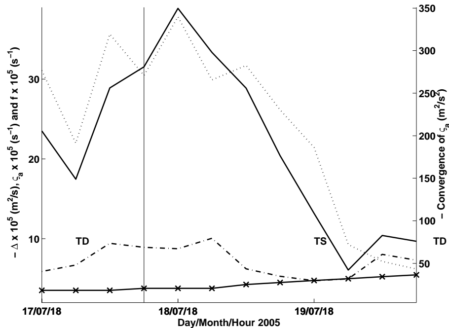
Fig. 6. Time evolution of minus the convergence of absolute vorticity (solid line), -\Delta (dotted line), and the absolute vorticity at the cyclone's boundary ( \zeta_a ) (dashed-dotted line) averaged over the 1000–900 hPa for tropical storm Eugene. The line with crosses represents the Coriolis parameter at Eugene's central latitude. The vertical solid line delimits the transition from tropical depression (TD) to tropical storm (TS).
