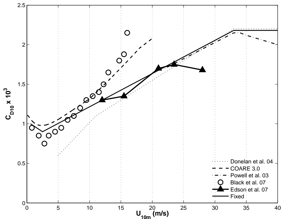
Fig. 16. Drag coefficient estimates as a function of the 10 m neutral wind from the several recent studies shown in the legend. The solid line shows the C_D obtained from them for this study.
