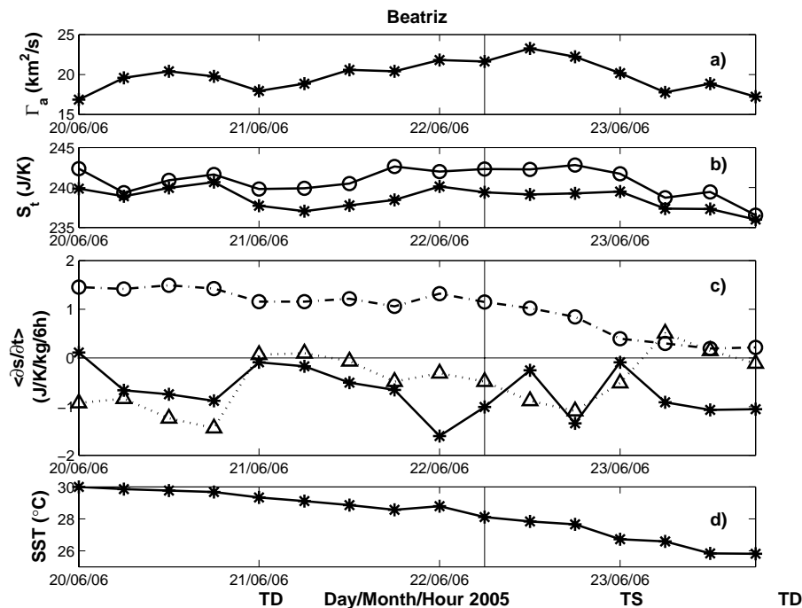
Fig. 13. Same as Fig. 11 but for tropical storm Beatriz. Vertical solid lines delimit the tropical depression (TD) and tropical storm (TS) stages.
