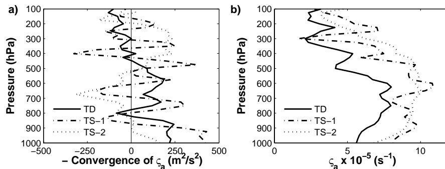
Fig. 9. Vertical profiles of (a) minus the convergence of absolute vorticity and (b) absolute vorticity at the cyclone's boundary averaged over the 4^\circ \times 4^\circ area at three times during tropical storm Eugene's life cycle. Tropical depression time (TD, solid line), first tropical storm time (TS-1, dashed-dotted line) and second tropical storm time (TS-2, dotted line) before it decayed back to tropical depression stage.
