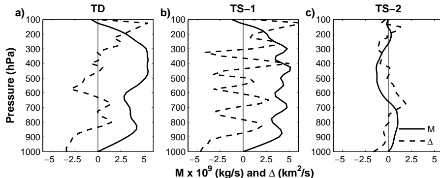
Fig. 10. Vertical profiles of horizontal ( \Delta , dashed line) and vertical ( M , solid line) mass fluxes for tropical storm Eugene at (a) the tropical depression time (TD), (b) the first tropical storm time (TS-1) and (c) the second tropical storm time (TS-2), before it decayed back to tropical depression stage.
