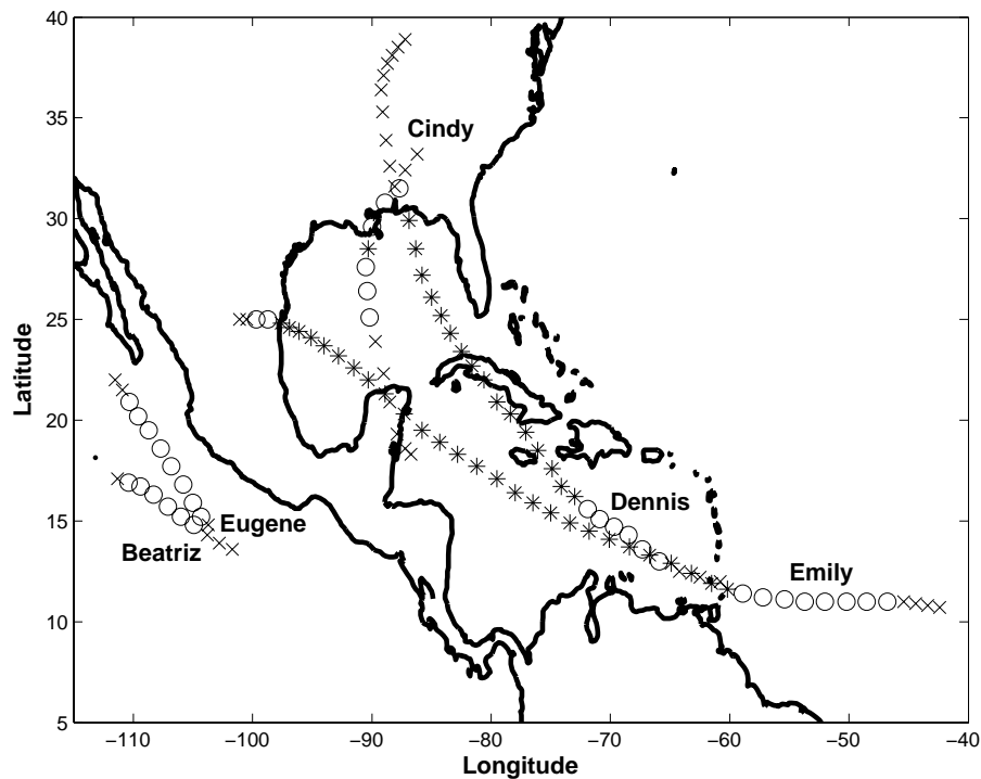
Fig. 1. Tracks of tropical cyclones studied. The tropical depression, tropical storm and hurricane stages are represented by crosses, open circles and stars, respectively.
