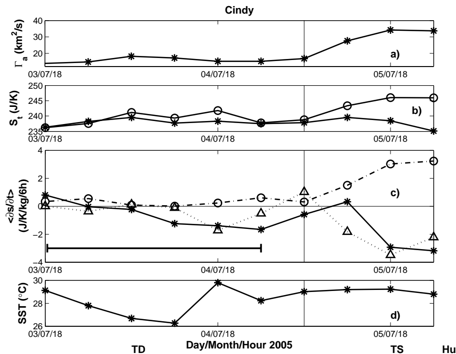
Fig. 14. Same as Fig. 11 but for hurricane Cindy. Periods when Cindy made landfalling are indicated by horizontal bars.
