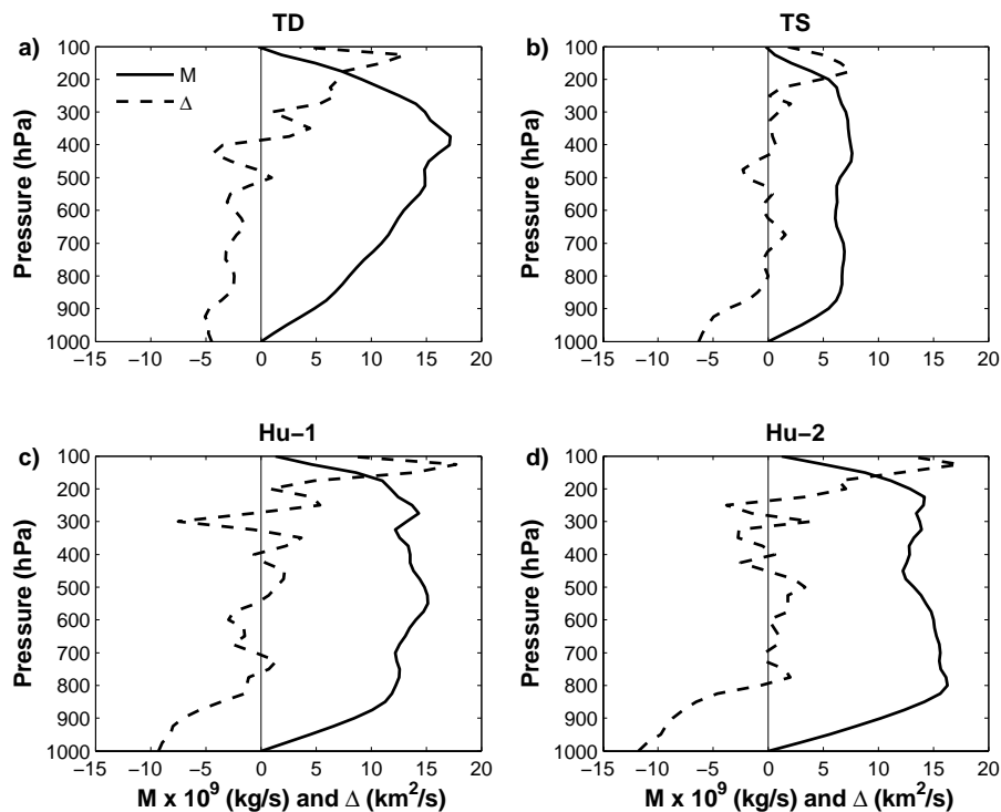
Fig. 8. Vertical profiles of horizontal ( \Delta , dashed line) and vertical ( M , solid line) mass fluxes for hurricane Dennis at (a) the tropical depression time (TD), (b) the tropical storm time (TS), (c) the first hurricane time (Hu-1) and (d) the second hurricane time (Hu-2) analyzed.
