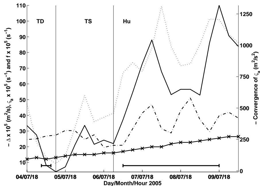
Fig. 5. Time evolution of minus the convergence of absolute vorticity (solid line), -\Delta (dotted line), and the absolute vorticity at the cyclone's boundary ( \zeta_a ) (dashed-dotted line) averaged over the 1000–900 hPa for hurricane Dennis. The line with crosses represents the Coriolis parameter at Dennis's central latitude. The absolute vorticity and Coriolis were multiplied by 4 for a better comparison with the other variables. Vertical solid lines delimit the tropical depression (TD), tropical storm (TS) and hurricane (Hu) stages. Periods when Dennis made landfalling are indicated by horizontal bars.
