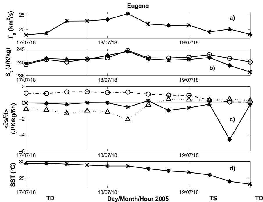
Fig. 12. Same as Fig. 11 but for tropical storm Eugene. Vertical solid lines delimit the tropical depression (TD) and tropical storm (TS) stages.
