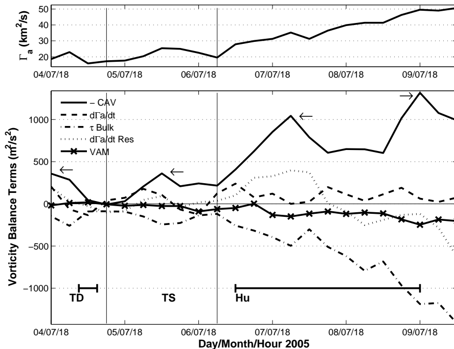
Fig. 3. Hurricane Dennis. (a) Time evolution of the absolute circulation averaged in the layer 1000–900 hPa. (b) Terms in the balance of Eq. (6) averaged in the layer 1000–900 hPa. The solid line represents minus the convergence of absolute vorticity ( -CAV ), line with crosses (vertical advection of momentum, VAM), dashed line ( \Gamma_a tendency), dashed-dotted line (bulk friction term, \tau Bulk) and dotted line (residual \Gamma_a tendency). Vertical solid lines delimit the tropical depression (TD), tropical storm (TS) and hurricane (Hu) stages as determined by the NHC. Periods when Dennis made landfall are indicated by horizontal bars. Arrows indicate certain times that will be discussed in the text and in Figs. 7 and 8.
