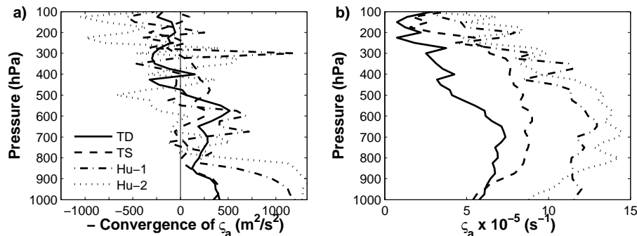
Fig. 7. Vertical profiles of (a) minus the convergence of absolute vorticity and (b) absolute vorticity at the cyclone's boundary averaged over the 4^\circ \times 4^\circ area at four times during hurricane Dennis' life cycle. Tropical depression time (TD, solid line), tropical storm time (TS, dashed line), first hurricane time (Hu-1, dashed-dotted line) and second hurricane time (Hu-2, dotted line).
