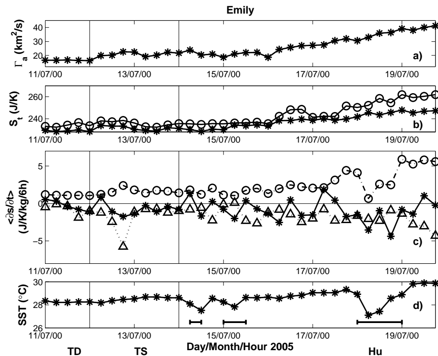
Fig. 15. Same as Fig. 11 but for hurricane Emily. Periods when Emily made landfalling are indicated by horizontal bars.
