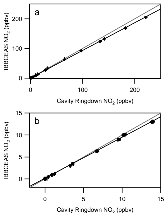
Fig. 4. (a) Correlation plot comparing NO 2 measurements from 0.45–222 ppbv acquired by the IBBCEAS instrument and the 532 nm CRDS. Measurements are averaged over similar 1-min time intervals. The slope is 0.932 \pm 0.001 (black line). The one-to-one line is shown in grey. (b) Expanded view of the 0–15 ppbv NO 2 data shown in (a). The 1\sigma standard deviation for 1-min IBBCEAS measurements with 1.13 ppbv NO 2 is 20 pptv.
