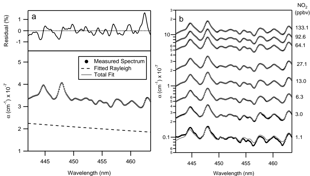
Fig. 3. (a) Example of \alpha_{\text{abs}} calculated for a single measured \text{NO}_2 spectrum (solid black points). The contribution from Rayleigh scattering (dashed line) and the total fit (grey line) are shown. The residual indicates the fitting error. The retrieved \text{NO}_2 concentration is 13.0 ppbv. (b) Examples of \alpha_{\text{abs}} calculated for a series spectra with different \text{NO}_2 concentrations (solid black points) and the corresponding spectral fits (grey lines). The fitted Rayleigh scattering has been subtracted to better display the \text{NO}_2 spectral fits.
