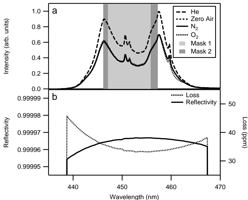
Fig. 2. (a) Representative spectra acquired with the IBBCEAS for He, N 2 , O 2 , and zero air. The difference between these spectra is due to Rayleigh scattering. The broad envelope is shaped by the transmission functions of the 450-nm bandpass filter and cavity mirrors. Narrow peaks near 450 and 452 nm are due to Xe emission lines superimposed on the broad continuum output of the lamp. Mask 1 indicates the spectral region used for retrievals. Mask 2 indicates the spectral region used for calculation of the reflectivity. (b) Reflectivity calculated according to Eq. (1) for the He and zero air spectra shown in (a). The peak reflectivity at 455 nm is 99.9966% (34 ppm total loss), corresponding to an effective pathlength of 29.4 km.
