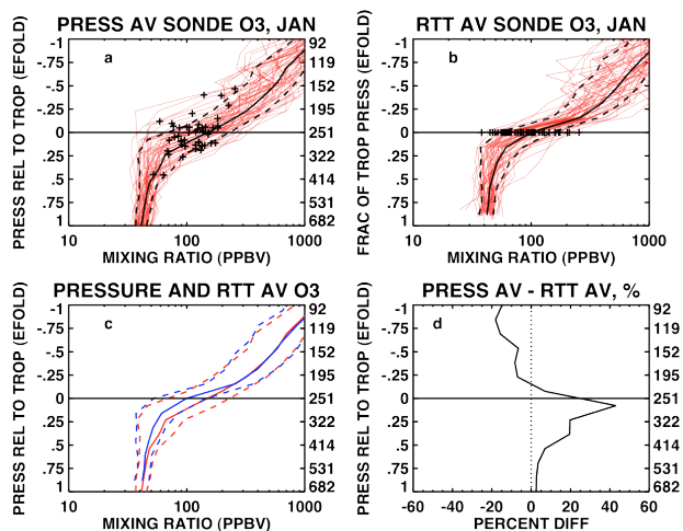
Fig. 9. (a) Daily ozonesonde profiles at Edmonton (red lines), plotted as function of pressure, for Januarys between 1985 and 2000. Left axis shows fraction of pressure efold from monthly median tropopause pressure. (The vertical axis is marked by the exponent y , where y varies over the range (-1,1) , and the pressure is given by P_{\text{trop}}e^y ). Right axis indicates pressure in hPa. Black crosses indicate thermal tropopause pressures for each profile. Black solid line is monthly mean ozone profile averaged as function of pressure. Black dashed lines indicate \pm one standard deviation. (b) Red lines show ozonesonde profiles at Edmonton in January, plotted as fraction of efold of each profile's tropopause pressure. (The vertical axis is marked by the exponent y , which varies over the range e^1 to e^{-1} .) Black crosses indicating the tropopause now all lie at y=0 . Black solid profile shows monthly average at constant fraction of tropopause pressure. Black dashed lines indicate \pm one standard deviation. (c) Comparison of monthly averaged profiles using pressure averaging (red lines) and relative-to-tropopause averaging (blue lines). Vertical axis is pressure. The relative-to-tropopause profile is plotted relative to the monthly median tropopause height. (d) Percent difference of pressure-averaged from RTT-averaged profiles.
