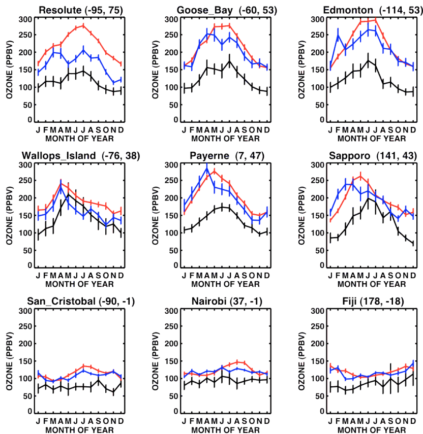
Fig. 6. Same as Fig. 5, except for 2^\circ \times 2.5^\circ run.
