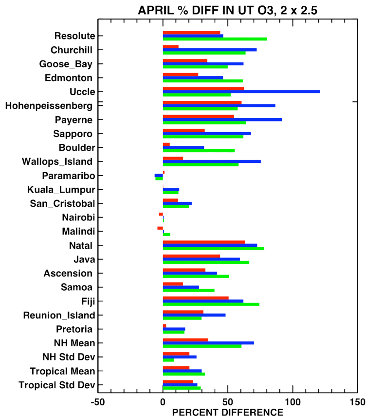
Fig. 13. Percent differences between modeled and observed ozone in the upper troposphere at observation locations, for the 2^\circ \times 2.5^\circ run. Red bar: Percent difference between observed and modeled pressure-averaged monthly mean ozone at a pressure that is one quarter of an efold higher than the observed monthly median tropopause pressure.
