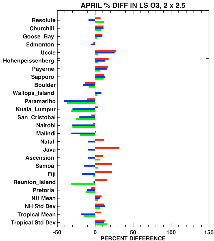
Fig. 14. Same as Fig. 13, except in the lower stratosphere at a pressure one quarter of an e-fold lower than the observed monthly median tropopause pressure.
