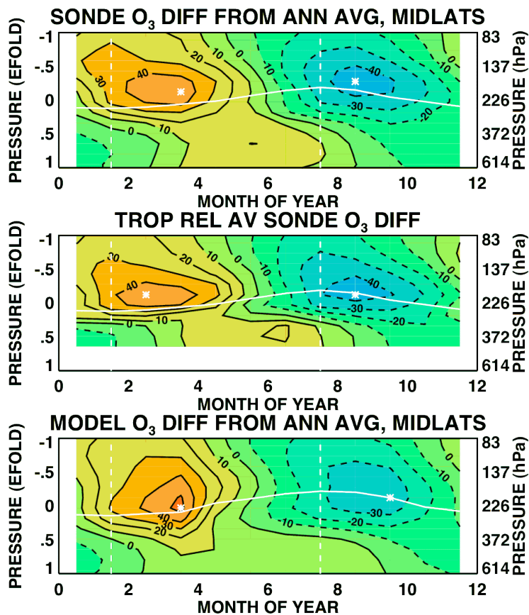
Fig. 17. Same as Fig. 15, except for midlatitude ozone stations.
