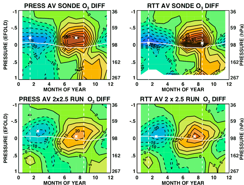
Fig. 15. Observed and modeled annual cycle of tropical ozone, expressed as percent deviation from annual mean ozone as function of pressure and time of year. Top left panel: Annual cycle for observed pressure-averaged ozone profiles. Top right panel: annual cycle for observed RTT-averaged ozone profiles. Bottom left panel: annual cycle for model pressure-averaged ozone profiles from the 2^\circ \times 2.5^\circ run. Bottom right panel: annual cycle for model RTT-averaged ozone profiles from the 2^\circ \times 2.5^\circ run. White solid line in each panel indicates thermal tropopause pressure. Vertical dashed lines mark position of minimum and maximum tropopause pressure. Asterisks mark location of maximum and minimum values of annual cycle in ozone.
