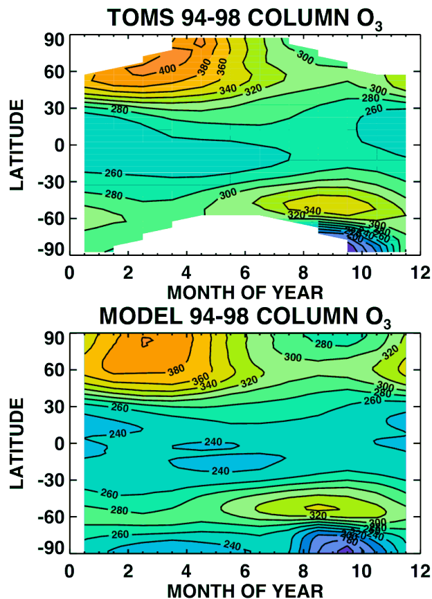
Fig. 2. Top panel: 1994–1998 average zonal mean total ozone from the Total Ozone Mapping Spectrometer merged ozone dataset, as function of time of year and latitude. Bottom panel: 1994–1998 average zonal mean total ozone from the GMI combined model, as function of time of year and latitude.
