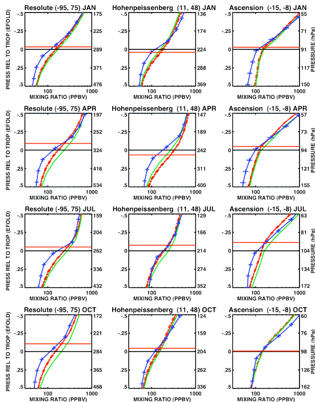
Fig. 11. Modeled and observed monthly average ozone profiles from the 2^{\circ} \times 2.5^{\circ} run at the stations of Resolute, Hohenpeissenberg, and Ascension for the months of January, April, July, and October. Blue line: observed RTT-averaged profile. Red line: Modeled RTT-averaged profile. Green line: Modeled RTT-averaged profile, plotted relative to the observed monthly median tropopause pressure, rather than relative to the model monthly median tropopause pressure. Black and red horizontal lines indicate observed and model monthly median tropopause pressures, respectively.
