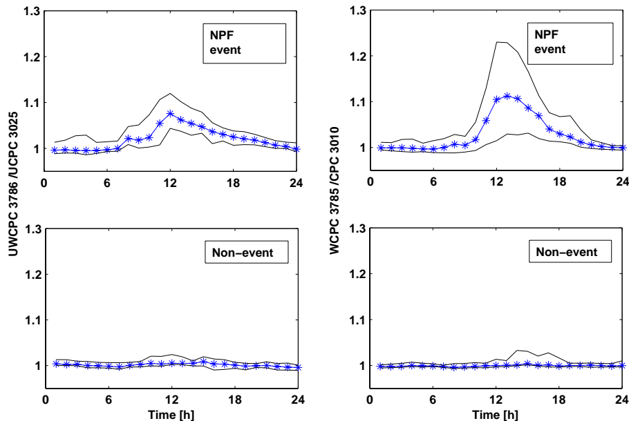
Fig. 5. The median (blue) diurnal behavior of the UWPC/UCPC (left) and WCPC/CPC (right) ratios on NPF event (top) and non-event (bottom) days during the measurement period in spring 2006. The black lines refer to the 25- and 75-percentiles.
