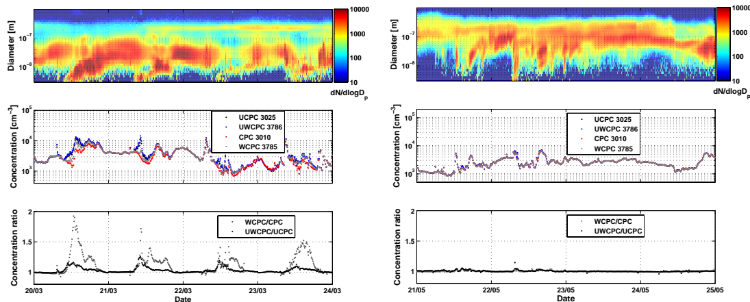
Fig. 4. Particle concentrations (middle) and water- to butanol-CPC concentration ratios (bottom) measured by the CPCB on (a) the period 20–23 March 2006 of four consecutive NPF event days; (b) the period 21–24 May 2006 of four consecutive days with no clear indications of NPF or growth. The corresponding particle size distributions measured with the DMPS are presented for comparison (top).
