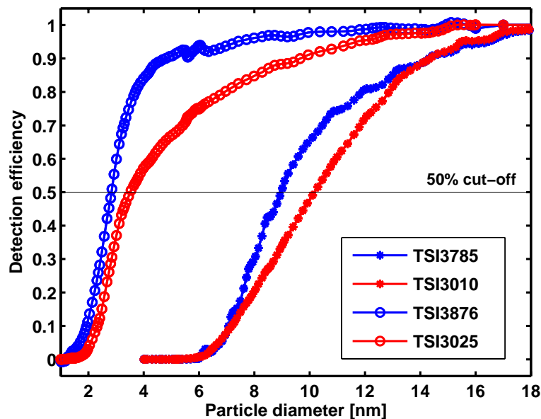
Fig. 3. The detection efficiencies of the individual CPCs in the CPCB, as measured for insoluble silver particles after the measurement campaign in Hyytiälä. Water-CPCs are indicated in blue and butanol-CPCs in red. The black line indicates the 50% detection efficiency limit (corresponding to the cut-off sizes D_{50} ).
