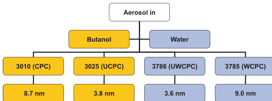
Fig. 1. A schematic figure of the setup of Condensation Particle Counter Battery (CPCB) used in this study. The CPCs using butanol as the working fluid are presented on yellow background, whereas the water-CPCs are on the blue background. The cut-off sizes set before the field measurements with silver particles are indicated under each individual CPC.
