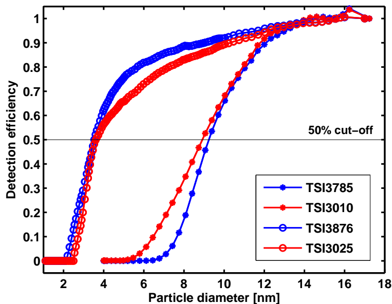
Fig. 2. The detection efficiencies of the individual CPCs in the CPCB, as measured for insoluble silver particles before the measurement campaign in Hyytiälä. Water-CPCs are indicated in blue and butanol-CPCs in red. The black line indicates the 50% detection efficiency limit (corresponding to the cut-off sizes D_{50} ).
