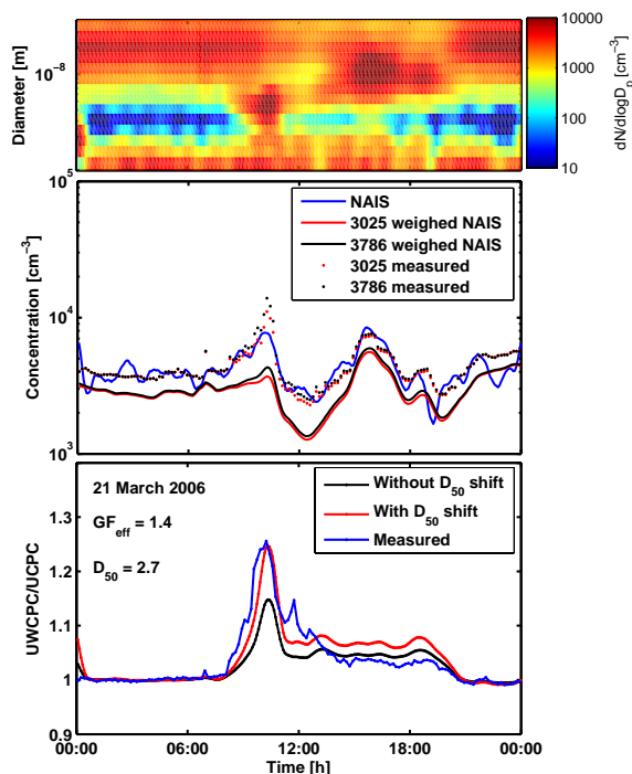
Fig. 7. Comparison between NAIS size distribution data and the concentrations measured by UWPCP and UCPC on a particle formation event day on 21 March 2006. Top: the size distributions measured by the NAIS. Middle: the total concentration measured by the NAIS (blue curve), the concentrations corresponding to the NAIS size distribution weighted with the detection efficiency curves of the UWPCP (black curve) and UCPC (red curve) for insoluble particles, and the total concentrations measured by the UWPCP (black dots) and UCPC (red dots). Bottom: the measured UWPCP to UCPC concentration ratio (blue) as predicted from the NAIS data assuming 1) the detection efficiency curves according to calibrations with insoluble particles (black); 2) the cut-off size of the UWPCP to be shifted to 2.7 nm (red).
