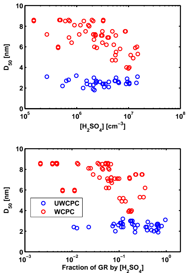
Fig. 10. The 50% cut-off sizes of the WPCP (red) and UWPCP (blue) as a function of modeled ambient sulfuric acid concentration (top) and the fraction of 3–7 (for WPCP) and 1.3–3 (for UWPCP) nm growth rates explained by sulfuric acid condensation (bottom).
