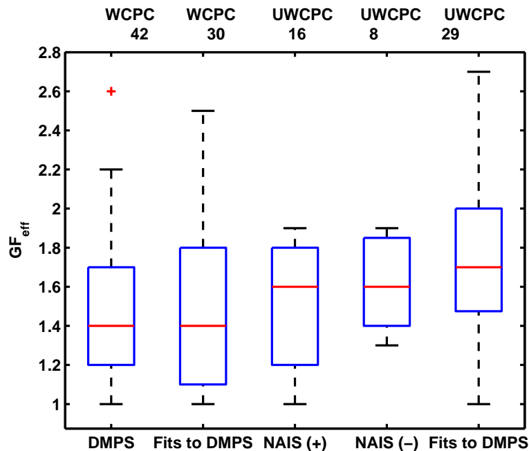
Fig. 9. The effective growth factors inside the WPCP and UWPCP during NPF events in spring 2006 according to different methods. The numbers above the figures refer to the number of particle formation event days included in the analysis. The red lines show the medians, the boxes indicate the 25- and 75-percentiles, and the error bars the 5- and 95-percentiles.
