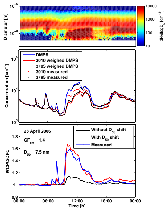
Fig. 6. Comparison between DMPS size distribution data and the concentrations measured by WCPC and CPC on a particle formation event day on 23 April 2006. Top: the size distributions measured by the DMPS. Middle: the total concentration measured by the DMPS (blue curve), the concentrations corresponding to the DMPS size distribution weighted with the detection efficiency curves of the WCPC (black curve) and CPC (red curve) for insoluble particles, and the total concentrations measured by the WCPC (black dots) and CPC (red dots). Bottom: the measured WCPC to CPC concentration ratio (blue) and as predicted from the DMPS data assuming 1) the detection efficiency curves according to calibrations with insoluble particles (black); 2) the cut-off size of the WCPC to be shifted to 7.5 nm (red).
