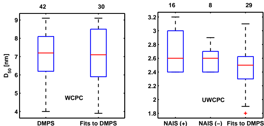
Fig. 8. The ambient 50% cut-off sizes of the WCPC (left) and UWPC (right) during NPF events in spring 2006, as obtained with different methods. The numbers above the figures refer to the number of particle formation event days included in the analysis. The red lines show the medians, the boxes indicate the 25- and 75-percentiles, and the error bars the 5- and 95-percentiles.
