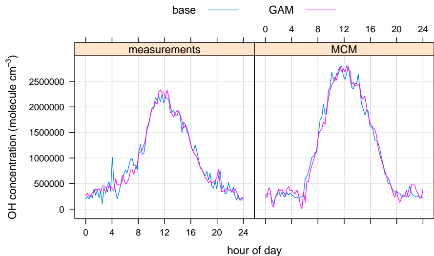
Fig. 5. Comparison of the measured (or modelled) OH concentration (shown as a blue line) against the predicted concentration (magenta line) produced using GAM_{ME} (or GAM_{MO} ) calibrating by bootstrapping the data.
