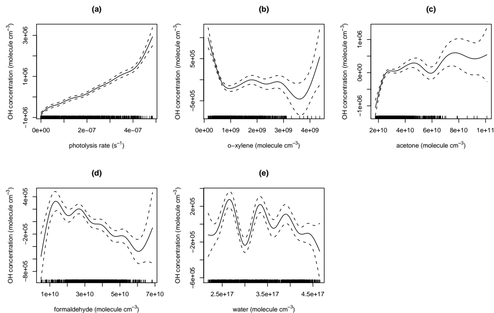
Fig. 3. Smooth functions of the predictor variables for measured OH (a) photolysis rate, (b) o-xylene, (c) acetone, (d) formaldehyde, (e) water. The concentrations of the predictor variables are shown along the x-axes and the value of the smooth function on the y-axis. The distribution of the data is indicated by the vertical marks along the x axis (rug plot). Confidence intervals at 95% are shown by dotted lines.
