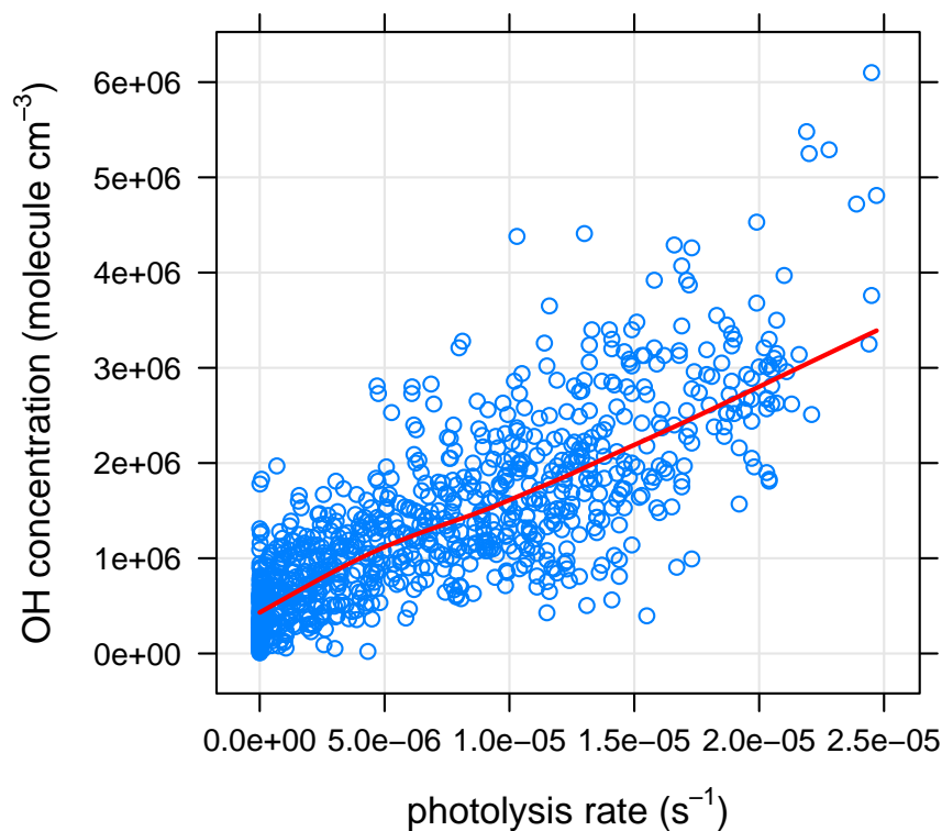
Fig. 2. Specimen smooth for OH concentration (molecule cm -3 ), the response variable, plotted against the photolysis rate of O 3 (to form O( 1 D)) (s -1 ), the predictor variable. The original data is shown with blue circles and the smooth as a red line.
