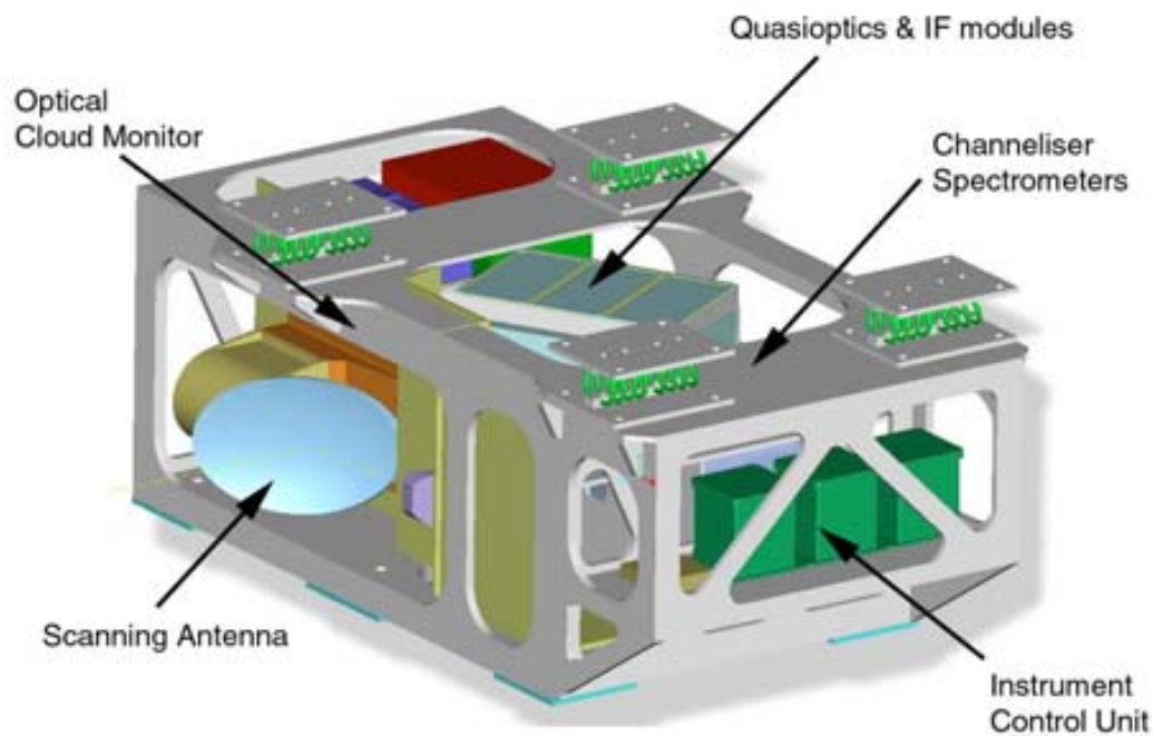
Fig. 1. MARSCHALS instrument configuration.
