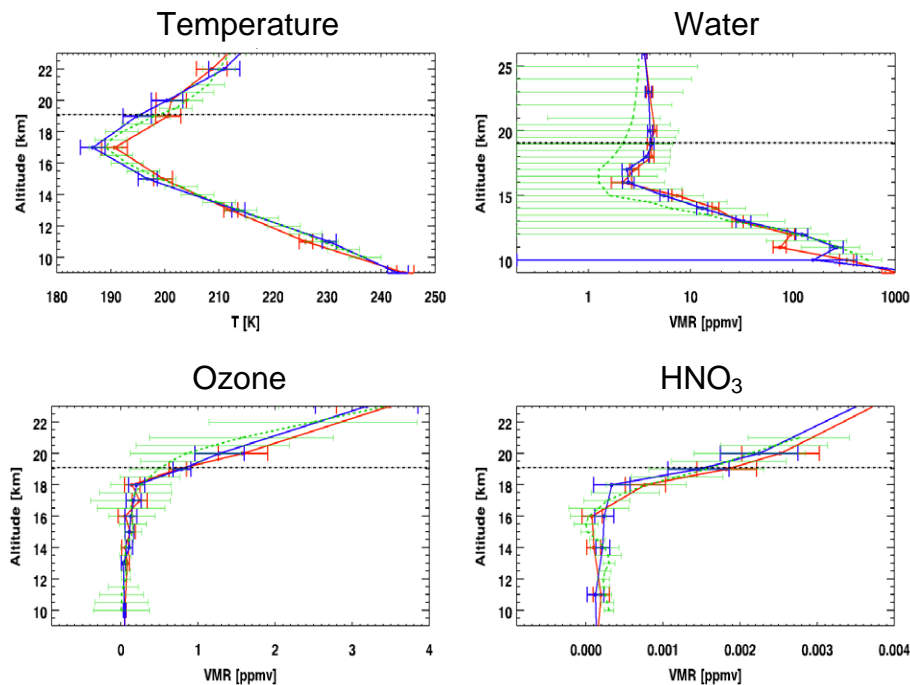
Fig. 17. Comparison of the results of MARSCHALS scans 36 (in red) and 39 (in blue) with MIPAS-STR (in green), together with the total error bars ( =3\sigma ).
