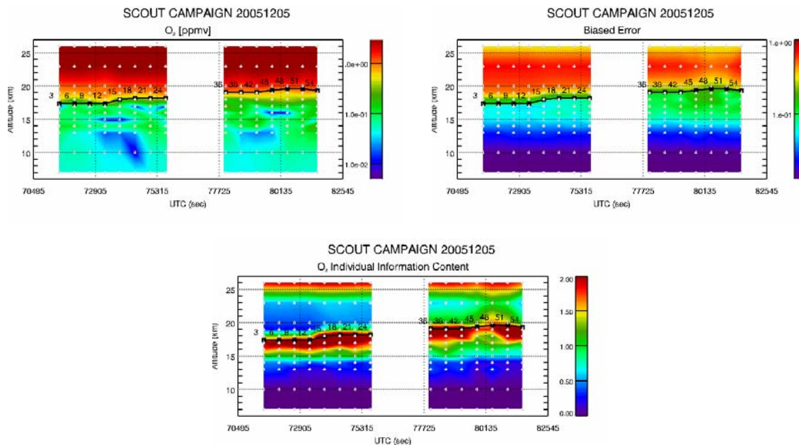
Fig. 12. Retrieved O 3 [ppmV] using the scans of band C (top-left panel), the related biased error [ppmV] (top-right panel) and the individual information content (bottom). The grey dots show the retrieval grid and the black line shows the aircraft altitude.
