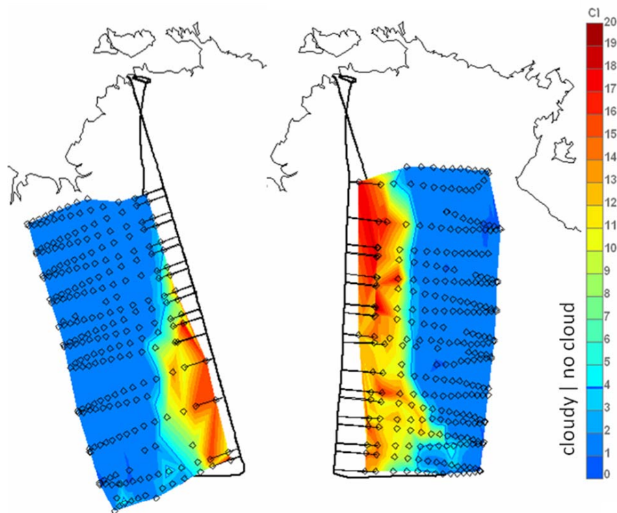
Fig. 4. Flight track of Geophysica on 5th December 2005 and the location of tangent points of the MIPAS-STR instrument. The altitude of the tangent point ranges from 6 km (farthest from the flight track) to flight altitude in 1 km steps. The under-laying field is the distribution of the cloud index (quotient of the radiance at 830\text{ cm}^{-1} and at 791\text{ cm}^{-1} ) derived for each tangent point from the individual MIPAS-STR spectrum. A value of 4 was chosen to separate cloud from no cloud.
