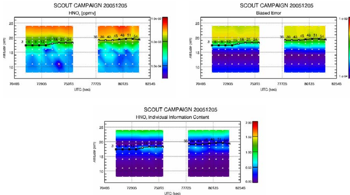
Fig. 13. Retrieved HNO 3 [ppmV] using the scans of band C (top-left panel), the related biased error [ppmV] (top-right panel) and the individual information content (bottom panel). The grey dots show the retrieval grid and the black line shows the aircraft altitude.
