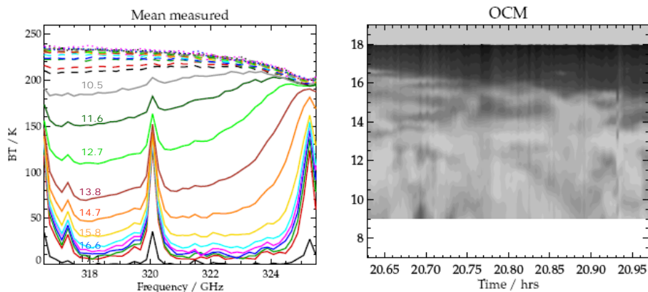
Fig. 5. Measured MARSCHALS Brightness Temperature spectra for Band C featuring \text{H}_2\text{O} at 325 GHz and \text{O}_3 at 320 GHz. All spectra are acquired during an 18 min period of level flight attitude and mean values around nominal view angles are calculated. The multi-coloured numbers in the left panel denote the respective tangent point altitudes of the measurements. The right panel shows the OCM (near-infrared) cloudiness during the same 18 min flight period. Note that spectral line features first become visible at around 10.5 km tangent point altitude. At this altitude and up to the Tropopause at around 17 km there are nevertheless significant amounts of visible clouds present in the field of view!
