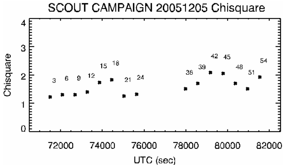
Fig. 7. Final \chi^2 -Test value for each scan reported as a function of the acquisition time (UTC).
