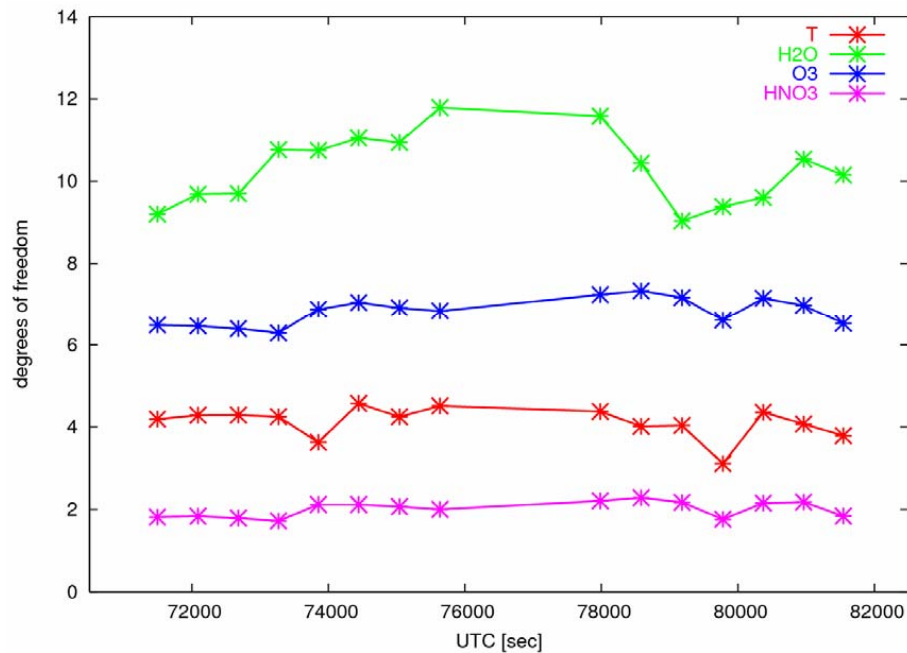
Fig. 9. Degrees of freedom for the different targets plotted as a function of the acquisition time (UTC).
