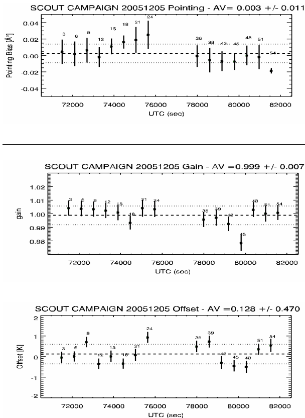
Fig. 15. Retrieved pointing bias (top panel), gain (central panel) and offset (bottom panel) using the scans of band C. The quantities are plotted versus the acquisition time (UTC). The dashed line represents their average value and the dotted lines represent the relative ESD.
