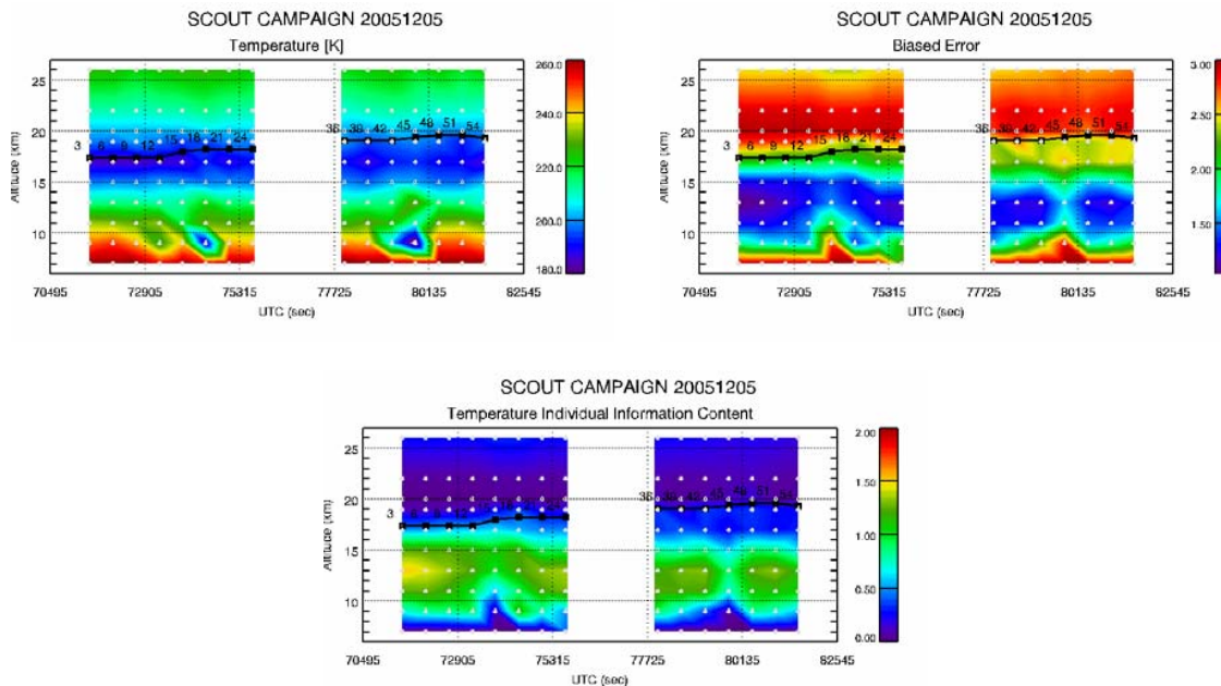
Fig. 10. Retrieved Temperature [K] using the scans of band C (top-left panel), the related biased error [K] (top-right) and the individual information content of the measurements (bottom). The grey dots show the retrieval grid and the black line shows the aircraft altitude.
