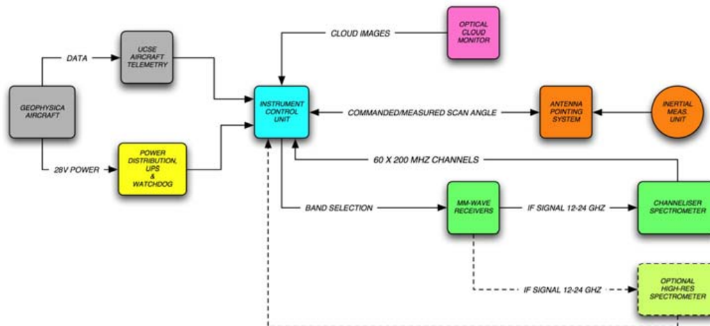
Fig. 2. Block diagram of MARSCHALS.
