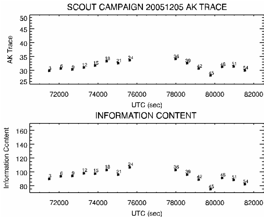
Fig. 8. A_{AKM} trace and Information content for the analysis of band C for each scan reported as a function of the acquisition time (UTC).
