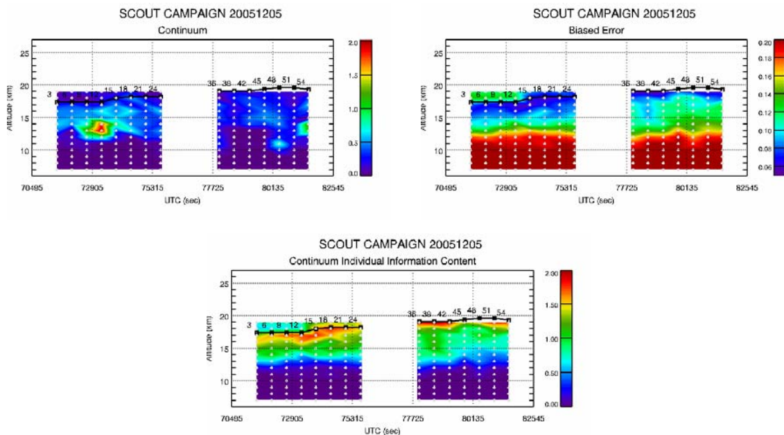
Fig. 14. Retrieved un-accounted continuum [ 10^{27} \text{ cm}^{-2} ] using the scans of band C (top-left panel), the related biased error [ 10^{27} \text{ cm}^{-2} ] (top-right panel) and the individual information content (bottom panel). The grey dots show the retrieval grid and the black line shows the aircraft altitude.
