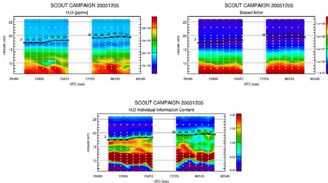
Fig. 11. Retrieved H 2 O [ppmV] using the scans of band C (top-left panel), the related biased error [ppmV] (top-right panel) and the individual information content (bottom panel). The grey dots show the retrieval grid and the black line shows the aircraft altitude.
