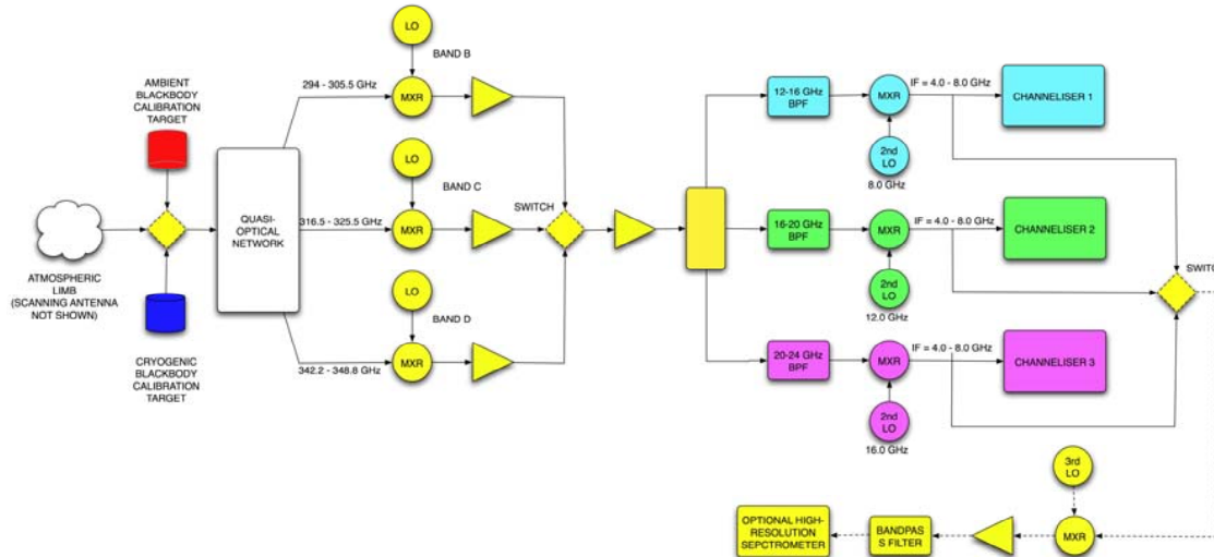
Fig. 3. Millimetre-wave receiver signal flow.
