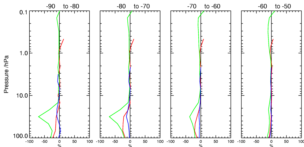
Fig. 7. Mean of (Analysis-MIPAS), normalised by climatology (in percent) over the intercomparison period, for ECMWF (Red), BASCOE (Green) and MIMOSA (Blue), concentrating on the southern high latitudes ( 50^{\circ} S to 90^{\circ} S in 10^{\circ} bands).
