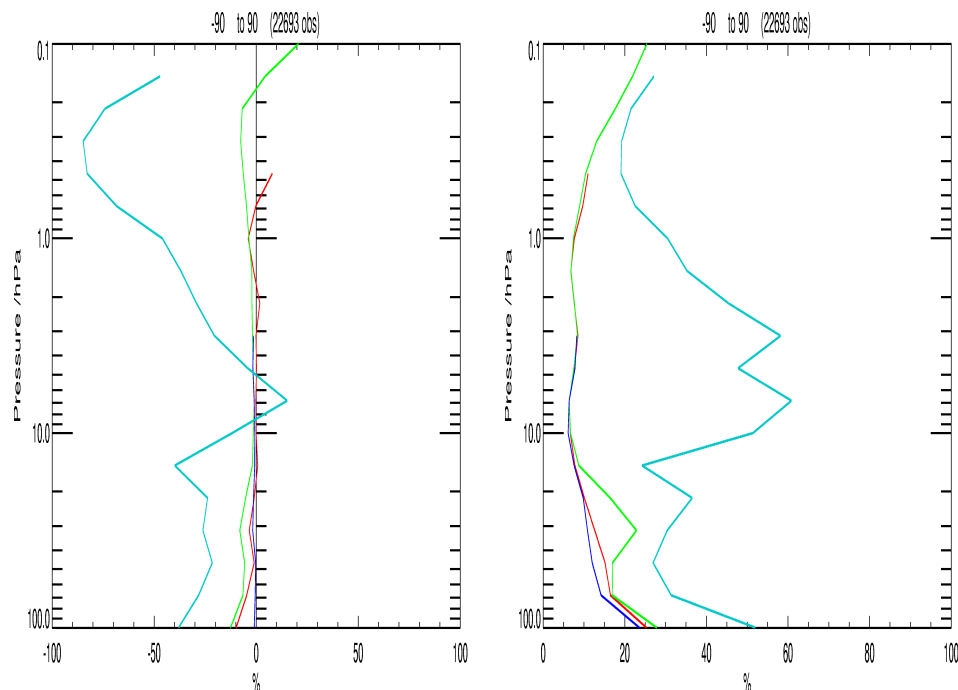
Fig. 12. Left: Mean of (Analysis – MIPAS) water vapour mixing ratio, normalised by climatology (in percent) over the intercomparison period, for ECMWF (Red), BASCOE (Green), MIMOSA (Blue) and Met Office (light Blue), for all latitudes. Right: As left but standard deviation rather than mean difference.
