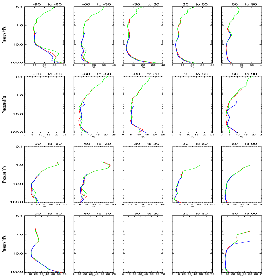
Fig. 6. Standard deviation of (Analysis-Observations) water vapour mixing ratio, normalised by climatology (in %) over the intercomparison period, for ECMWF (Red), BASCOE (Green) and MIMOSA (Blue), for the five different latitude bins. For rows 1 to 4, the observational data is MIPAS, HALOE, SAGE-II and POAM-III respectively. If there are not any satellite profiles available, the graphs are blank.
