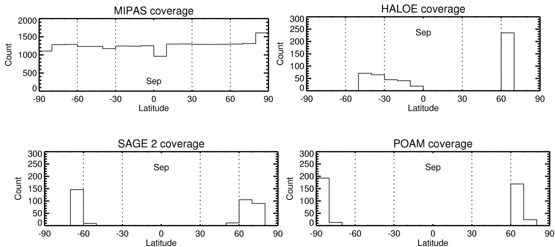
Fig. 1. Latitudinal coverage of MIPAS (top left), HALOE (top right), SAGE II (bottom left) and POAM III (bottom right) profiles over the intercomparison period (29 August–29 September 2003). Data are collected in 10° latitude bins.
