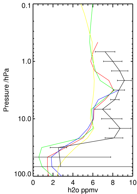
Fig. 10. A comparison of a POAM profile (black, with one standard deviation error bars – 21 September 2003, 12 p.m., 283° E, 88° S) with the different analyses and climatology (colours as Fig. 2).
