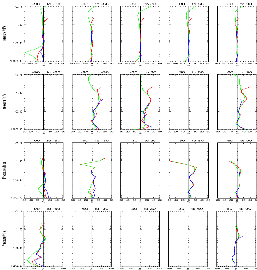
Fig. 5. Mean of (Analysis-Observations) water vapour mixing ratio, normalised by climatology (in %) over the intercomparison period, for ECMWF (Red), BASCOE (Green) and MIMOSA (Blue), for the five different latitude bins. For rows 1 to 4, the analyses are compared with MIPAS, HALOE, SAGE-II and POAM-III data respectively. If there are not any satellite profiles available, the graphs are blank.
