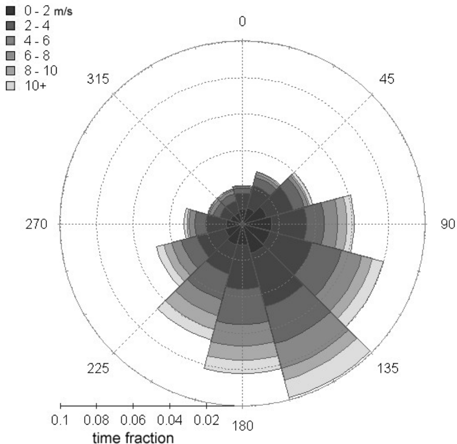
Fig. 2. Wind direction and speed during years 2003–2006. Data represents approximately 2/3 of each year, with data only available in the warmer months ( T > -35^{\circ}\text{C} ).
